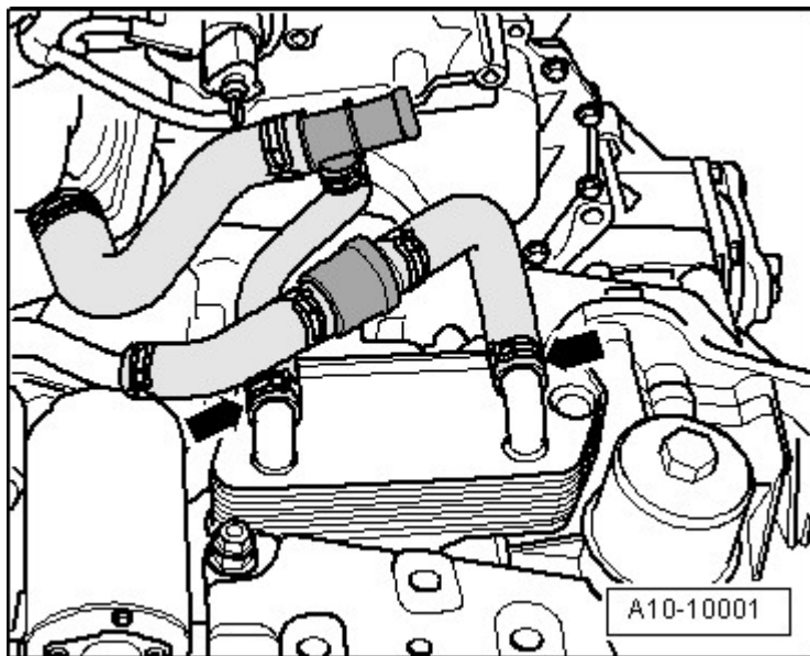
Fig. 95: Transmission Oil Cooler Coolant Hoses
