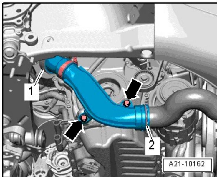
Fig. 48: Air Guide Pipe And Bolts
