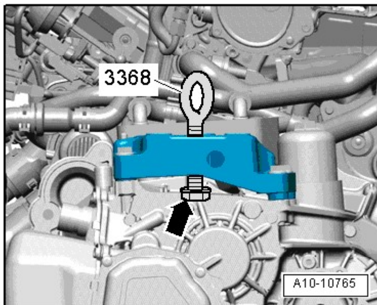
Fig. 97: Lifting Eyebolt 3368
