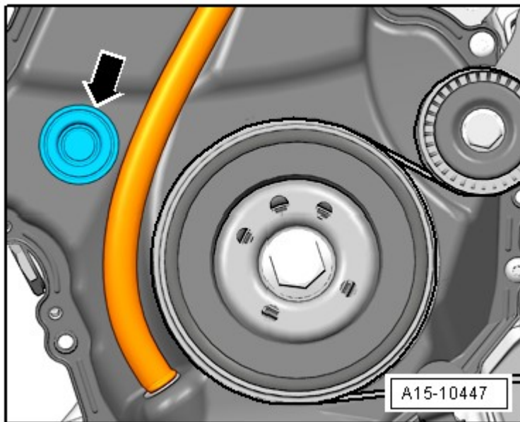
Fig. 146: Locating Plug
