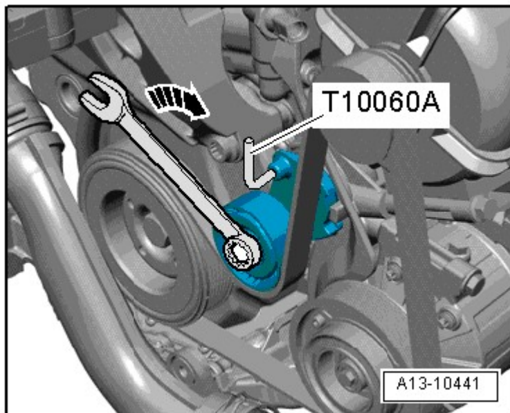
Fig. 44: Rotating Tensioner
