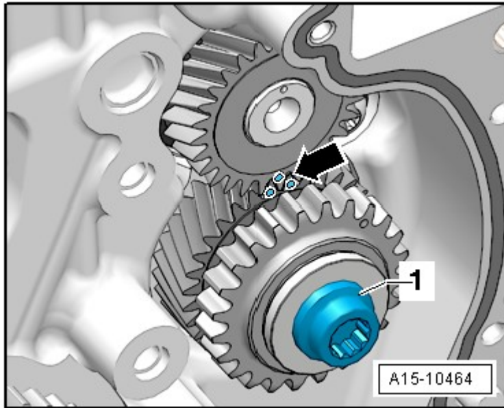
Fig. 75: Identifying Intermediate Shaft Sprocket
