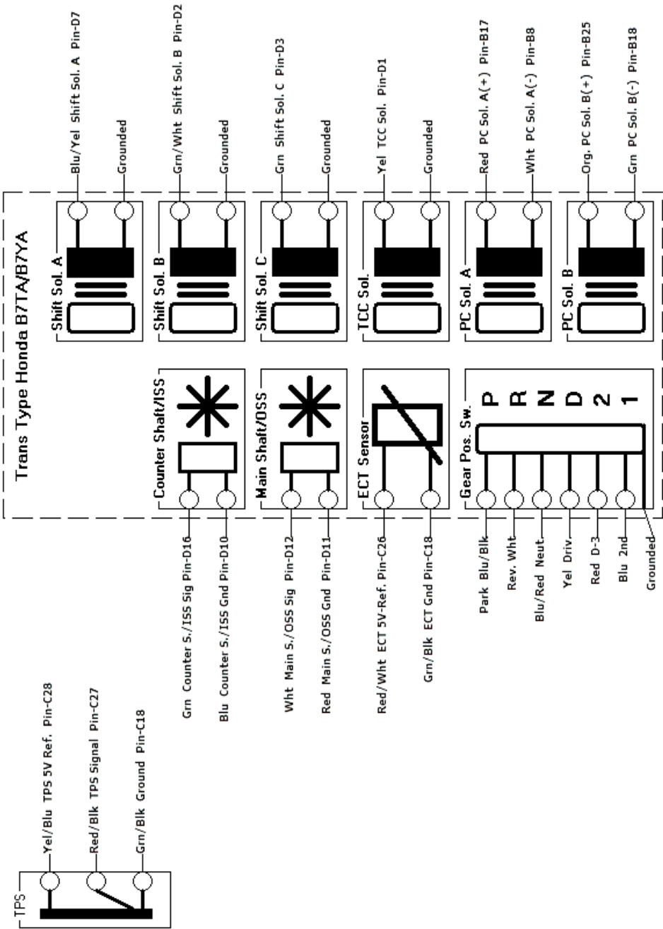
Honda B7TA/B7YA Transmission Wiring Diagram
