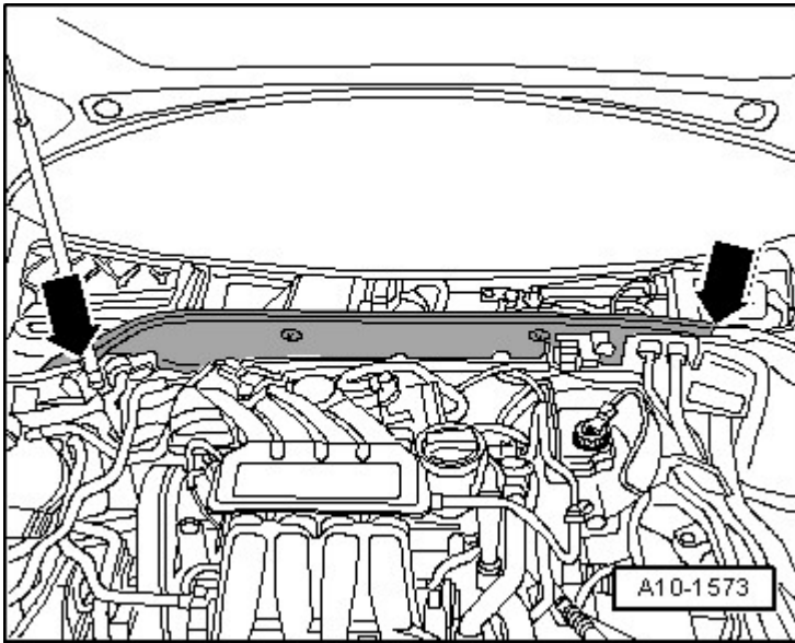
Fig. 55: Plenum Chamber Partition Courtesy of AUDI OF AMERICA, LLC
