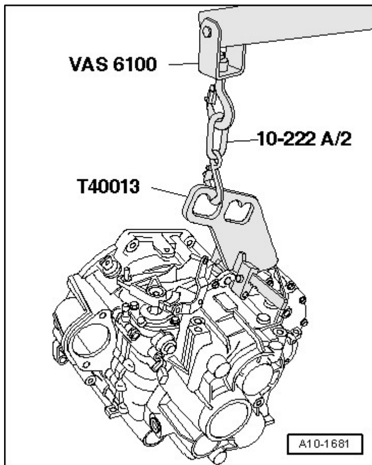
Fig. 92: Engaging Workshop Crane VAS 6100 With Additional Hooks 10-222 A/2 At Lifting Tackle Courtesy of AUDI OF AMERICA, LLC
