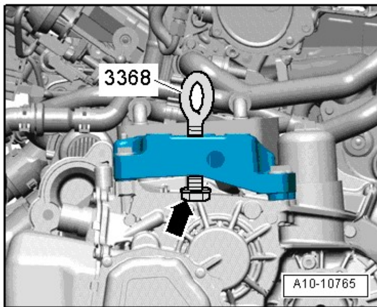
Fig. 97: Lifting Eyebolt 3368
