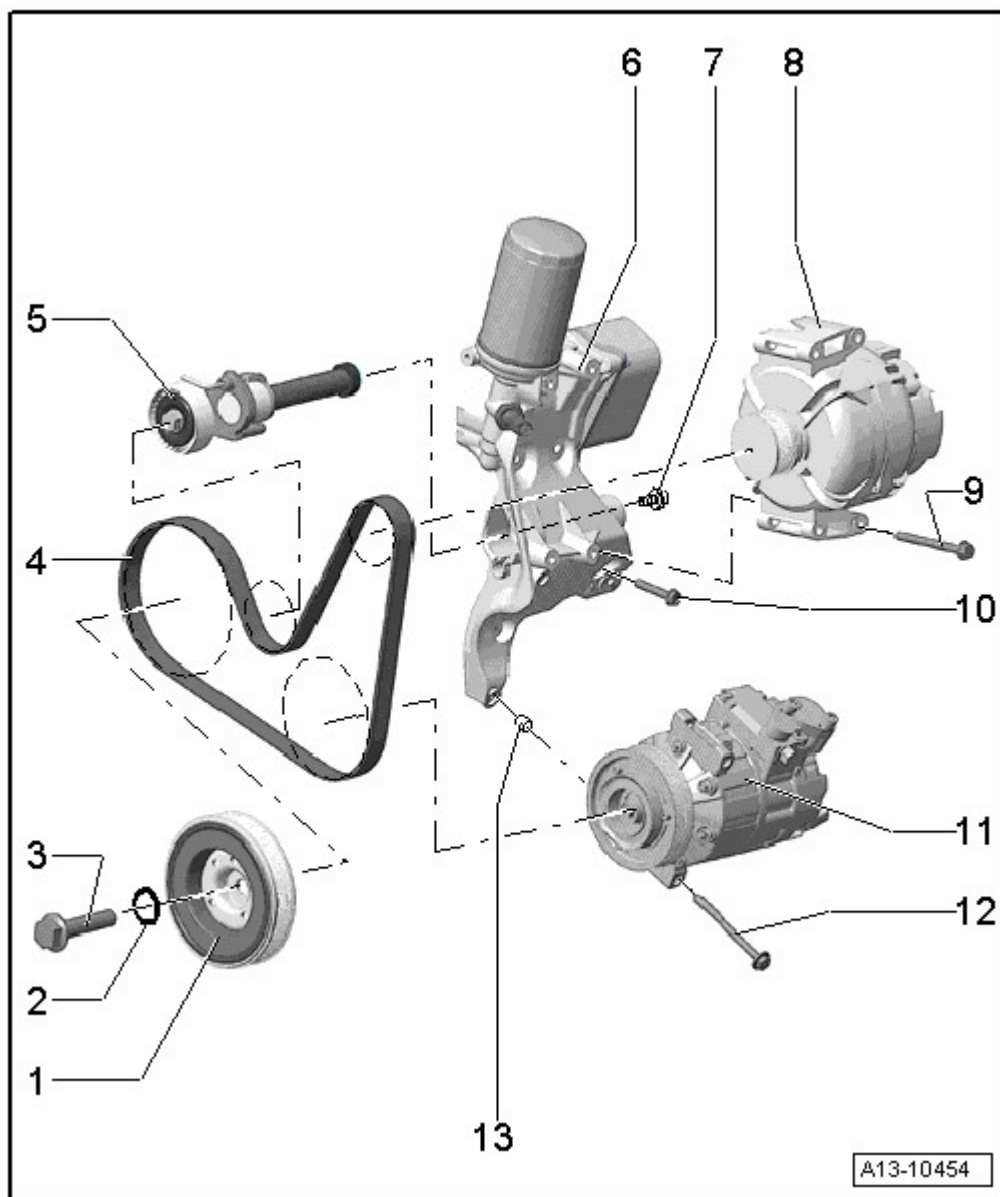
Fig. 4: Identifying Ribbed Belt Drive Assembly Overview
