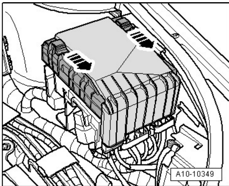
Fig. 58: Identifying E-Box Cover And Latches
