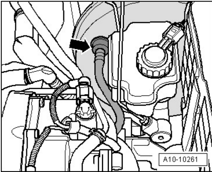
Fig. 50: Brake Booster Vacuum Hose
