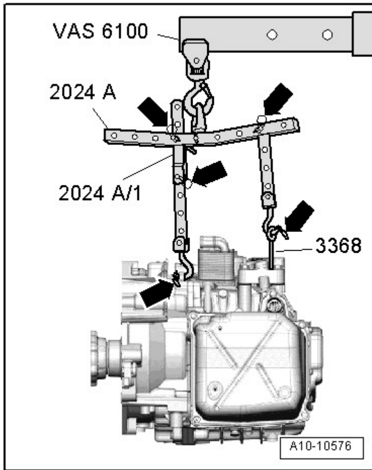
Fig. 98: Transmission Lifted
