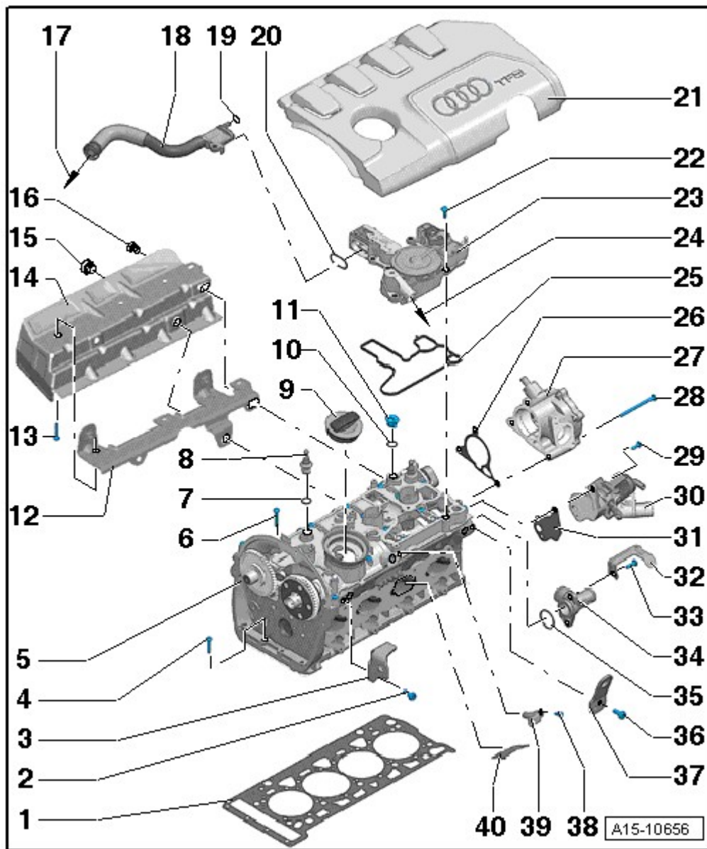
Fig. 10: Identifying Cylinder Head Assembly Overview
