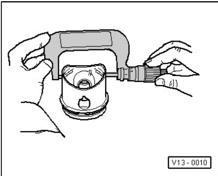
Fig. 25: Checking Piston
