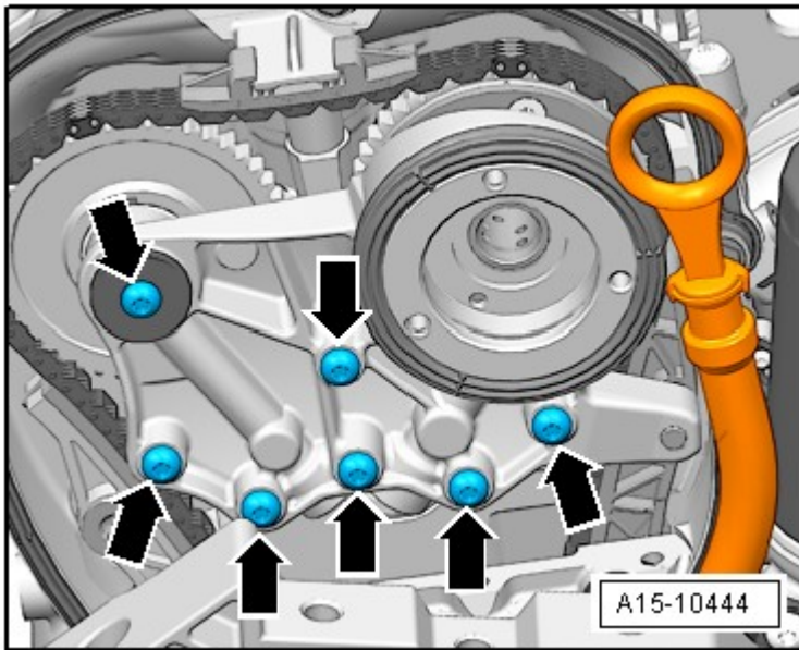
Fig. 132: Identifying Bearing Bracket Bolts
