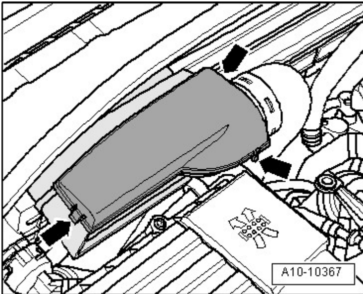
Fig. 26: Air Duct Cover Slide Clips
