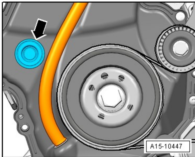
Fig. 146: Locating Plug
