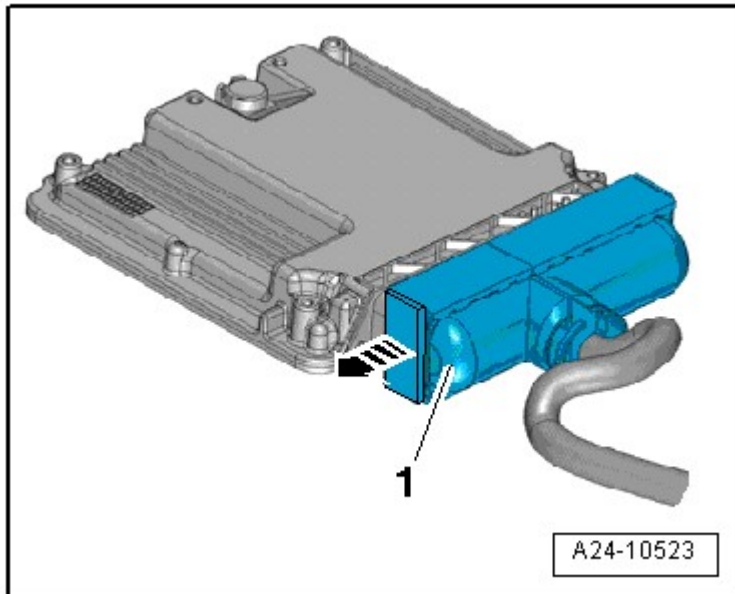
Fig. 56: Disconnecting Engine Wiring Harness Electrical Connector Courtesy of AUDI OF AMERICA, LLC
