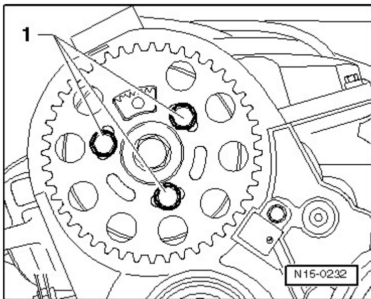
Fig. 104: Identifying Camshaft Pulley Securing Bolts Courtesy of AUDI OF AMERICA, LLC
