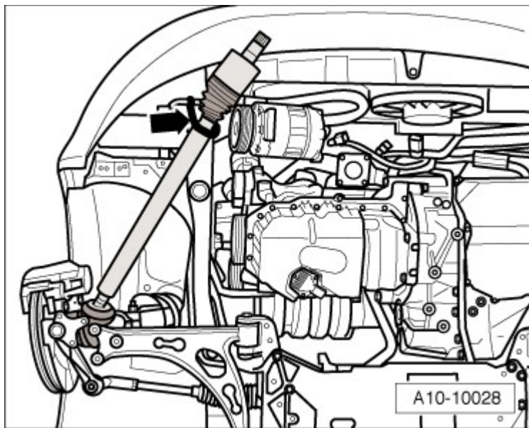
Fig. 93: Identifying Drive Axle Secured To Longitudinal Member
