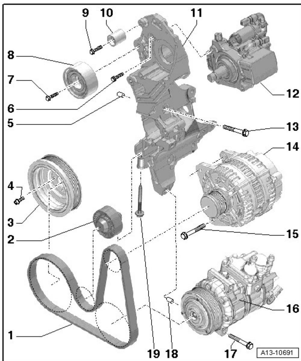
Fig. 3: Identifying Ribbed Belt With Tensioning Roller, Overview
