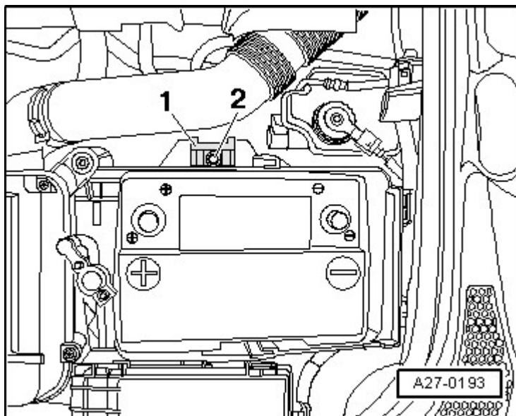
Fig. 42: Identifying Screws And Securing Bracket For Battery Courtesy of AUDI OF AMERICA, LLC
