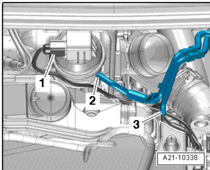
Fig. 45: Identifying Turbocharger Vacuum Diaphragm Courtesy of AUDI OF AMERICA, LLC
