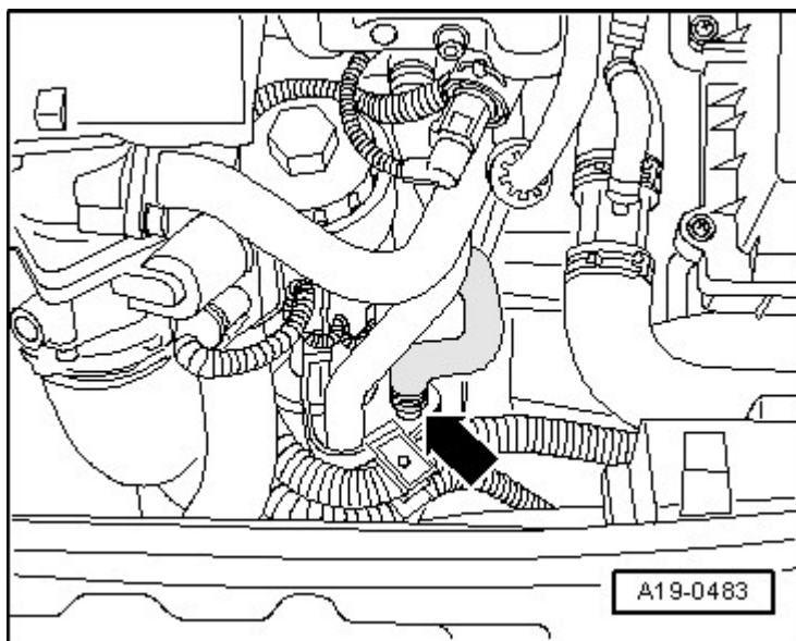
Fig. 41: Identifying Hose Clamp Courtesy of AUDI OF AMERICA, LLC
