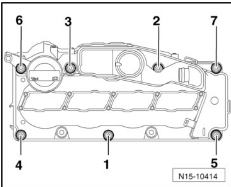
Fig. 58: Identifying Head Cover Bolts -1 Through 7- Tightening Sequence Courtesy of AUDI OF AMERICA, LLC
