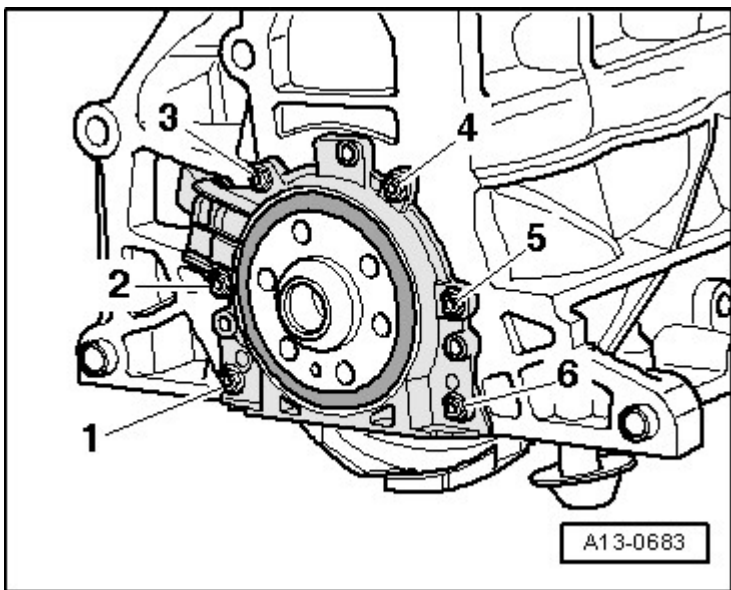
Fig. 97: Tightening Sequence
