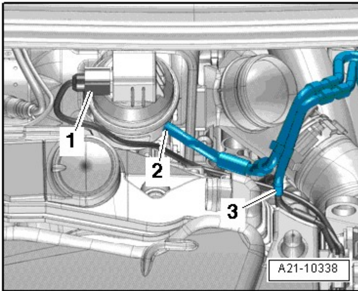
Fig. 71: Identifying Turbocharger Vacuum Diaphragm
