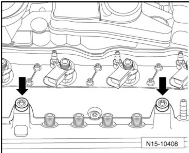
Fig. 57: Identifying Bolts -Arrows- And Fuel Rail Courtesy of AUDI OF AMERICA, LLC
