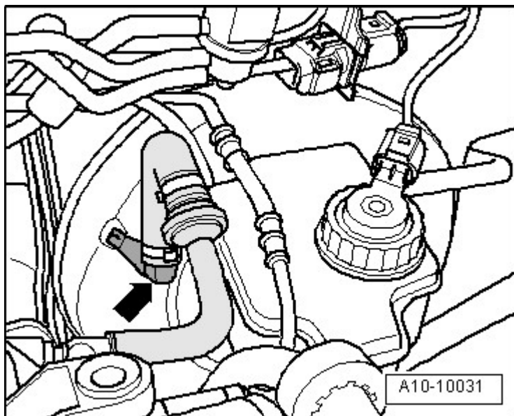
Fig. 46: Identifying Vacuum Hose Courtesy of AUDI OF AMERICA, LLC
