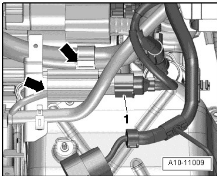
Fig. 77: Identifying Wiring Harnesses And Connector On Hot Side Charge Air Pipe Courtesy of AUDI OF AMERICA, LLC
