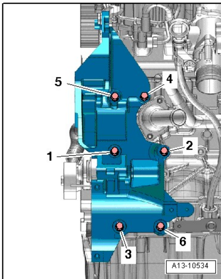
Fig. 22: Tightening Sequence
