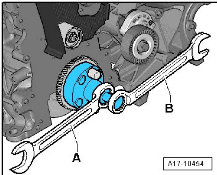
Fig. 103: View Of Counter-Holding Crankshaft
