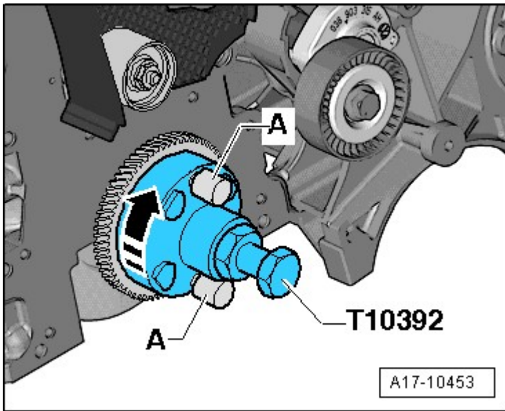
Fig. 102: Identifying Puller T10392
