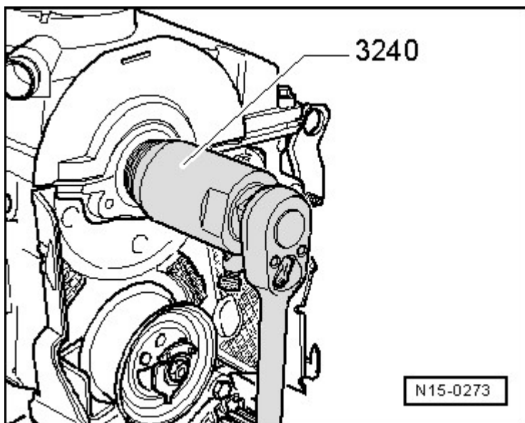
Fig. 100: Identifying Special Tool - 3240
