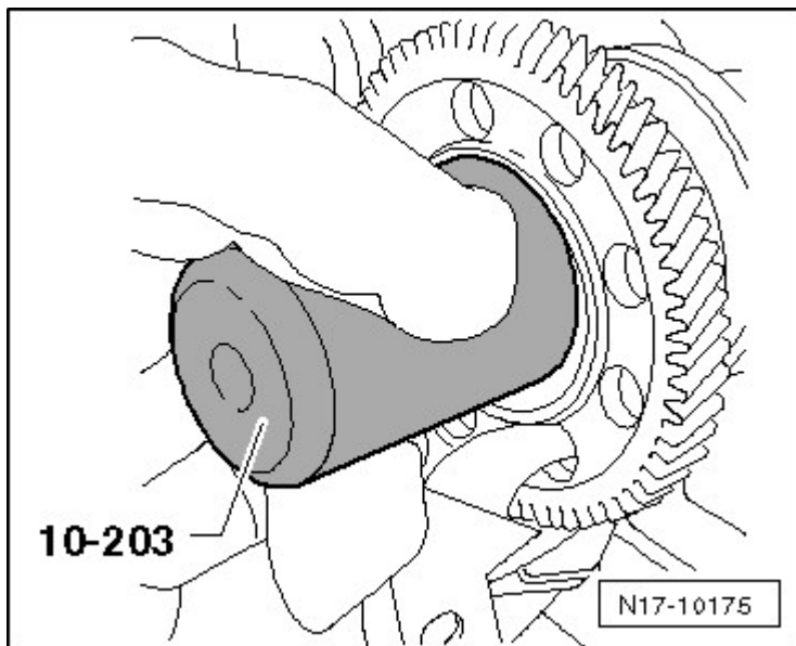
Fig. 106: View Of Oil Seal Driver 10-203
