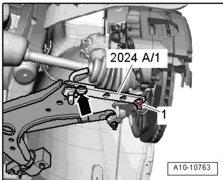
Fig. 94: Tilting Right Suspension Strut Outward And Supporting It With Extension 2024 A /1
