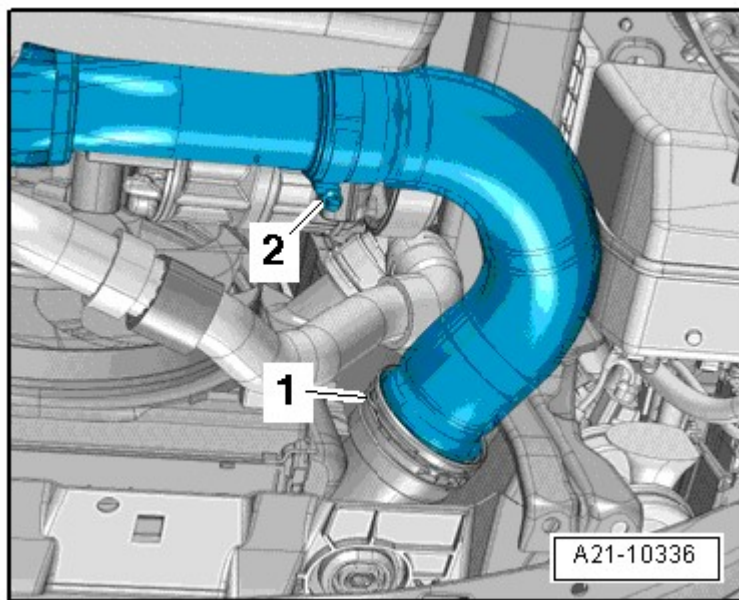
Fig. 64: Identifying Air Guide Hose And Clamps
