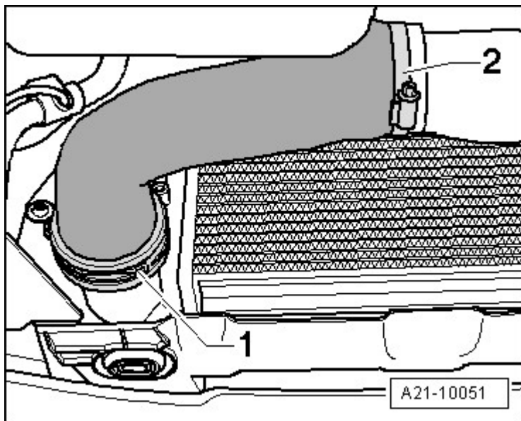
Fig. 63: Identifying Air Guide Hose And Clamps
