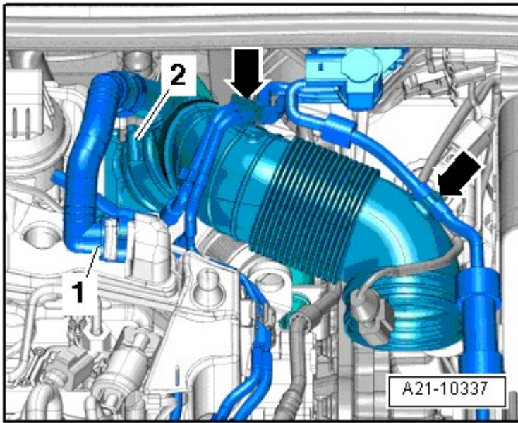
Fig. 70: Identifying Air Guide Pipe
