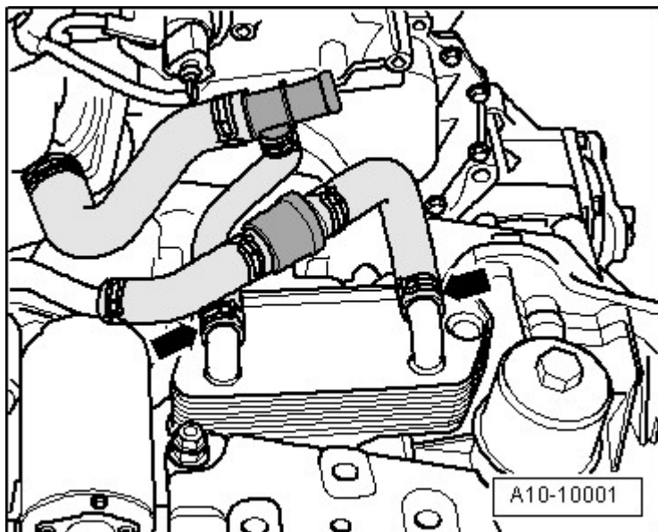
Fig. 76: Identifying Hose Clamps Courtesy of AUDI OF AMERICA, LLC
