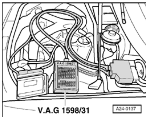
Fig. 322: Connecting Test Box VAG1598/31 To Engine Control Module Wiring Harness Courtesy of VOLKSWAGEN UNITED STATES, INC.
