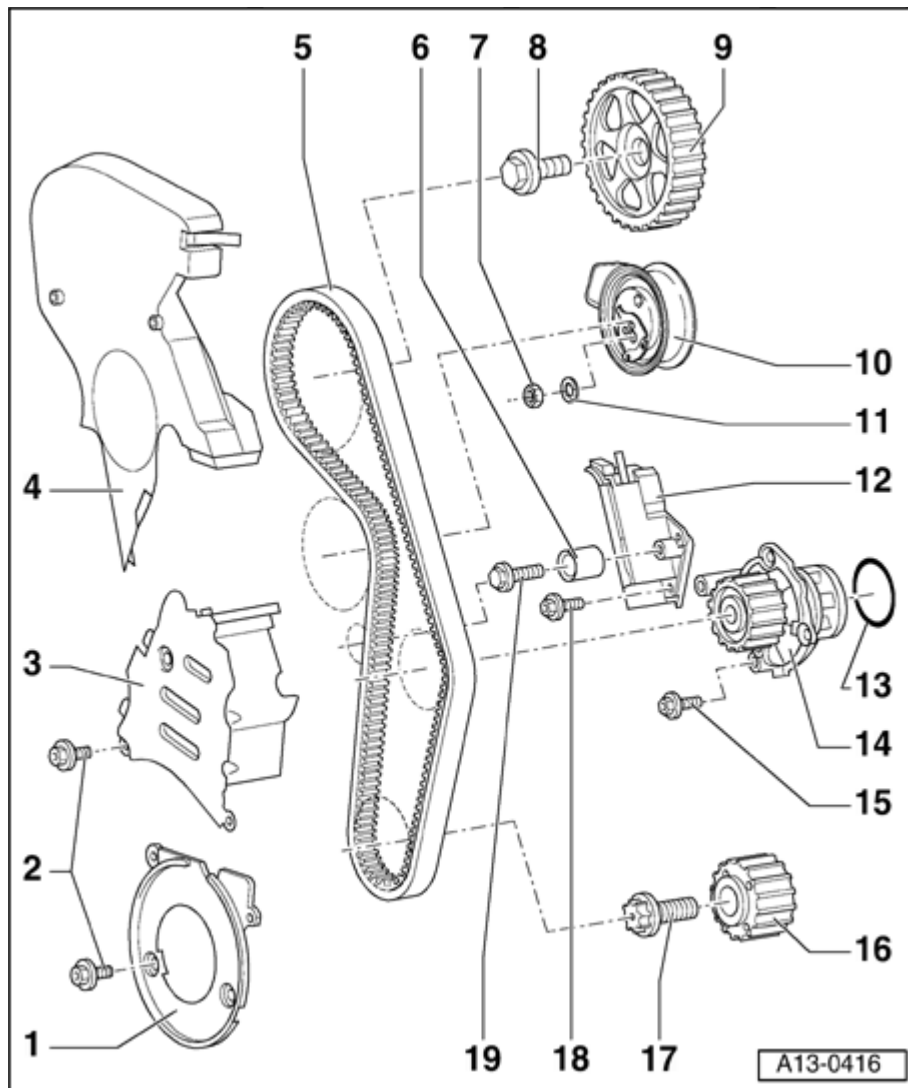
Fig. 79: Toothed Belt Drive, Overview
