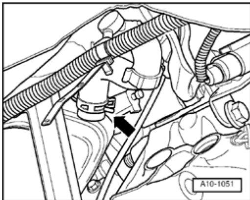
Fig. 271: Disconnecting Coolant Hose From Oil Cooler And Drain Off Remaining Coolant Courtesy of VOLKSWAGEN UNITED STATES, INC.
