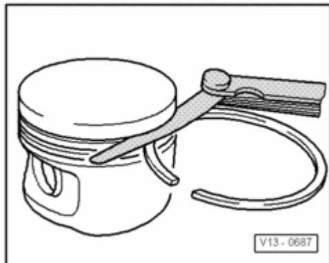
Fig. 139: Checking Ring To Groove Clearance
