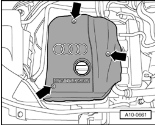
Fig. 409: Removing Engine Cover
