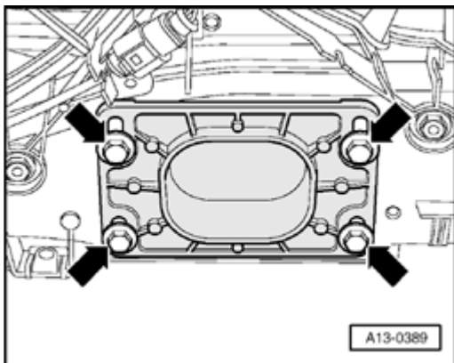
Fig. 64: Bolt Lock Carrier To Longitudinal Member And To Fenders Courtesy of VOLKSWAGEN UNITED STATES, INC.
