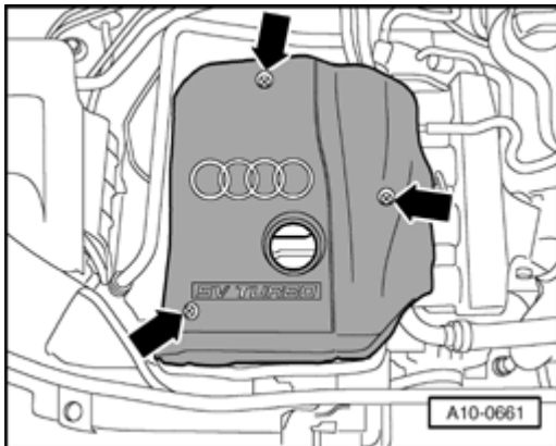
Fig. 413: Removing Engine Cover
