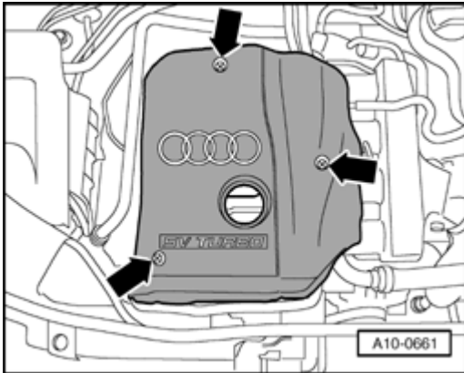
Fig. 7: Removing Engine Cover
