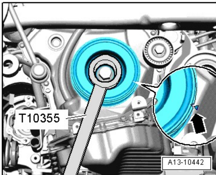
Fig. 480: Loosening Clamping Sleeve Courtesy of VOLKSWAGEN UNITED STATES, INC.
