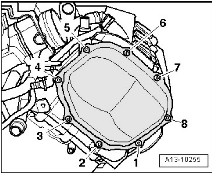
Fig. 49: Right Timing Chain Cover Bolt Tightening Sequence & Specification
