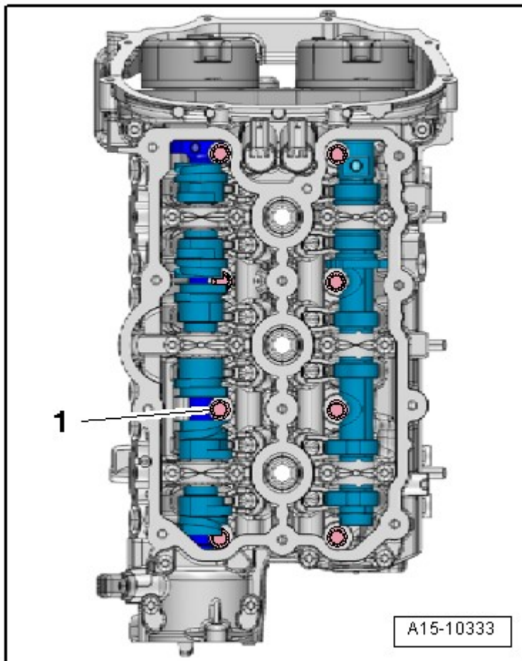
Fig. 153: Identifying Bolt (Left Cylinder Head)
