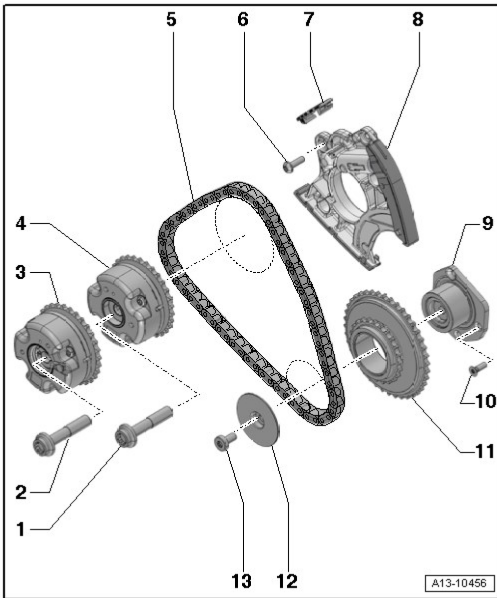
Fig. 5: Identifying Camshaft Timing Chains Assembly
