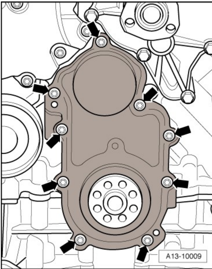
Fig. 16: Identifying Front Sealing Flange Bolts Courtesy of AUDI OF AMERICA, LLC
