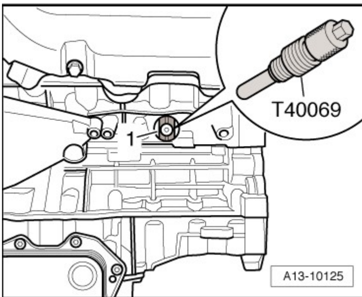
Fig. 93: Identifying Crankshaft Holder T40069 In Hole, Removal/Installation
