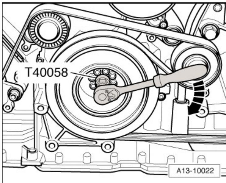
Fig. 71: Identifying TDC With Special Tool Adapter T40058
