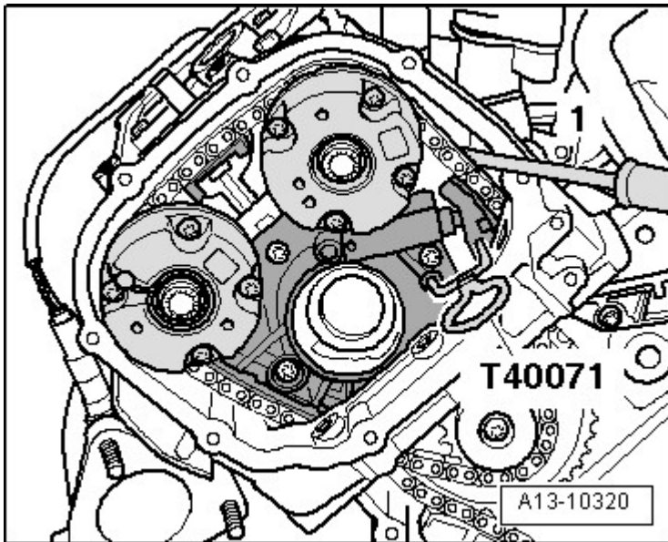
Fig. 78: Pressing Left Camshaft Timing Chain Tensioner Glide Track Inward With Screwdriver As Far As Stop And Securing Chain Tensioner With Locking Pin T40071
