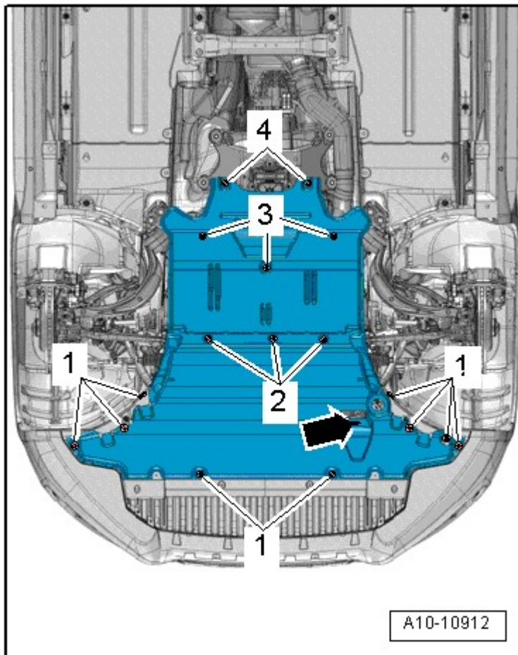
Fig. 68: Identifying Noise Insulation
