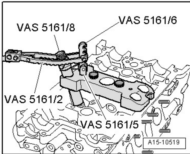
Fig. 213: Identifying Engaging Device VAS 5161/6, Installation Fork VAS 5161/5 And Guide Plate, Removal/Installation Courtesy of AUDI OF AMERICA, LLC
