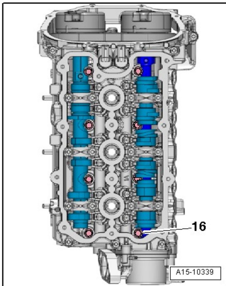
Fig. 28: Identifying Bolt -16-
