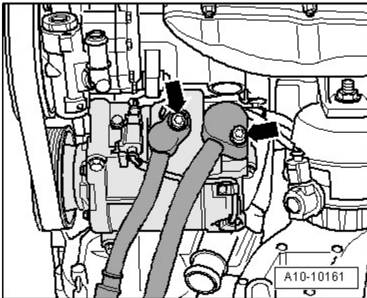
Fig. 26: Identifying Bolts
