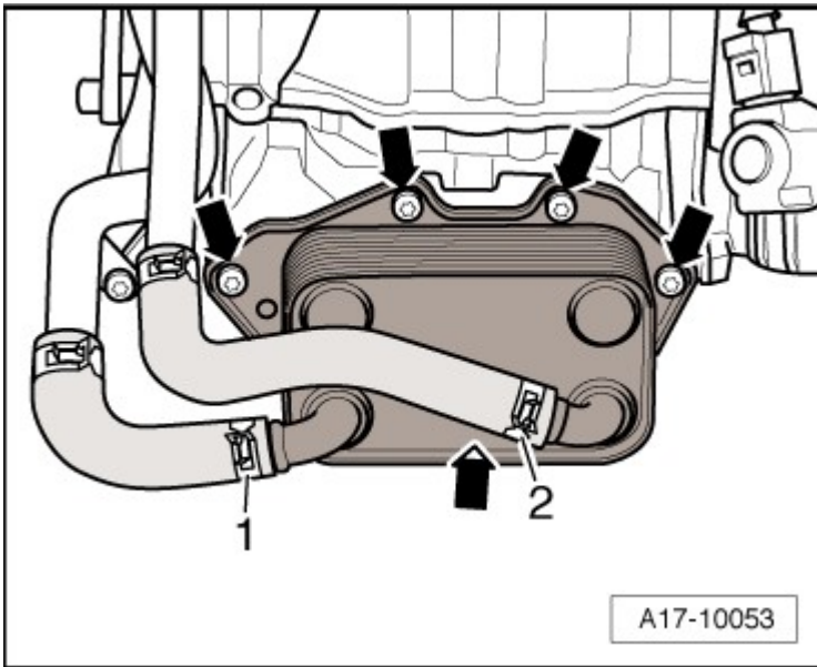
Fig. 191: Connecting/Disconnecting Coolant Hoses With Hose Clamps
