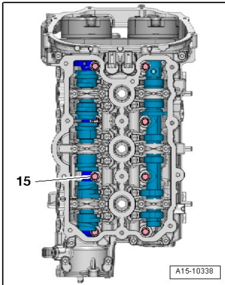
Fig. 174: Identifying Bolt
