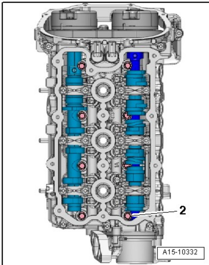
Fig. 154: Identifying Bolt (Right Cylinder Head)
