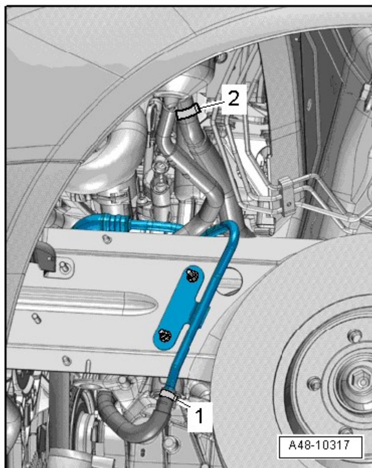
Fig. 9: Disconnecting Power Steering Hydraulic Oil Supply Line
