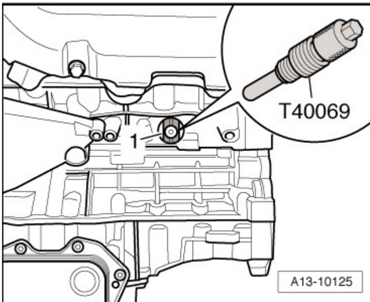
Fig. 97: Identifying Crankshaft Holder T40069 In Hole, Removal/Installation Courtesy of AUDI OF AMERICA, LLC
