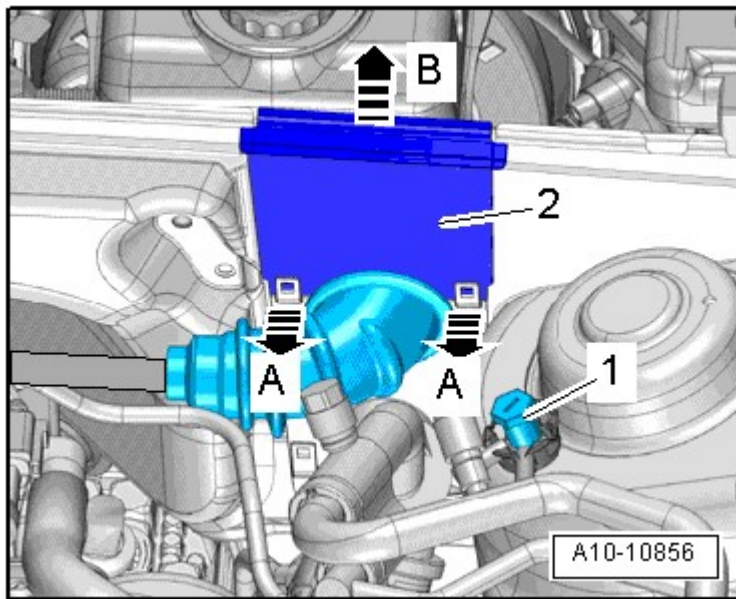
Fig. 132: Disengaging Catches -Arrows A- And Remove Upper Part Of Line Pass-Through -2- Upward - Arrow B-
