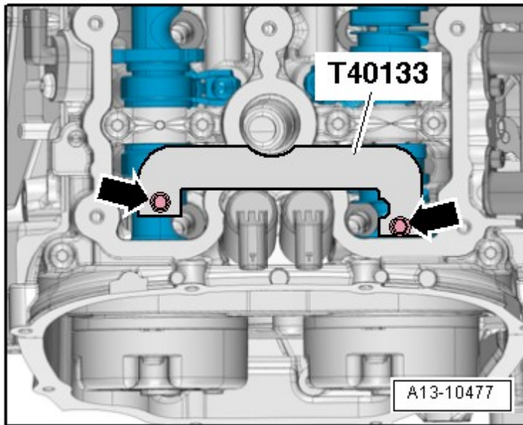
Fig. 96: Camshaft Adjuster T40133 Courtesy of AUDI OF AMERICA, LLC
