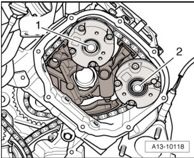
Fig. 92: Identifying Bolts For Camshaft Adjuster Using Multipoint Socket T10035 Courtesy of AUDI OF AMERICA, LLC
