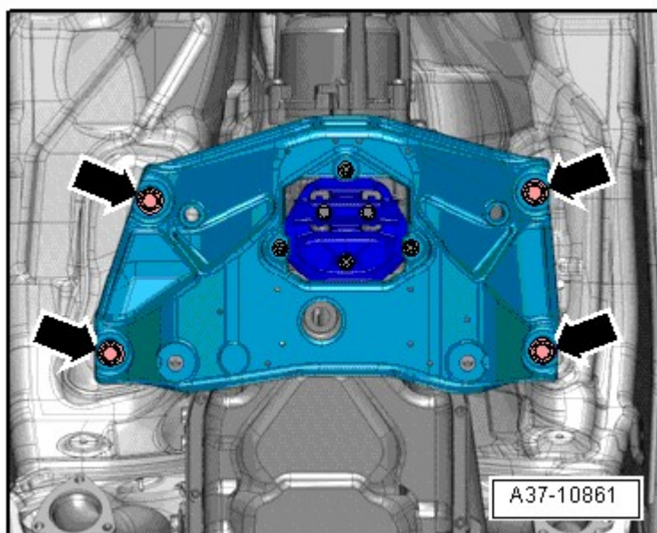
Fig. 189: Identifying Tunnel Crossmember
