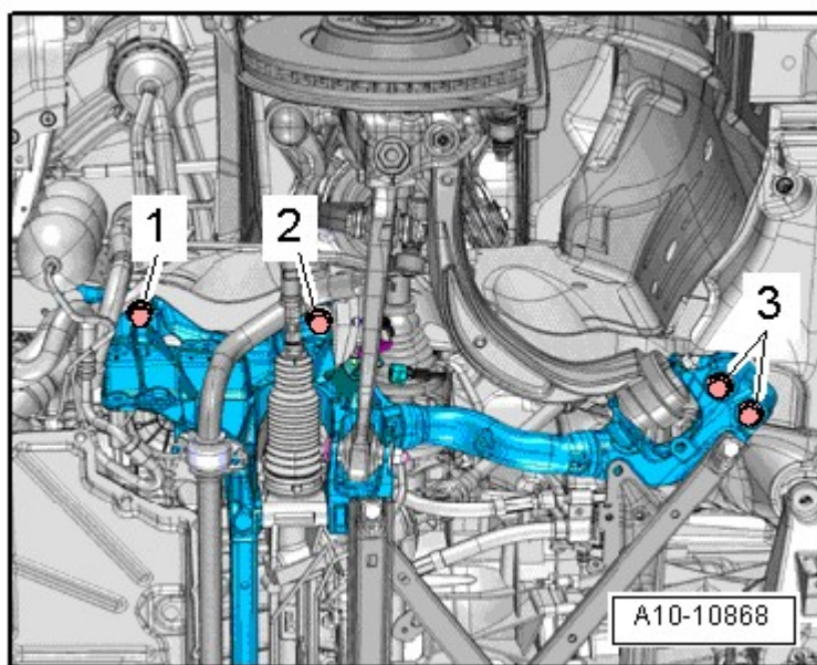
Fig. 188: Identifying Subframe Bolts (Tighten To Specifications)
