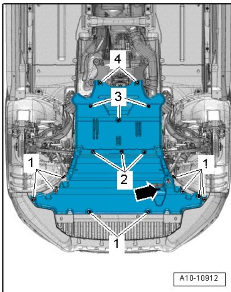
Fig. 23: Identifying Noise Insulation
