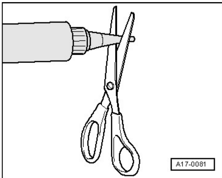
Fig. 51: Cutting Tube Nozzle At Front Marking (Nozzle Diameter Approx. 2 Mm)
