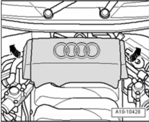
Fig. 592: Removing Rear Engine Cover
