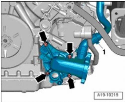
Fig. 489: Loosening Hose Clip At Coolant Hose Courtesy of VOLKSWAGEN UNITED STATES, INC.
