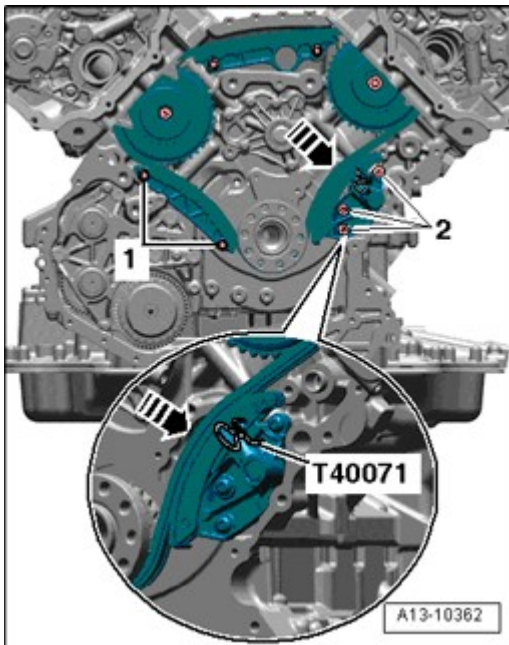
Fig. 314: Pushing Drive Chain Tensioner Guide Rail And Securing Chain Tensioner Using Locking Pin T40071
