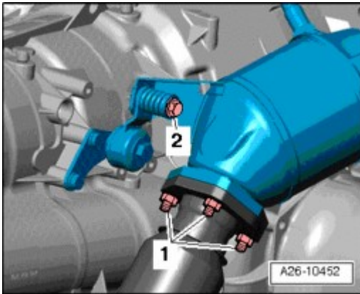
Fig. 88: Removing Right Front Muffler Nuts Courtesy of VOLKSWAGEN UNITED STATES, INC.
