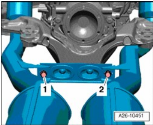
Fig. 543: Removing Bolts
