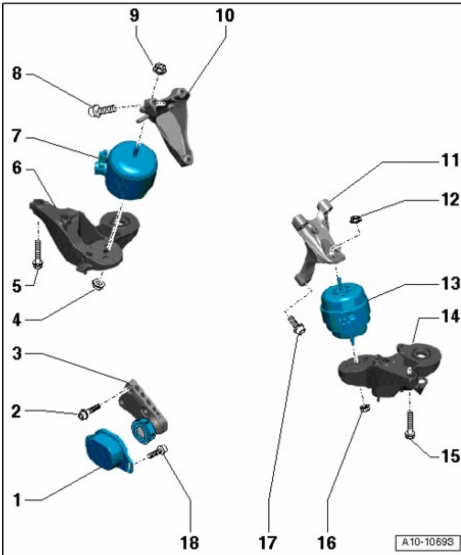
Fig. 122: Assembly Mount, Overview
