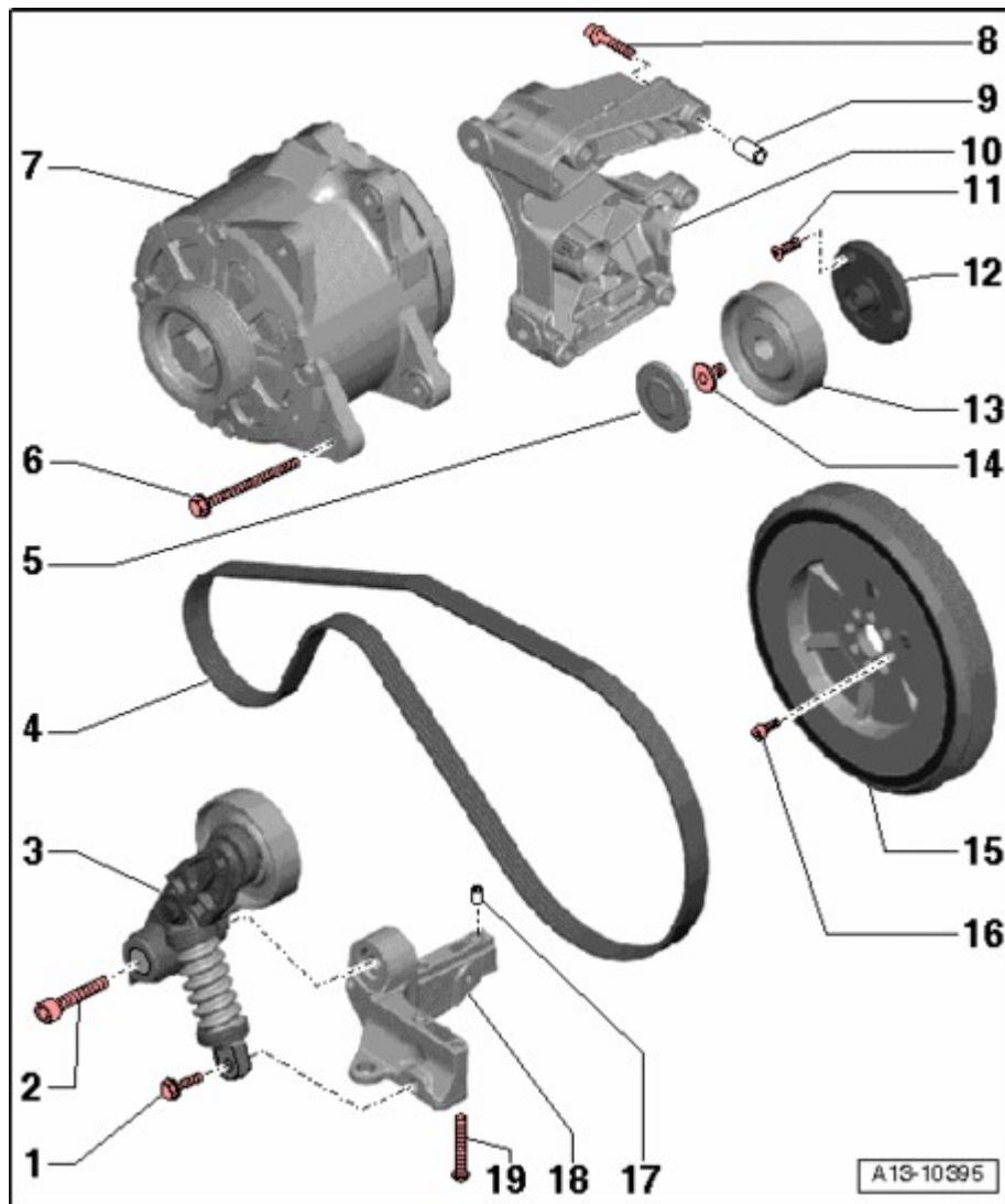
Fig. 157: Ribbed Belt Drive, Assembly Overview
