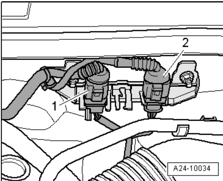
Fig. 575: Disconnecting Electrical Harness Connector For Oxygen Sensor (O2S) Behind Three Way Catalytic Converter (TWC) G130 Courtesy of VOLKSWAGEN UNITED STATES, INC.
