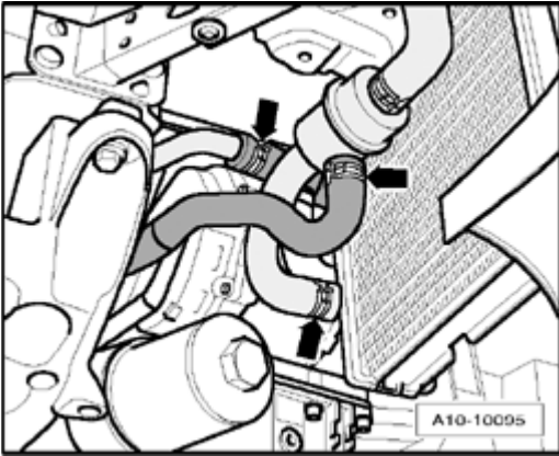
Fig. 15: Coolant Hoses
