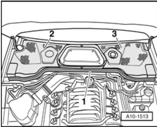
Fig. 356: Plenum Chamber Covers & Rubber Seal
