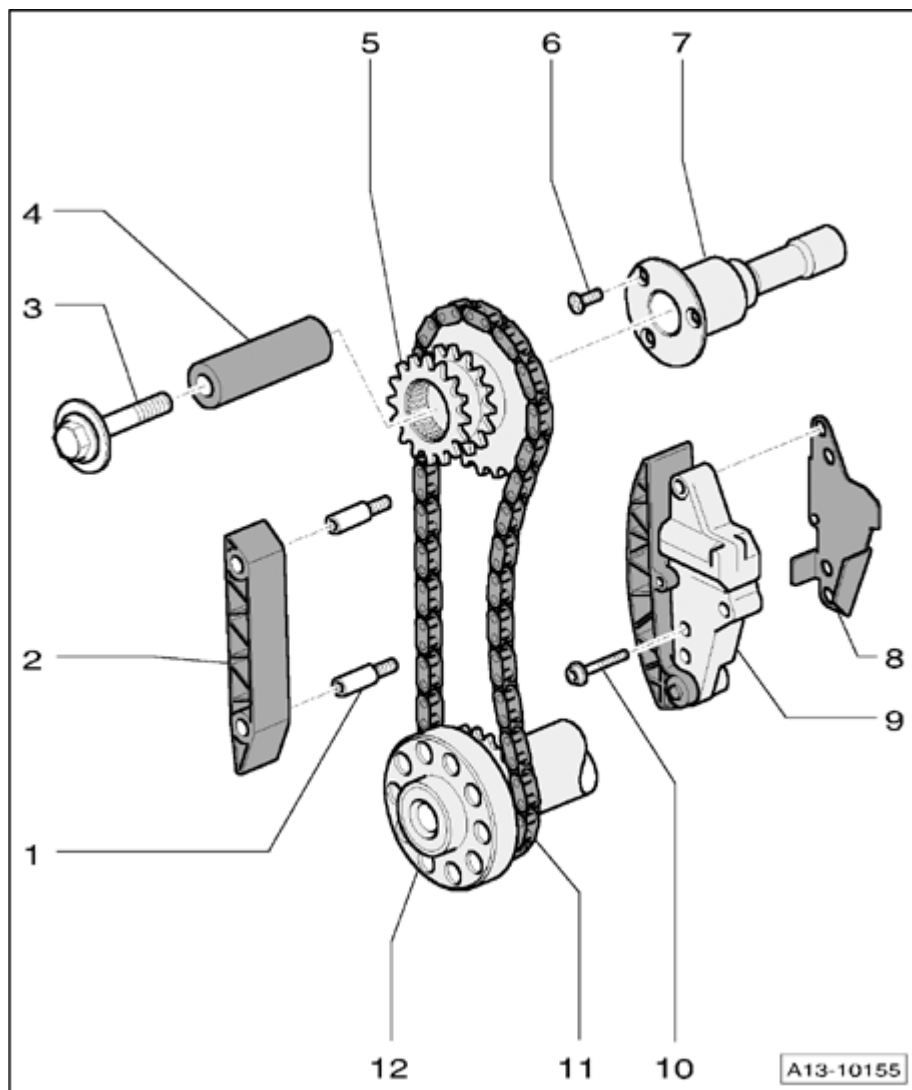
Fig. 192: Drive Chain, Assembly Overview
