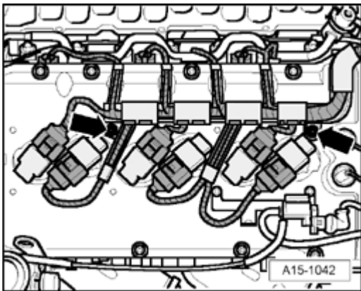
Fig. 201: Removing Bolts
