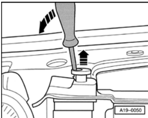
Fig. 445: Releasing Both Fan Shroud Retaining Pins And Removing By Pulling Upward
