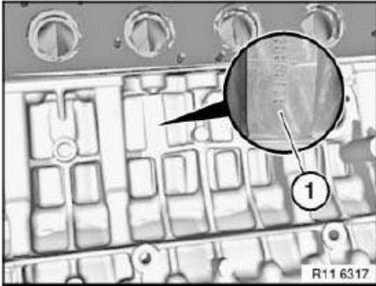
Fig. 124: Identifying Bearing Classification Of Crankcase Upper Section Courtesy of BMW OF NORTH AMERICA, INC.
