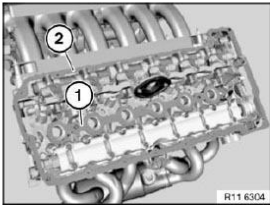
Fig. 36: Identifying Seal And Sealing Faces Courtesy of BMW OF NORTH AMERICA, INC.
