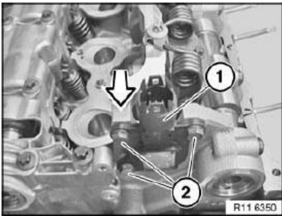
Fig. 296: Identifying Screws And Bolts Courtesy of BMW OF NORTH AMERICA, INC.
