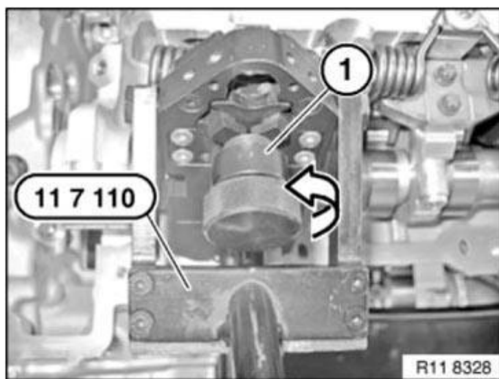
Fig. 275: Releasing Knurled Screw On Special Tool (11 7 110) Courtesy of BMW OF NORTH AMERICA, INC.
