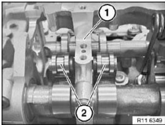
Fig. 256: Identifying Contact Surfaces And Intermediate Levers Courtesy of BMW OF NORTH AMERICA, INC.
