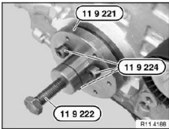
Fig. 63: Identifying Special Tools Courtesy of BMW OF NORTH AMERICA, INC.
