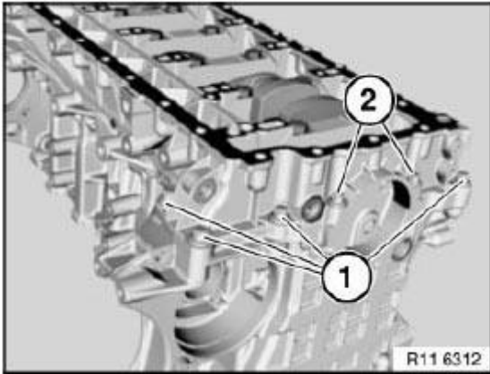
Fig. 105: Identifying Aluminum Screws Courtesy of BMW OF NORTH AMERICA, INC.
