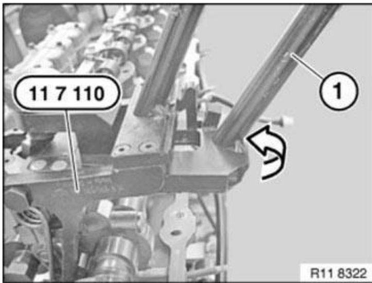
Fig. 271: Preloading Return Spring On Special Tool (11 7 110) Courtesy of BMW OF NORTH AMERICA, INC.
