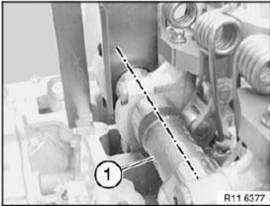
Fig. 178: Identifying Camshaft
