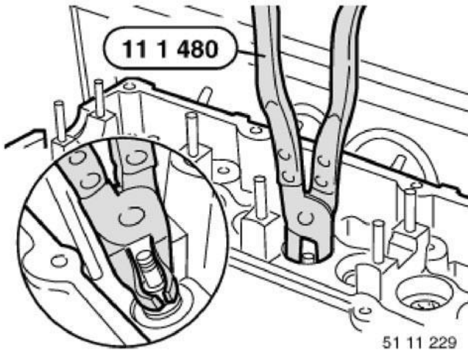
Fig. 222: Identifying Special Tool (11 1 480) Courtesy of BMW OF NORTH AMERICA, INC.
