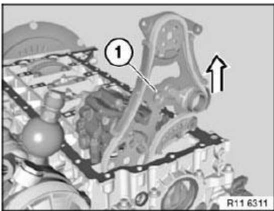
Fig. 310: Removing Screw Plug Courtesy of BMW OF NORTH AMERICA, INC.
