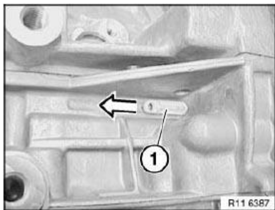
Fig. 193: Removing Fastener
