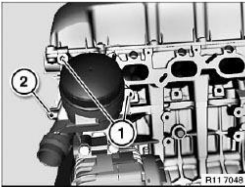
Fig. 316: Identifying Screws
