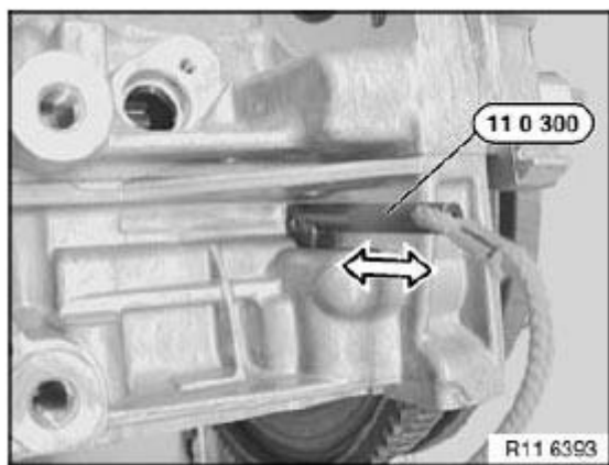
Fig. 194: Securing Crankshaft
