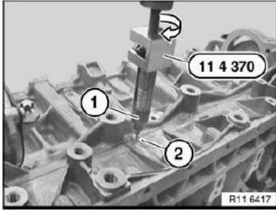
Fig. 116: Inserting Liquid Gasket Using Special Tool (11 4 370) Courtesy of BMW OF NORTH AMERICA, INC.
