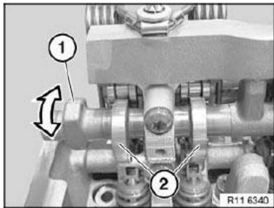
Fig. 265: Moving Eccentric Shaft Courtesy of BMW OF NORTH AMERICA, INC.
