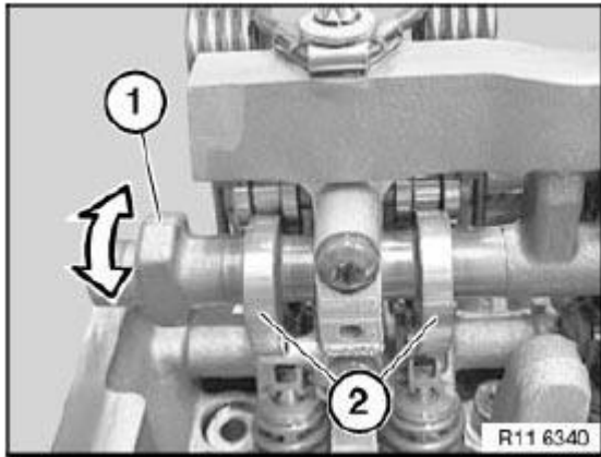
Fig. 236: Removing Eccentric Shaft Courtesy of BMW OF NORTH AMERICA, INC.
