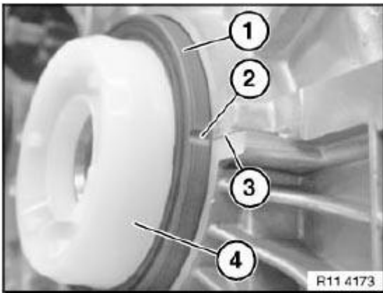
Fig. 86: Fitting Support Sleeve With Radial Shaft Seal On Crankshaft Courtesy of BMW OF NORTH AMERICA, INC.
