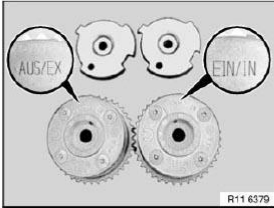
Fig. 233: Identifying AUS And EX Marks For Exhaust Camshaft Courtesy of BMW OF NORTH AMERICA, INC.
