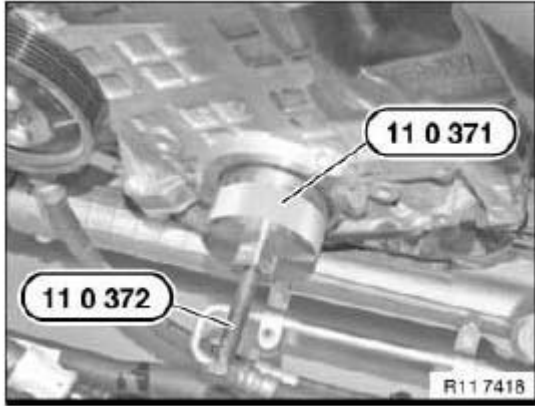
Fig. 64: Identifying Special Tool (11 3 372) Courtesy of BMW OF NORTH AMERICA, INC.
