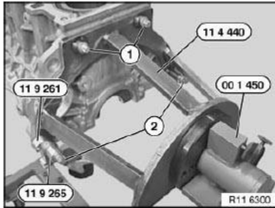
Fig. 32: Identifying Engine Block Steel Bolts And Special Tools Courtesy of BMW OF NORTH AMERICA, INC.
