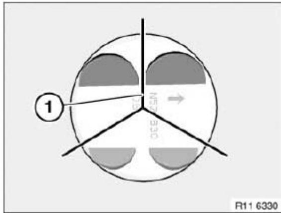
Fig. 162: Identifying Piston Rings Angle Courtesy of BMW OF NORTH AMERICA, INC.
