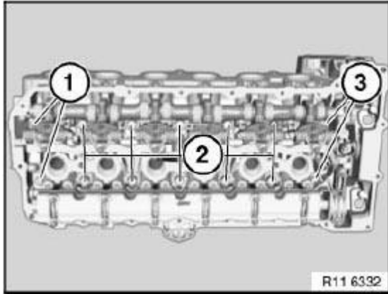
Fig. 44: Identifying Screws
