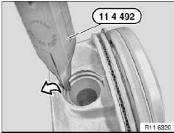
Fig. 149: Removing Piston Pin Circlip With Special Tool (11 4 492)
