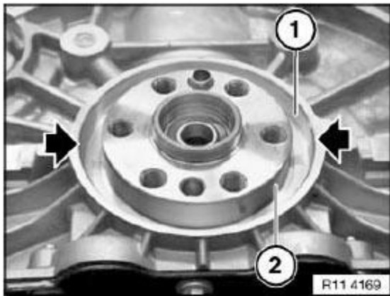
Fig. 91: Identifying Sealing Surface And Running Surface Of Radial Shaft Seal Courtesy of BMW OF NORTH AMERICA, INC.
