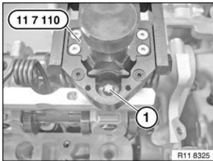
Fig. 300: Tightening Bolt
