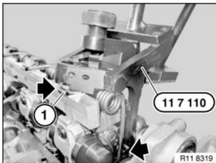
Fig. 276: Positioning Special Tool (11 7 110) On Return Spring Courtesy of BMW OF NORTH AMERICA, INC.
