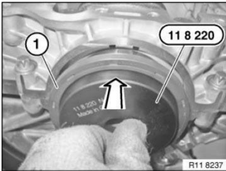
Fig. 169: Positioning Radial Shaft Seal On Crankshaft Using Special Tool 11 8 220 Courtesy of BMW OF NORTH AMERICA, INC.
