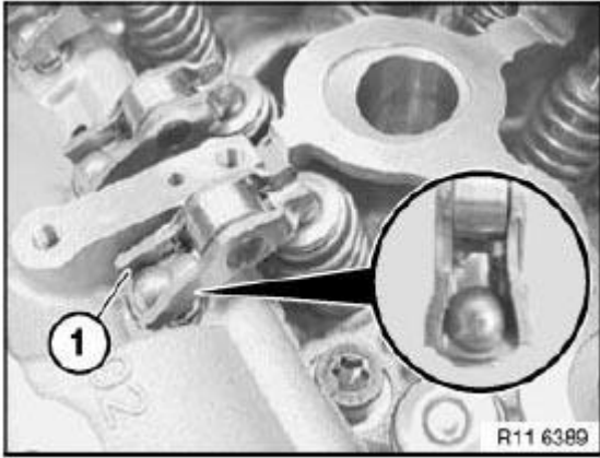
Fig. 299: Identifying Roller Cam Follower Installation Position Courtesy of BMW OF NORTH AMERICA, INC.
