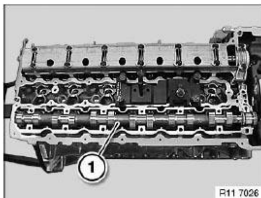
Fig. 260: Identifying Exhaust Camshaft In Lower Bearing Bank Courtesy of BMW OF NORTH AMERICA, INC.
