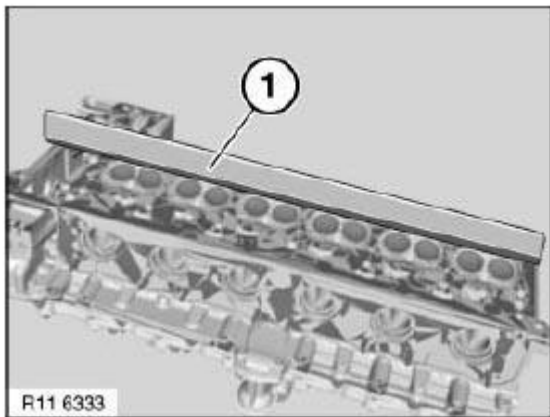
Fig. 67: Checking Evenness Of Cylinder Head Sealing Faces Using Standard Straight-Edge Courtesy of BMW OF NORTH AMERICA, INC.
