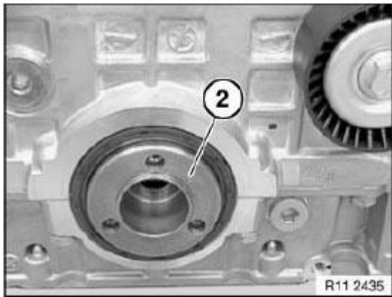
Fig. 338: Identifying Hub Courtesy of BMW OF NORTH AMERICA, INC.
