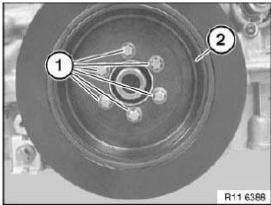
Fig. 193: Identifying Vibration Damper With Mounting Screws Courtesy of BMW OF NORTH AMERICA, INC.
