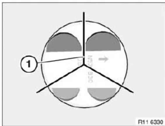
Fig. 223: Off Setting Of Piston Rings Contact Points Courtesy of BMW OF NORTH AMERICA, INC.
