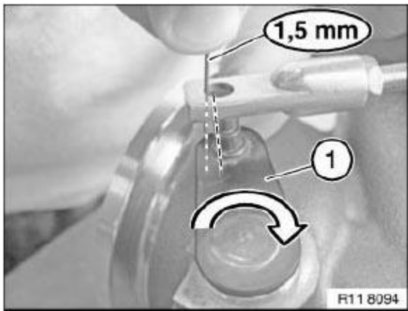
Fig. 416: Identifying Drill Bit Dimension Courtesy of BMW OF NORTH AMERICA, INC.
