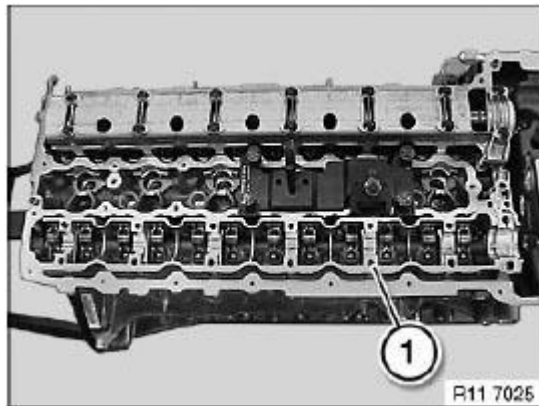
Fig. 259: Identifying Lower Bearing Strip On Cylinder Head Courtesy of BMW OF NORTH AMERICA, INC.
