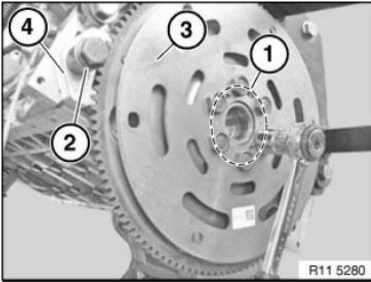
Fig. 153: Identifying Flywheel With Mounting Bolts Courtesy of BMW OF NORTH AMERICA, INC.
