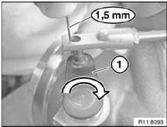
Fig. 415: Sealing Off Wastegate Valve Courtesy of BMW OF NORTH AMERICA, INC.
