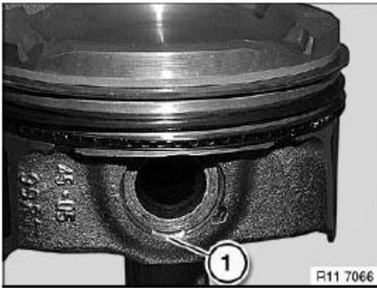
Fig. 211: Position Of Installing Piston Pin Circlip Courtesy of BMW OF NORTH AMERICA, INC.
