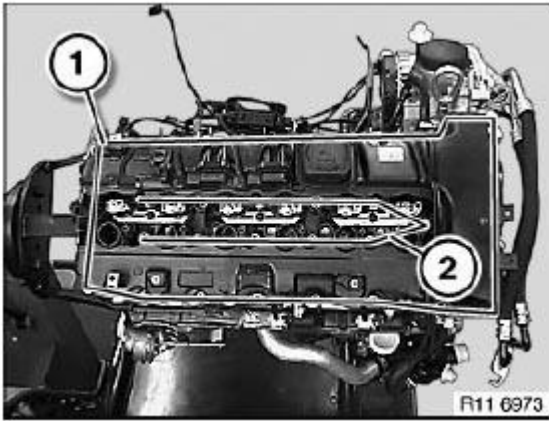
Fig. 48: Identifying Screws
