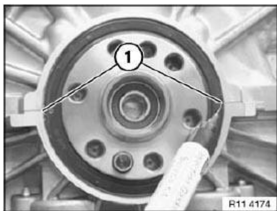
Fig. 100: Filling Both Grooves Flush With Loctite Sealing Compound Courtesy of BMW OF NORTH AMERICA, INC.
