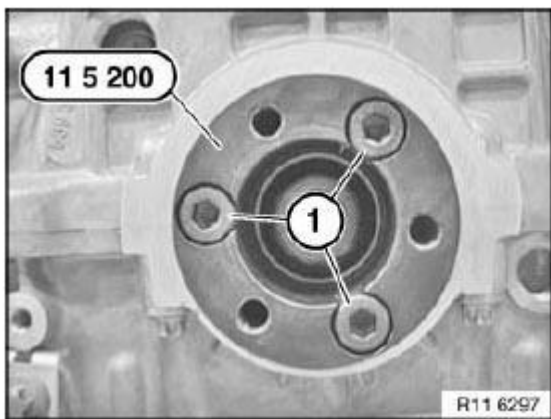
Fig. 348: Identifying Special Tool 11 5 200 Courtesy of BMW OF NORTH AMERICA, INC.
