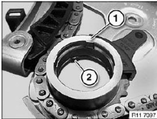
Fig. 285: Identifying Friction Plates Courtesy of BMW OF NORTH AMERICA, INC.
