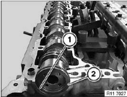
Fig. 261: Identifying Installation Position Of Exhaust Camshaft At Cylinder No. 1 Courtesy of BMW OF NORTH AMERICA, INC.
