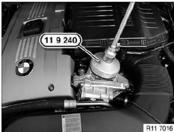
Fig. 6: Identifying Special Tool 11 9 240 For Releasing Oil Filter
