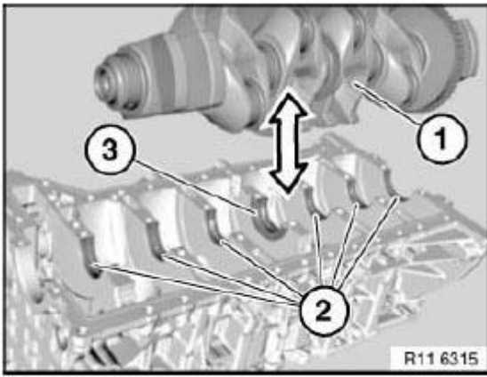
Fig. 130: Identifying Bearing Shells
