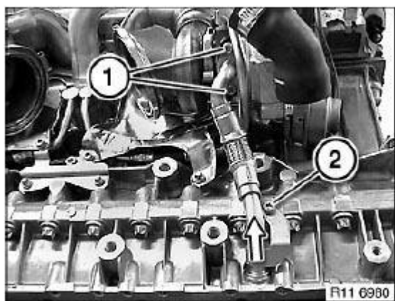
Fig. 389: Identifying Screws
