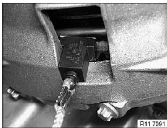
Fig. 275: Securing Flywheel (Crankshaft) Using Special Tool 11 8 660 Courtesy of BMW OF NORTH AMERICA, INC.
