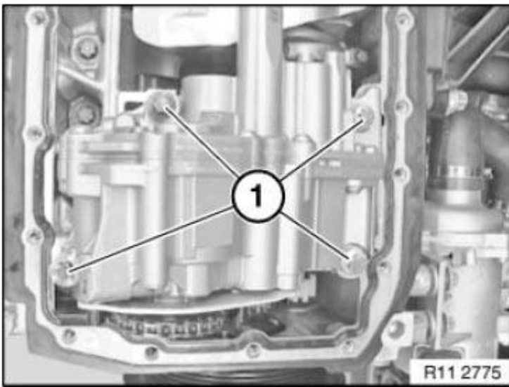
Fig. 148: Identifying Oil Pump Mounting Screws Courtesy of BMW OF NORTH AMERICA, INC.
