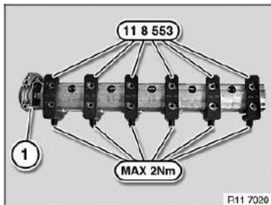
Fig. 250: Identifying Upper And Lower Bearing Strips With Special Tools 11 8 553 Courtesy of BMW OF NORTH AMERICA, INC.
