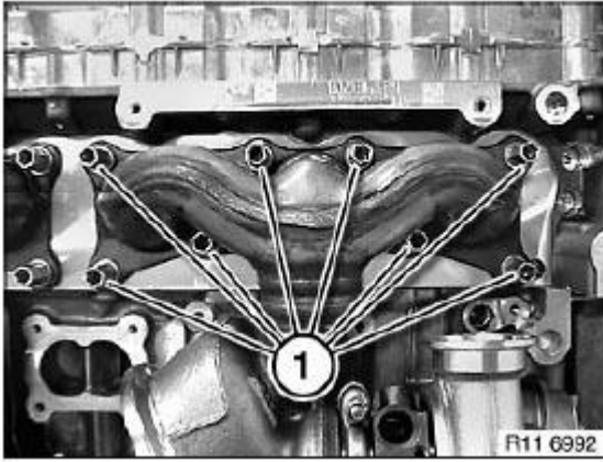
Fig. 398: Identifying Nuts
