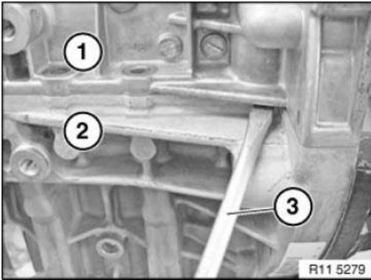
Fig. 157: Removing Crankcase Lower Section From Upper Section Using Tool Courtesy of BMW OF NORTH AMERICA, INC.
