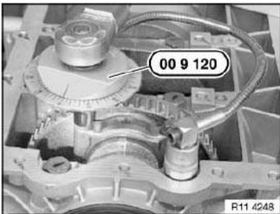
Fig. 217: Adjusting Torsion Angle Of Conrod Using Special Tool 00 9 120 Courtesy of BMW OF NORTH AMERICA, INC.
