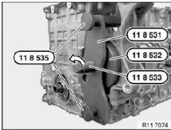
Fig. 87: Identifying Special Tools 11 8 535, 11 8 531 And 11 8 537 Courtesy of BMW OF NORTH AMERICA, INC.
