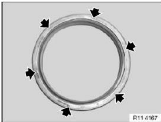
Fig. 72: Locating Crankshaft Radial Seal Removal Openings Courtesy of BMW OF NORTH AMERICA, INC.
