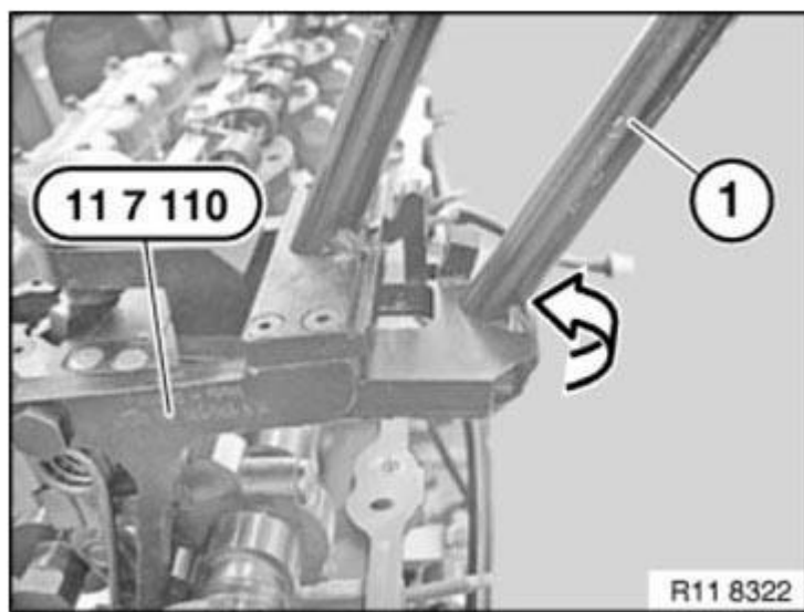
Fig. 335: Identifying Return Spring With Lever And Special Tool 11 7 110 Courtesy of BMW OF NORTH AMERICA, INC.
