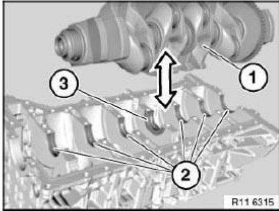
Fig. 117: Removing Guide Bearing Shell And Bearing Shells Courtesy of BMW OF NORTH AMERICA, INC.
