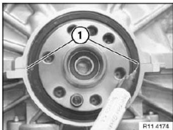
Fig. 82: Filing Grooves With Loctite Sealing Compound Using Injector Courtesy of BMW OF NORTH AMERICA, INC.
