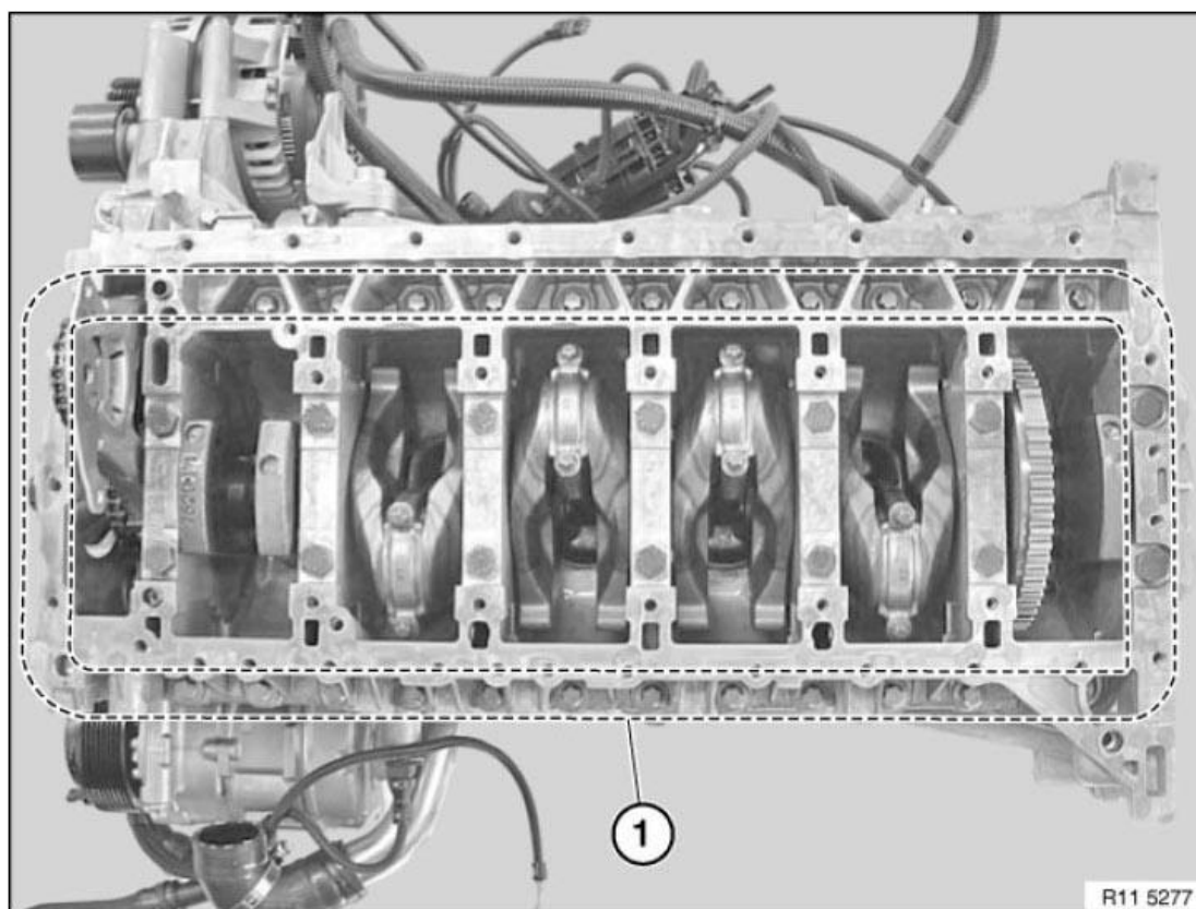
Fig. 155: Identifying Crankshaft Bolt Mounting Area Courtesy of BMW OF NORTH AMERICA, INC.
