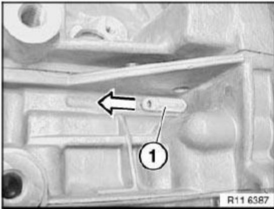
Fig. 239: Installing Fastener
