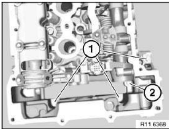
Fig. 59: Identifying Bolts
