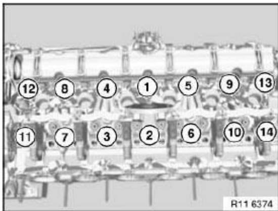
Fig. 58: Insert Cylinder Head Bolts Using Special Tool Courtesy of BMW OF NORTH AMERICA, INC.
