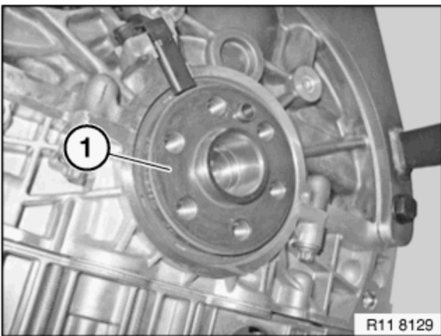
Fig. 84: Identifying Magnet Wheel Courtesy of BMW OF NORTH AMERICA, INC.
