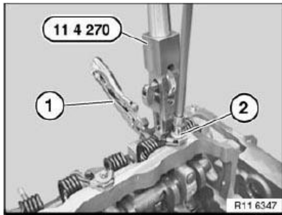
Fig. 326: Identifying Steel Screw Courtesy of BMW OF NORTH AMERICA, INC.
