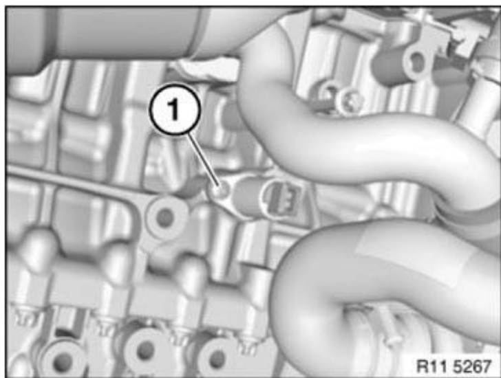
Fig. 232: Identifying Hydraulic Valve Screw Courtesy of BMW OF NORTH AMERICA, INC.
