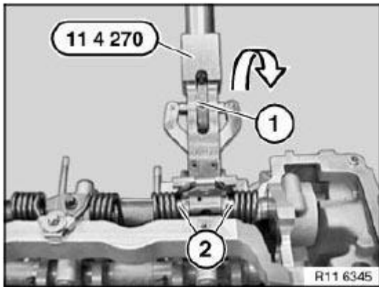
Fig. 334: Securing Bearing Pins Using Special Tool (11 4 270)
