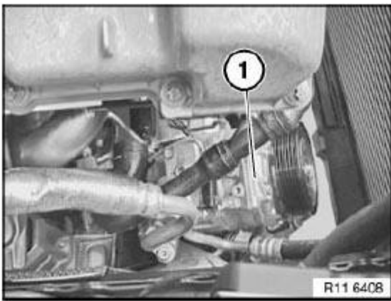
Fig. 23: Identifying Air-Conditioning Compressor Courtesy of BMW OF NORTH AMERICA, INC.
