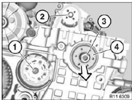
Fig. 385: Removing Hub
