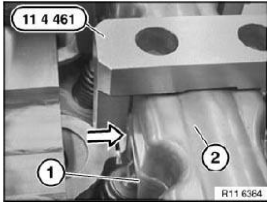
Fig. 265: Positioning Special Tool (11 4 461) On Screw Connection Of Bearing Strips Courtesy of BMW OF NORTH AMERICA, INC.
