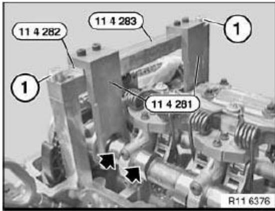
Fig. 302: Releasing Cylinder Head Bolt Courtesy of BMW OF NORTH AMERICA, INC.
