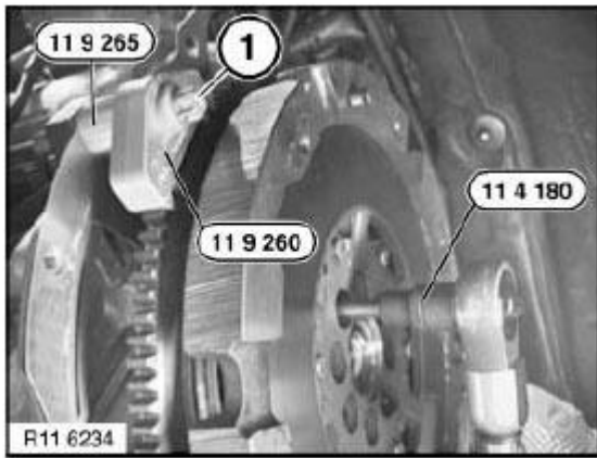
Fig. 127: Releasing Flywheel Bolts Using Special Tool (11 4 180) Courtesy of BMW OF NORTH AMERICA, INC.
