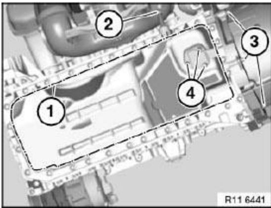
Fig. 71: Identifying Return Hose, Oil Level Sensor Nuts And Bolts Courtesy of BMW OF NORTH AMERICA, INC.
