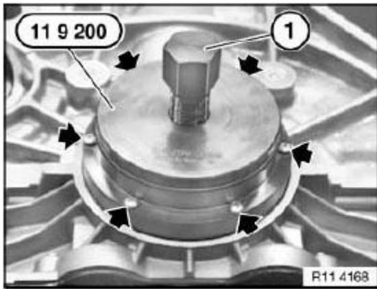
Fig. 98: Locating Crankshaft Radial Seal Screws Courtesy of BMW OF NORTH AMERICA, INC.
