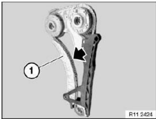
Fig. 307: Identifying Clamping Rail Courtesy of BMW OF NORTH AMERICA, INC.
