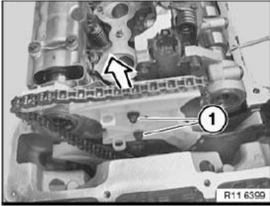
Fig. 283: Removing Chain Module
