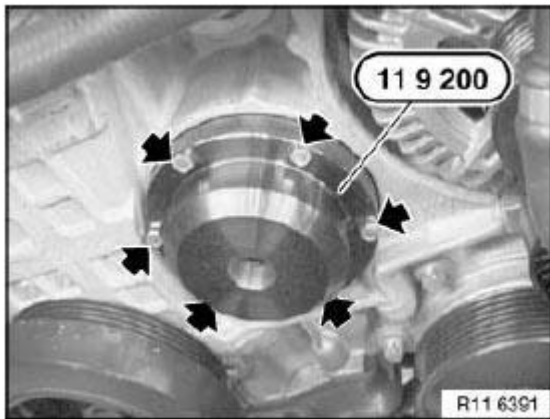
Fig. 122: Inserting Sealing Cover Screws Using Special Tool (11 9 200) Courtesy of BMW OF NORTH AMERICA, INC.
