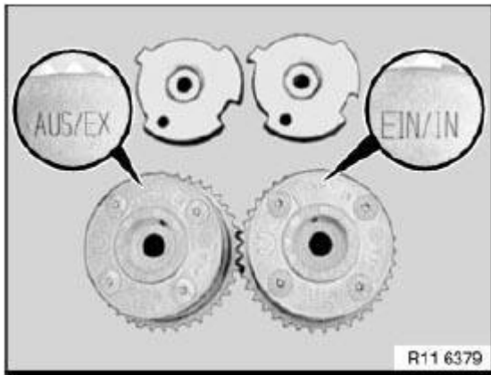
Fig. 305: Identifying Marking On Exhaust And Inlet Camshaft Courtesy of BMW OF NORTH AMERICA, INC.
