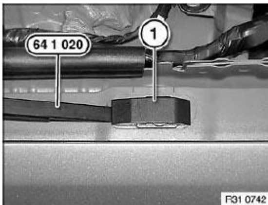
Fig. 32: Removing Cover Caps Using Special Tool (64 1 020)
