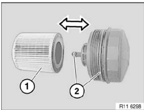
Fig. 374: Disconnecting Oil Filter Element Courtesy of BMW OF NORTH AMERICA, INC.
