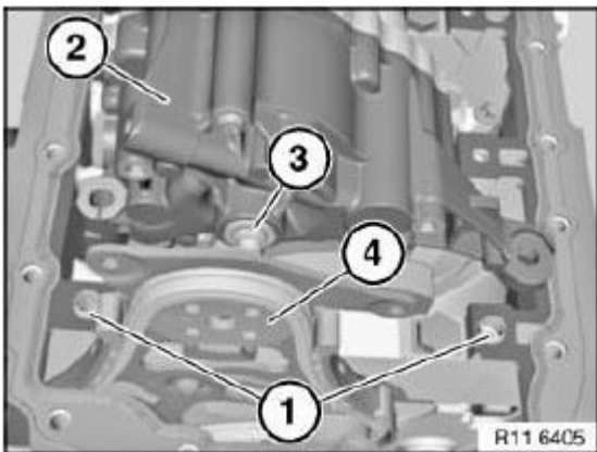
Fig. 396: Identifying Spacer, Oil Pump And Sprocket Wheel Courtesy of BMW OF NORTH AMERICA, INC.
