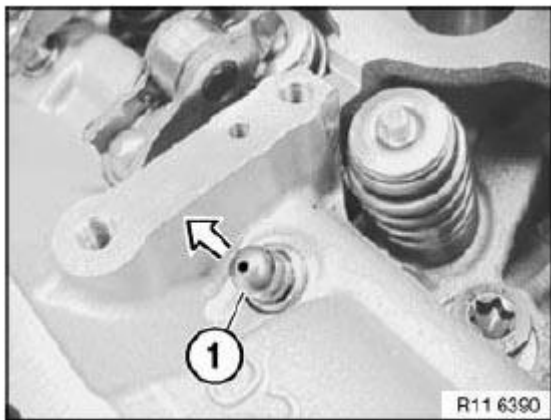
Fig. 291: Removing HVCA Element
