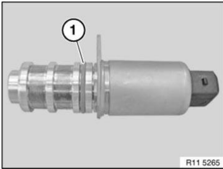
Fig. 233: Identifying O-Ring
