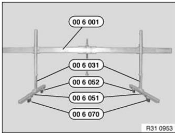
Fig. 39: Identifying Profile Strips, Supports And Connections Of Special Tool Courtesy of BMW OF NORTH AMERICA, INC.
