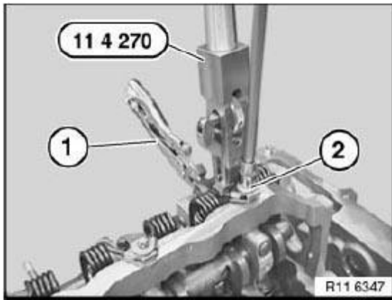
Fig. 335: Inserting Screw Of Torsion Spring Courtesy of BMW OF NORTH AMERICA, INC.
