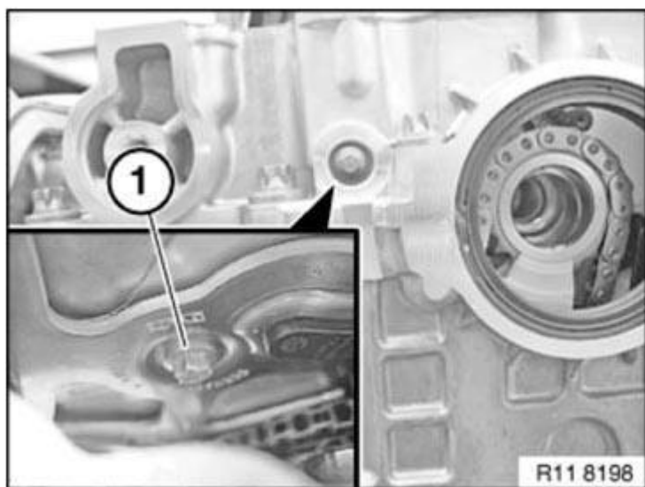
Fig. 382: Identifying Front Hub Screw
