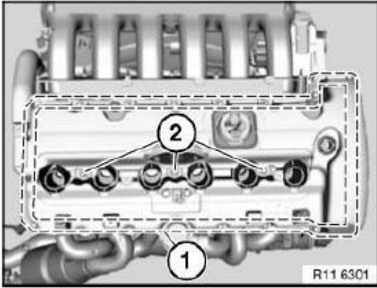
Fig. 61: Identifying Metal Bracket Screws Area And Threaded Pin Courtesy of BMW OF NORTH AMERICA, INC.
