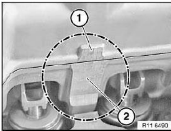
Fig. 263: Identifying Bearing Strips Aligning Area Courtesy of BMW OF NORTH AMERICA, INC.
