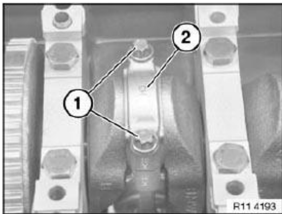
Fig. 223: Identifying Bearing Caps And Connecting Rod Bolts
