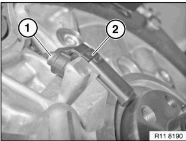
Fig. 85: Identifying Pulse Sensor And Screw Courtesy of BMW OF NORTH AMERICA, INC.
