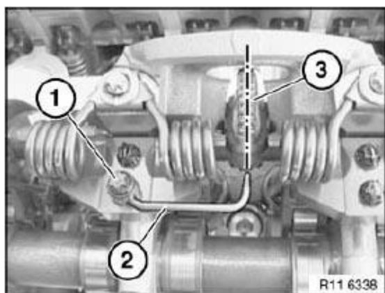
Fig. 336: Identifying Oil Spray Nozzle With Spray Courtesy of BMW OF NORTH AMERICA, INC.
