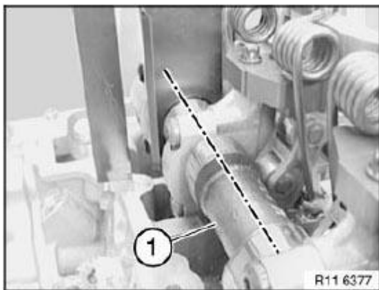
Fig. 241: Identifying Inlet Camshaft Courtesy of BMW OF NORTH AMERICA, INC.
