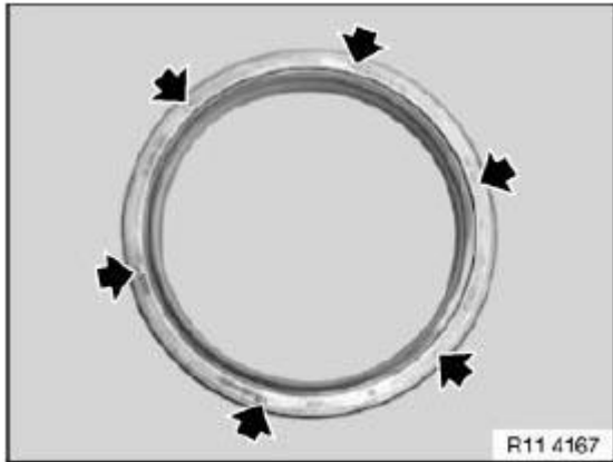
Fig. 121: Locating Crankshaft Radial Seal Openings Courtesy of BMW OF NORTH AMERICA, INC.
