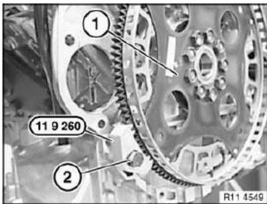
Fig. 198: Securing Flywheel With Existing Transmission Bolt Courtesy of BMW OF NORTH AMERICA, INC.
