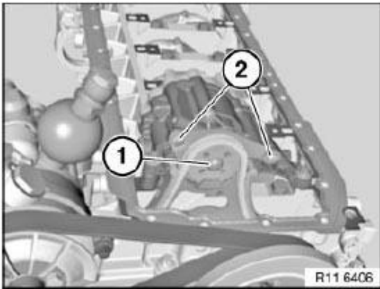
Fig. 379: Identifying Sprocket And Chain Module Screws Courtesy of BMW OF NORTH AMERICA, INC.
