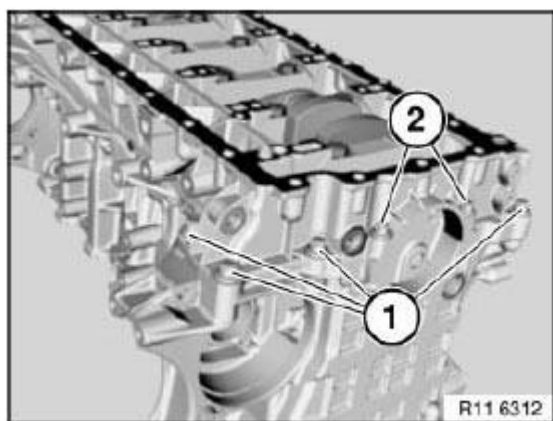
Fig. 138: Identifying Screws
