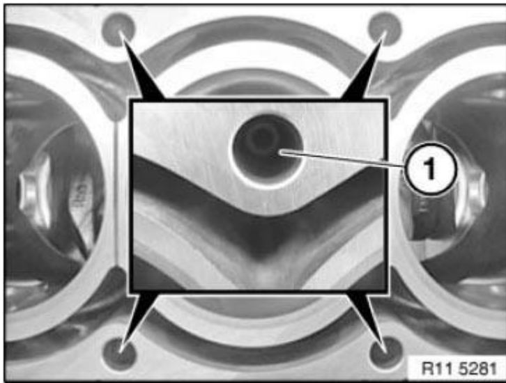
Fig. 57: Identifying Threaded Holes Cylinder Head Bolt Connections Courtesy of BMW OF NORTH AMERICA, INC.
