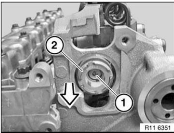
Fig. 47: Removing Magnet Wheel Courtesy of BMW OF NORTH AMERICA, INC.
