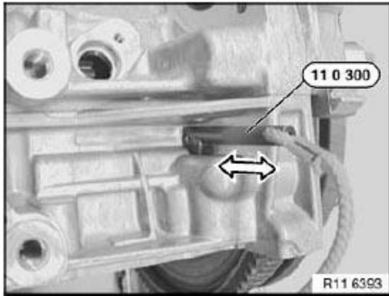
Fig. 240: Sliding Special Tool (11 0 300) Courtesy of BMW OF NORTH AMERICA, INC.
