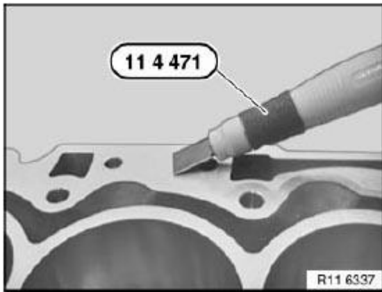
Fig. 55: Removing Coarse Residues Of Sealing Surfaces Using Special Tool (11 4 471) Courtesy of BMW OF NORTH AMERICA, INC.
