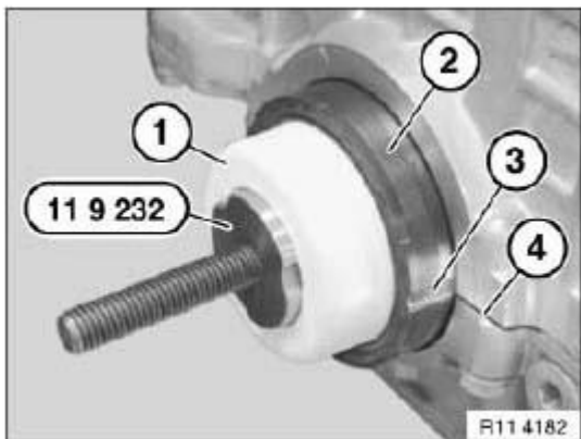
Fig. 116: Pushing Support Sleeve Onto Special Tool (11 9 232) Courtesy of BMW OF NORTH AMERICA, INC.
