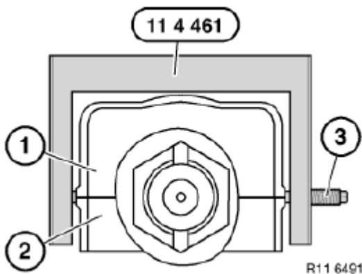
Fig. 264: Identifying Screw, Upper And Lower Bearing Strips Courtesy of BMW OF NORTH AMERICA, INC.
