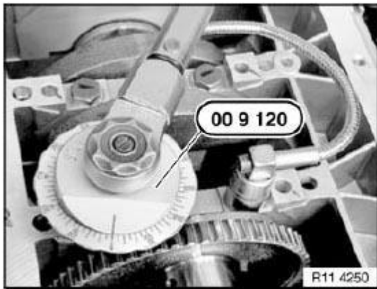
Fig. 145: Tightening Aluminum Screws Using Special Tool (00 9 120) Courtesy of BMW OF NORTH AMERICA, INC.
