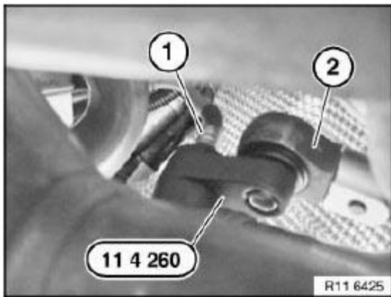
Fig. 412: Releasing Lambda Control Sensor Courtesy of BMW OF NORTH AMERICA, INC.
