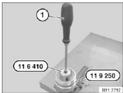
Fig. 371: Inserting Central Screw Using Screwdriver Courtesy of BMW OF NORTH AMERICA, INC.
