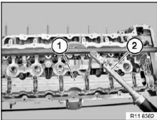
Fig. 262: Tightening Bearing Strips Bolt Courtesy of BMW OF NORTH AMERICA, INC.
