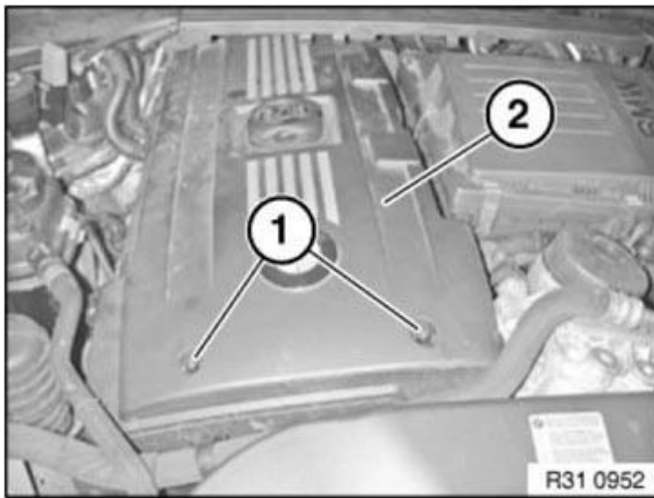
Fig. 35: Identifying Front Screws On Acoustic Cover Courtesy of BMW OF NORTH AMERICA, INC.
