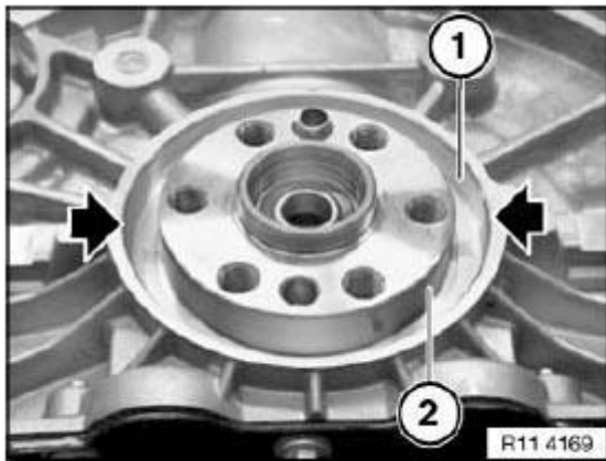
Fig. 99: Identifying Crankshaft Radial Seal Running And Sealing Surfaces Courtesy of BMW OF NORTH AMERICA, INC.
