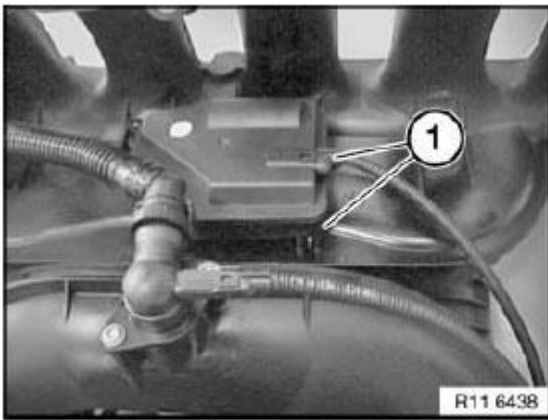
Fig. 407: Identifying Air Intake Manifold Plug Connections Courtesy of BMW OF NORTH AMERICA, INC.
