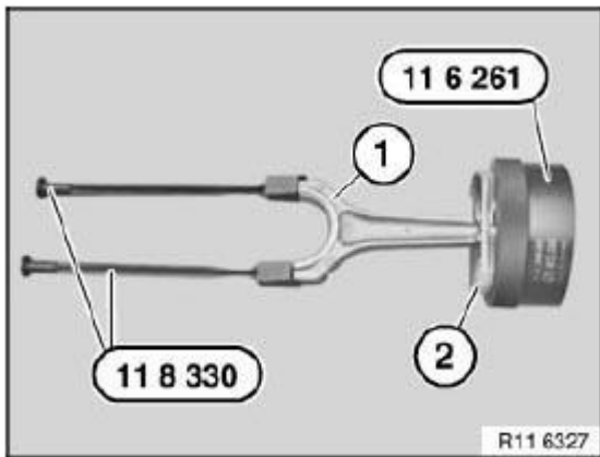
Fig. 218: Attaching Special Tool (11 8 330) To Connecting Rod Courtesy of BMW OF NORTH AMERICA, INC.
