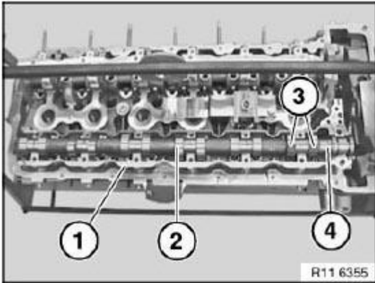
Fig. 261: Identifying Lower Bearing Strip, Exhaust Camshaft And Cams Courtesy of BMW OF NORTH AMERICA, INC.
