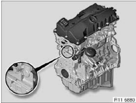
Fig. 9: Identifying Engine Identification Mark - N42/N46/N46T Courtesy of BMW OF NORTH AMERICA, INC.
