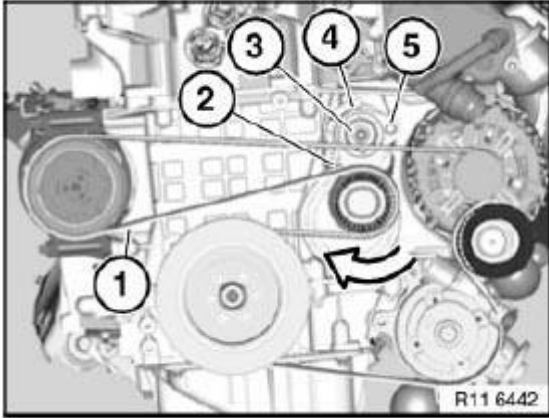
Fig. 237: Turning Belt Tensioner (E9X) Courtesy of BMW OF NORTH AMERICA, INC.
