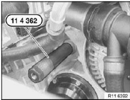
Fig. 123: Identifying Special Tool (11 4 362) Courtesy of BMW OF NORTH AMERICA, INC.
