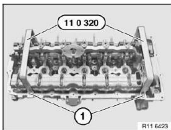
Fig. 53: Securing Special Tool (11 0 320) With Cylinder Head Bolts Courtesy of BMW OF NORTH AMERICA, INC.
