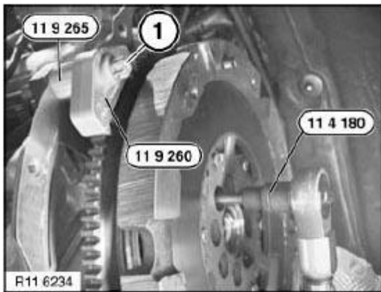
Fig. 199: Securing Flywheel With Transmission Bolt Courtesy of BMW OF NORTH AMERICA, INC.
