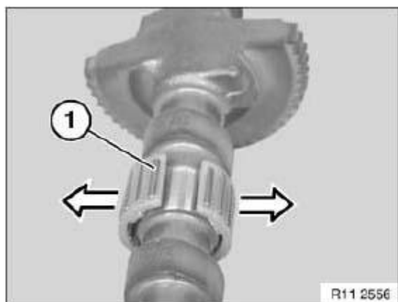
Fig. 312: Removing Needle Bearing From Eccentric Shaft Courtesy of BMW OF NORTH AMERICA, INC.
