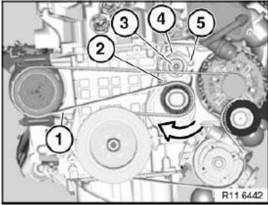
Fig. 234: Turning Belt Tensioner And Drive Belt Routing (E9X) Courtesy of BMW OF NORTH AMERICA, INC.
