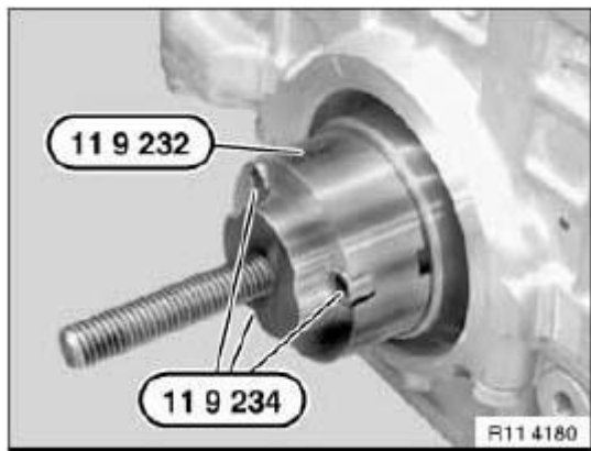
Fig. 113: Inserting Special Tool (11 9 232) With Screws Into Crankshaft Courtesy of BMW OF NORTH AMERICA, INC.
