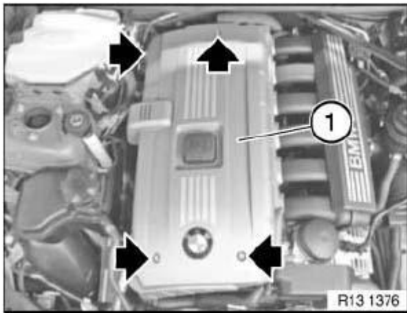
Fig. 29: Locating Acoustic Cover Screws Courtesy of BMW OF NORTH AMERICA, INC.
