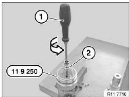
Fig. 369: Releasing Insert Using Screwdriver Courtesy of BMW OF NORTH AMERICA, INC.
