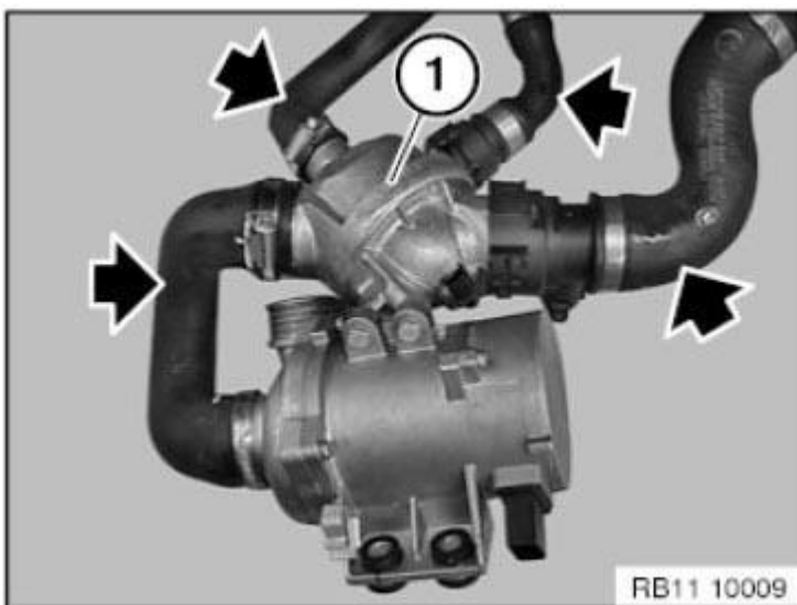
Fig. 401: Locating Coolant Hoses On Thermostat
