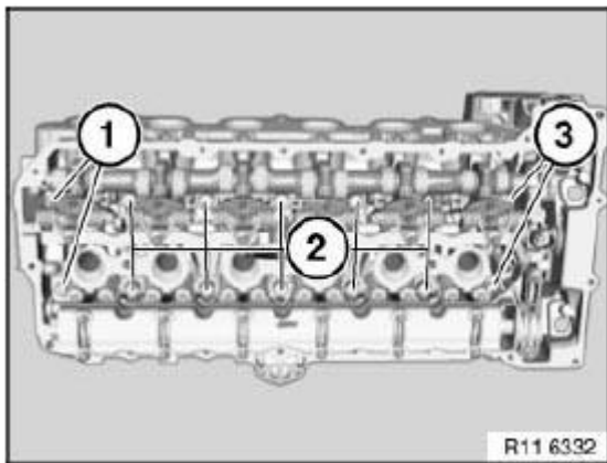
Fig. 52: Identifying Cylinder Head Bolts Courtesy of BMW OF NORTH AMERICA, INC.
