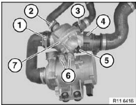
Fig. 402: Identifying Coolant Thermostat, Hose Clamps, Coolant Hoses And Screws Courtesy of BMW OF NORTH AMERICA, INC.
