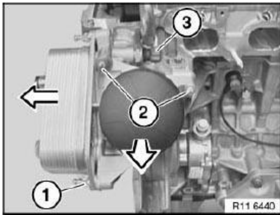
Fig. 366: Disconnecting Plug Connection Of Oil Pressure Switch Courtesy of BMW OF NORTH AMERICA, INC.
