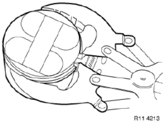
Fig. 226: Removing Compression Ring And Stepped Ring Courtesy of BMW OF NORTH AMERICA, INC.
