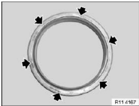
Fig. 96: Locating Crankshaft Radial Seal Openings Courtesy of BMW OF NORTH AMERICA, INC.
