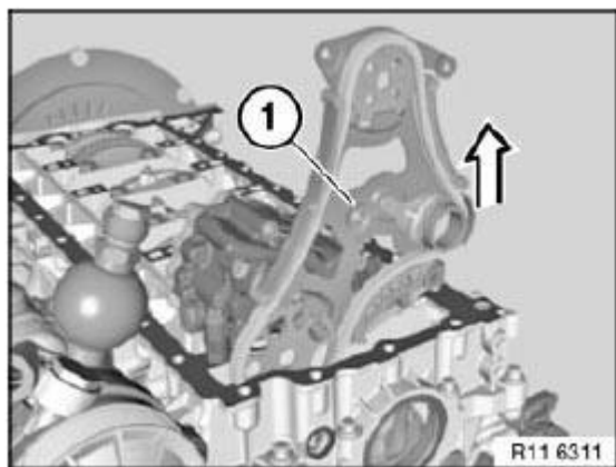
Fig. 383: Removing Chain Module
