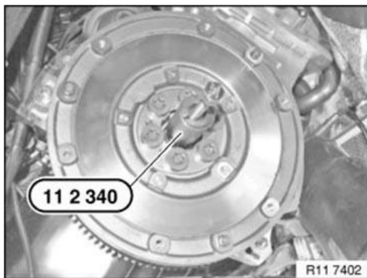
Fig. 151: Removing Guide Bearing Using Special Tool (11 2 340) Courtesy of BMW OF NORTH AMERICA, INC.
