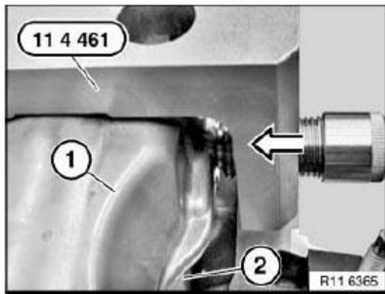
Fig. 266: Tightening Screw Of Special Tool (11 4 461) Courtesy of BMW OF NORTH AMERICA, INC.
