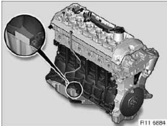
Fig. 13: Identifying Engine Identification Mark - S54 Courtesy of BMW OF NORTH AMERICA, INC.
