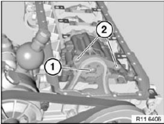
Fig. 393: Identifying Sprocket Wheel And Chain Module Screws And Bolts Courtesy of BMW OF NORTH AMERICA, INC.
