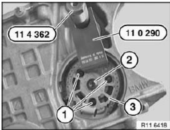
Fig. 410: Identifying Special Tool (11 0 290) And (11 4 362) Courtesy of BMW OF NORTH AMERICA, INC.
