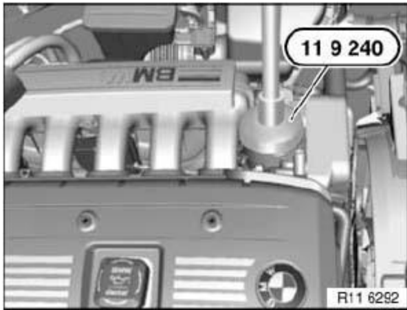
Fig. 373: Releasing Oil Filter Cap Using Special Tool (11 9 240) Courtesy of BMW OF NORTH AMERICA, INC.
