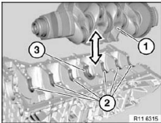
Fig. 129: Removing Bearing Shell Courtesy of BMW OF NORTH AMERICA, INC.
