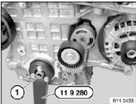
Fig. 380: Releasing Central Screw Courtesy of BMW OF NORTH AMERICA, INC.
