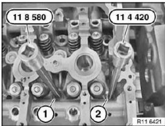
Fig. 51: Releasing Cylinder Head Bolt Using Special Tool (11 8 580) Courtesy of BMW OF NORTH AMERICA, INC.
