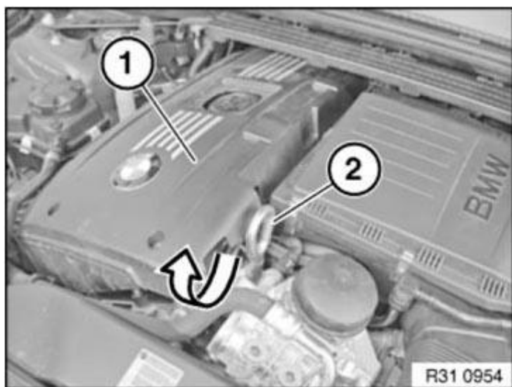
Fig. 36: Raising Acoustic Cover
