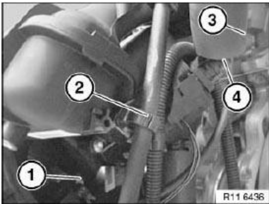
Fig. 403: Identifying Plug Connection, Crankcase Breathers And Holder Courtesy of BMW OF NORTH AMERICA, INC.
