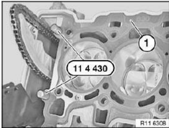
Fig. 64: Inserting Special Tool (11 4 430) Into Bores Courtesy of BMW OF NORTH AMERICA, INC.
