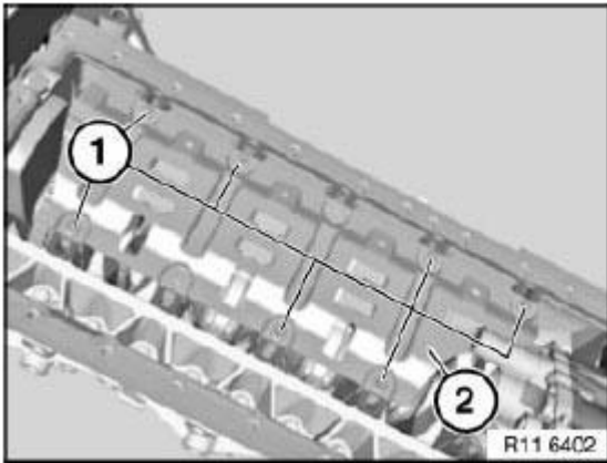
Fig. 137: Identifying Oil Deflector And Screws Courtesy of BMW OF NORTH AMERICA, INC.
