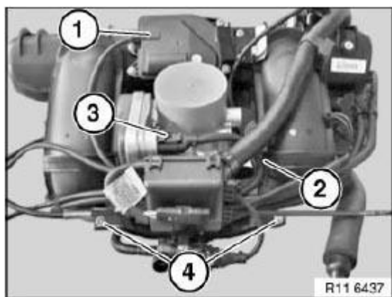
Fig. 404: Identifying Engine Wiring Harness Courtesy of BMW OF NORTH AMERICA, INC.
