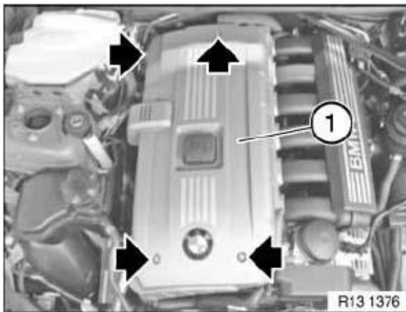
Fig. 28: Locating Acoustic Cover Screws
