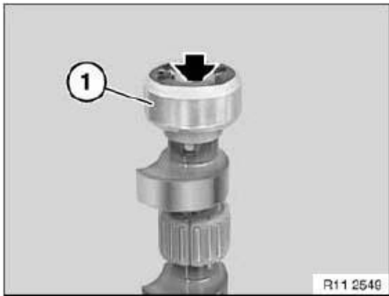
Fig. 310: Identifying Magnet Wheel
