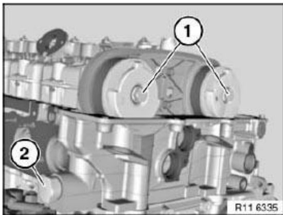
Fig. 303: Identifying Inlet/Exhaust Adjustment Units And Chain Tensioner Courtesy of BMW OF NORTH AMERICA, INC.
