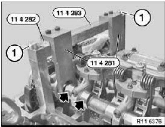
Fig. 282: Securing Special Tool (11 4 283) To Cylinder Head With Bolts Courtesy of BMW OF NORTH AMERICA, INC.
