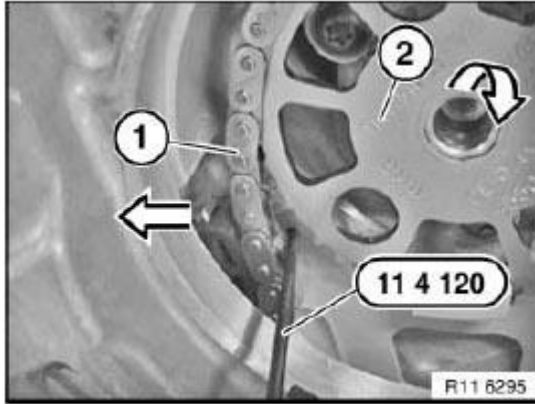
Fig. 411: Removing Camshaft Sprocket Courtesy of BMW OF NORTH AMERICA, INC.
