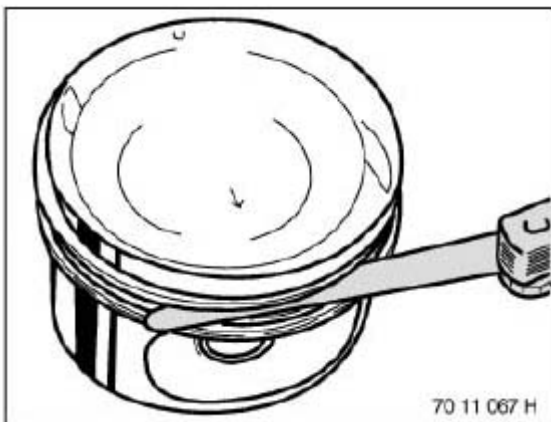
Fig. 225: Measuring Axial Clearance Of Piston Rings Courtesy of BMW OF NORTH AMERICA, INC.
