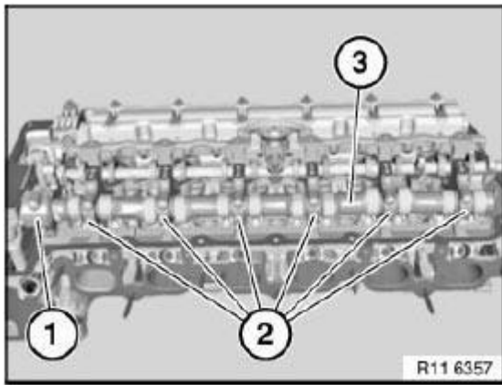
Fig. 270: Identifying Bearing Caps
