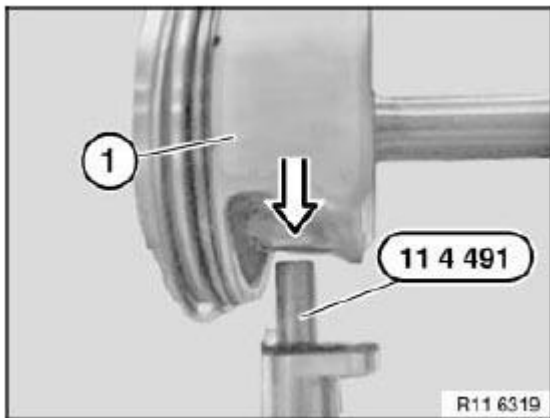
Fig. 211: Securing Piston With Connecting Rod To Special Tool (11 4 491) Courtesy of BMW OF NORTH AMERICA, INC.
