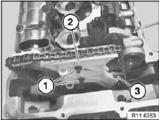
Fig. 45: Identifying Timing Chain Module With Mounting Screws Courtesy of BMW OF NORTH AMERICA, INC.
