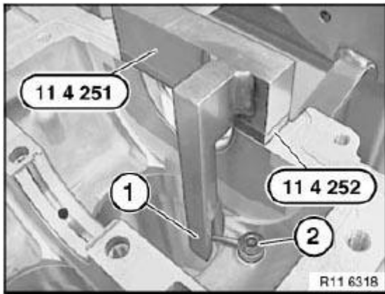
Fig. 128: Checking Oil Spray Nozzle Position On Special Tool (11 4 251) Courtesy of BMW OF NORTH AMERICA, INC.
