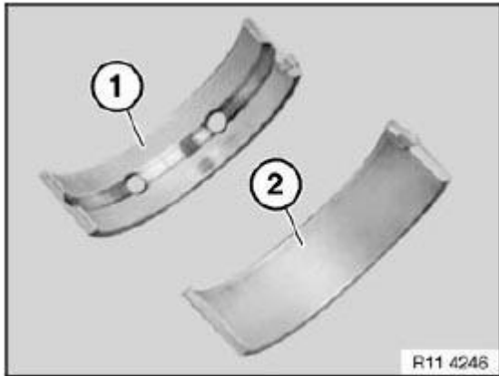
Fig. 134: Identifying Bearing Shell With/Without Lubricant Groove Courtesy of BMW OF NORTH AMERICA, INC.
