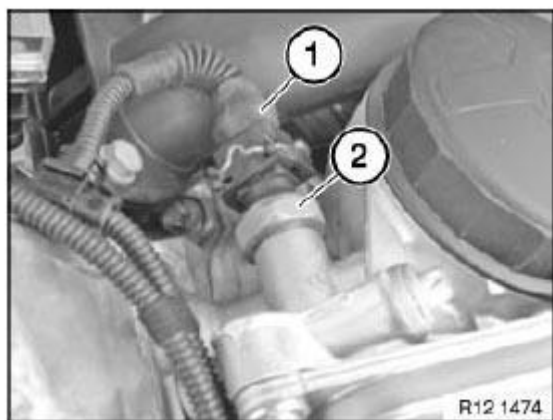
Fig. 405: Identifying Plug Connection On Oil Pressure Switch Courtesy of BMW OF NORTH AMERICA, INC.
