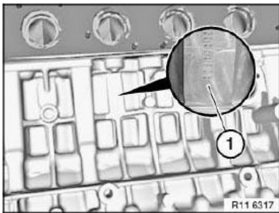
Fig. 132: Identifying Bearing Classification On Crankcase Courtesy of BMW OF NORTH AMERICA, INC.
