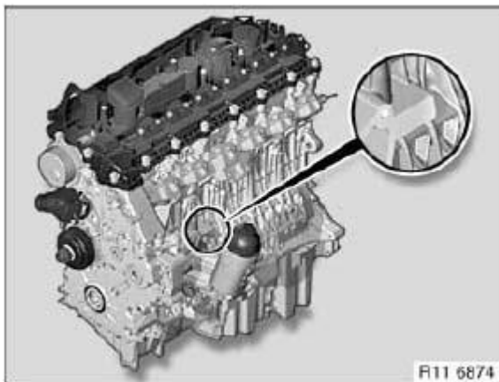
Fig. 2: Identifying Engine Identification Mark - M57/M57TU/M57T2 Courtesy of BMW OF NORTH AMERICA, INC.
