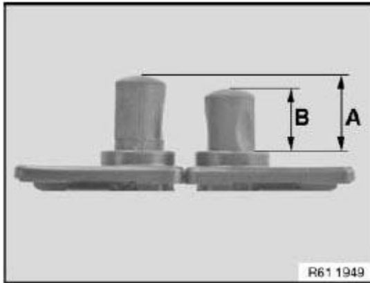
Fig. 31: Identifying Basic Setting For Engine Hood/Bonnet Courtesy of BMW OF NORTH AMERICA, INC.
