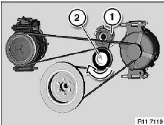
Fig. 235: Turning Belt Tensioner And Drive Belt Routing (E85) Courtesy of BMW OF NORTH AMERICA, INC.
