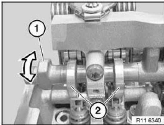
Fig. 317: Moving Eccentric Shaft Courtesy of BMW OF NORTH AMERICA, INC.
