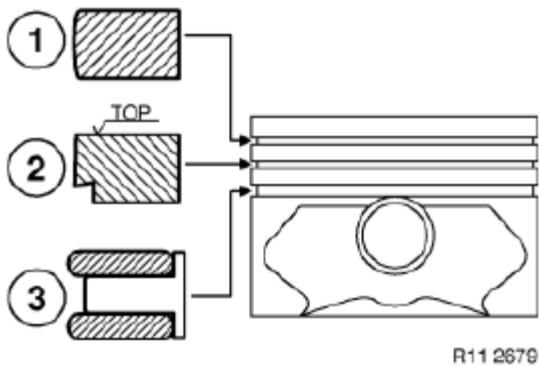
Fig. 228: Identifying Piston Rings
