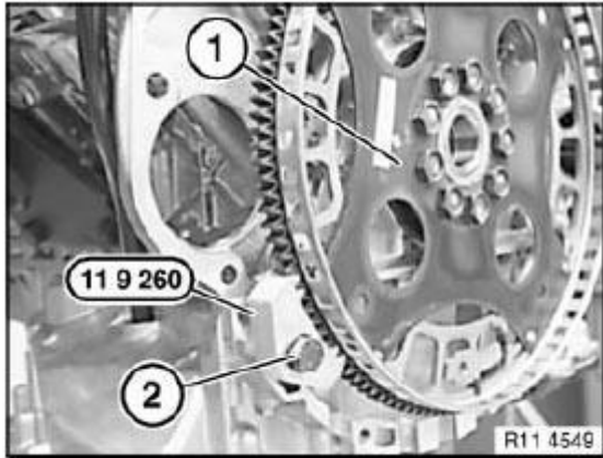
Fig. 126: Securing Flywheel With Existing Transmission Bolt Courtesy of BMW OF NORTH AMERICA, INC.
