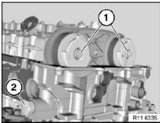
Fig. 306: Identifying Central Bolts Courtesy of BMW OF NORTH AMERICA, INC.
