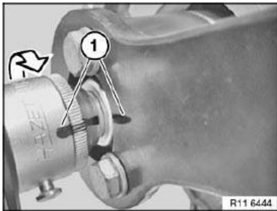
Fig. 388: Tightening Central Bolt To Angle Of Rotation Courtesy of BMW OF NORTH AMERICA, INC.
