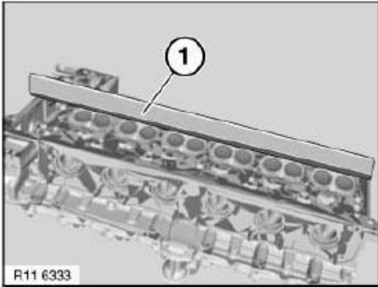
Fig. 68: Checking Cylinder Head Sealing Faces Evenness Using Standard Straight-Edge (Longitudinal) Courtesy of BMW OF NORTH AMERICA, INC.
