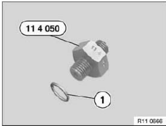
Fig. 367: Identifying Sealing Ring And Special Tool (11 4 050) Courtesy of BMW OF NORTH AMERICA, INC.
