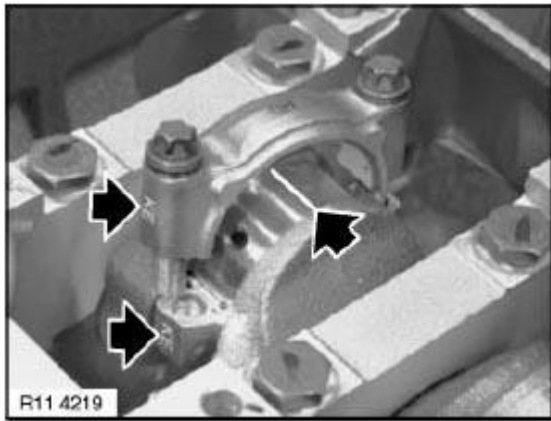
Fig. 204: Locating Bearing Cap Pairing Letters Courtesy of BMW OF NORTH AMERICA, INC.
