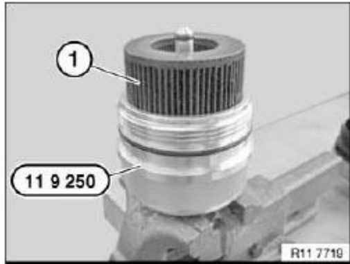
Fig. 375: Installing Filter Element On Special Tool (11 9 250) Courtesy of BMW OF NORTH AMERICA, INC.
