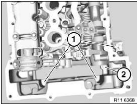
Fig. 59: Identifying Timing Chain Module Screws And Bolts Courtesy of BMW OF NORTH AMERICA, INC.
