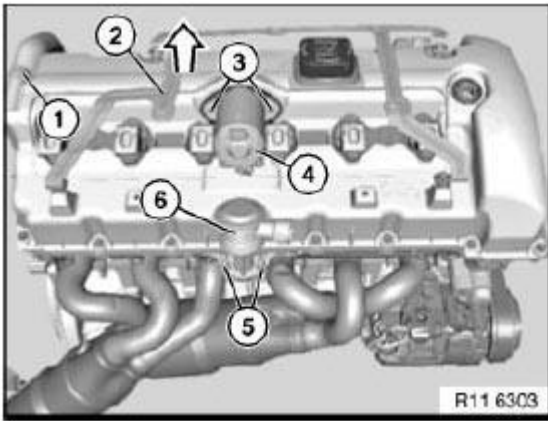
Fig. 60: Pulling Metal Bracket Courtesy of BMW OF NORTH AMERICA, INC.
