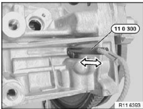
Fig. 249: Sliding Special Tool (11 0 300)
