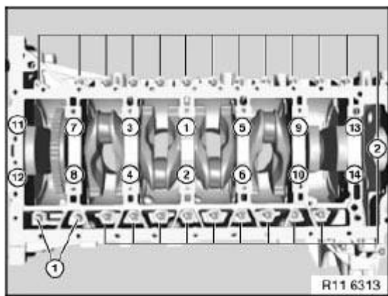
Fig. 139: Crankshaft Cover Screws In Tightening Sequence
