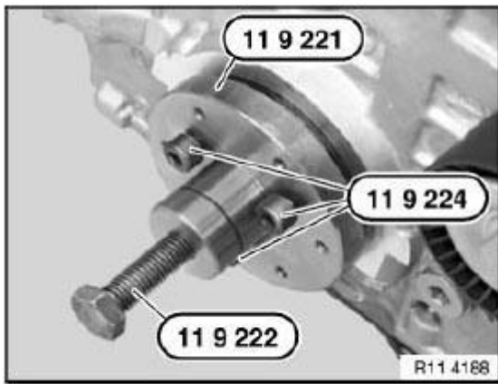
Fig. 109: Pushing Special Tools (11 9 221) Onto Crankshaft Courtesy of BMW OF NORTH AMERICA, INC.
