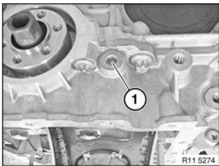
Fig. 179: Identifying Crankcase Screws Plug Courtesy of BMW OF NORTH AMERICA, INC.
