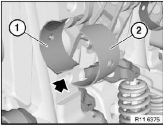
Fig. 314: Identifying Bearing Shell
