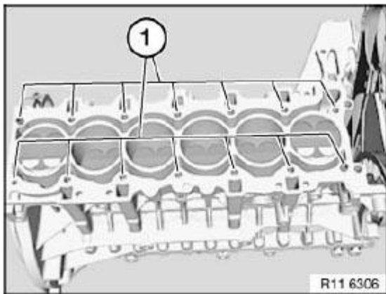
Fig. 65: Identifying Threaded Holes Of Cylinder Head Connections Courtesy of BMW OF NORTH AMERICA, INC.
