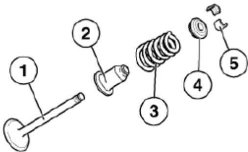
Fig. 292: Identifying Upper/Lower Spring Plate, Valve Spring And Stem Seal Courtesy of BMW OF NORTH AMERICA, INC.
