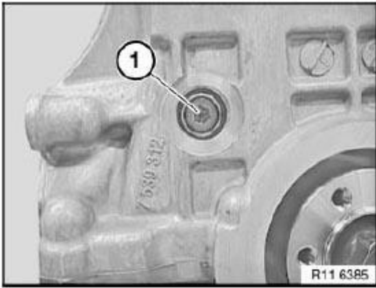
Fig. 281: Identifying Timing Chain Module Bearing Pin (Crankcase) Courtesy of BMW OF NORTH AMERICA, INC.
