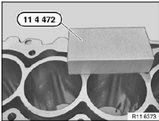
Fig. 56: Removing Fine Residues Of Sealing Surfaces Using Special Tool (11 4 472) Courtesy of BMW OF NORTH AMERICA, INC.
