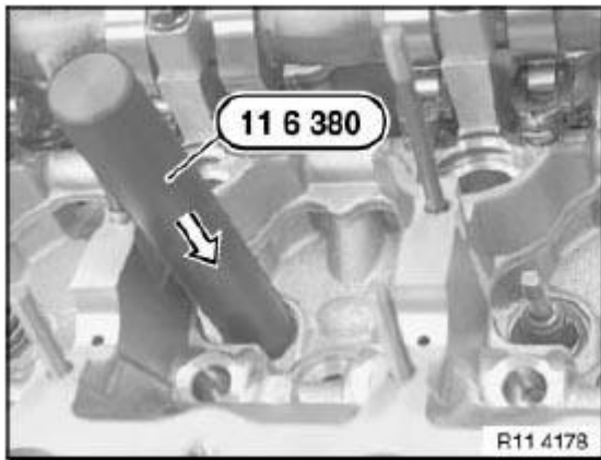
Fig. 300: Pressing Valve Stem Seal Using Special Tool (11 6 380) Courtesy of BMW OF NORTH AMERICA, INC.
