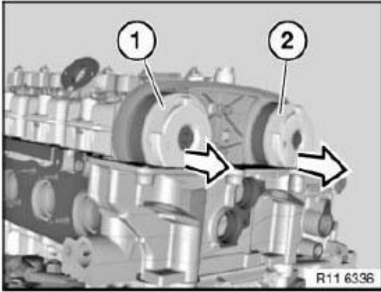
Fig. 304: Removing Exhaust Adjustment Unit From Exhaust Camshaft Courtesy of BMW OF NORTH AMERICA, INC.
