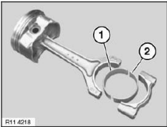
Fig. 203: Identifying Connecting Rod Bearing Shells Courtesy of BMW OF NORTH AMERICA, INC.
