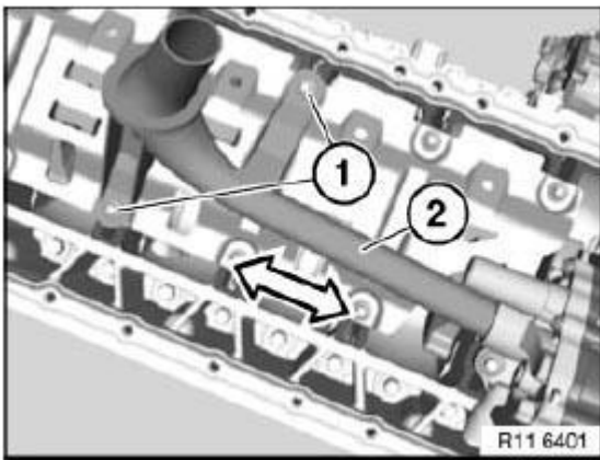
Fig. 392: Removing Oil Pump Intake Pipe Courtesy of BMW OF NORTH AMERICA, INC.
