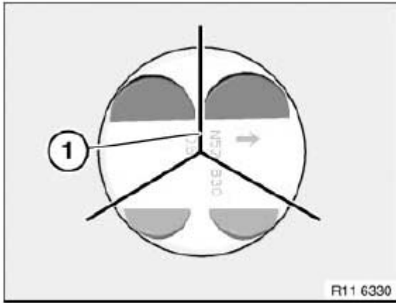
Fig. 230: Identifying Contact Points Of Piston Rings Courtesy of BMW OF NORTH AMERICA, INC.
