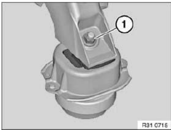
Fig. 40: Identifying Engine Mounting Nut Courtesy of BMW OF NORTH AMERICA, INC.
