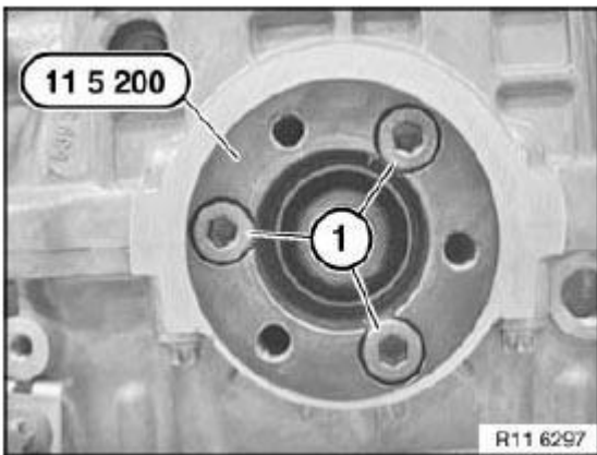
Fig. 286: Tightening Special Tool (11 5 200) With Screws Courtesy of BMW OF NORTH AMERICA, INC.
