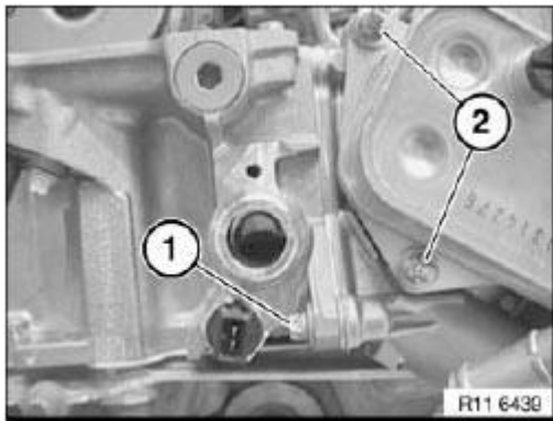
Fig. 397: Identifying Oil Filter Cover Screws Courtesy of BMW OF NORTH AMERICA, INC.
