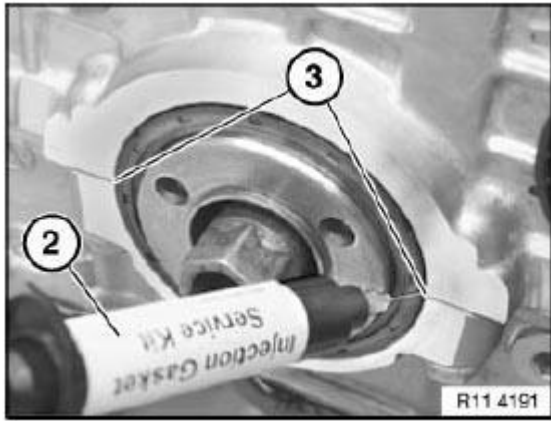
Fig. 119: Filling Grooves With Loctite Sealing Compound Using Injector Courtesy of BMW OF NORTH AMERICA, INC.
