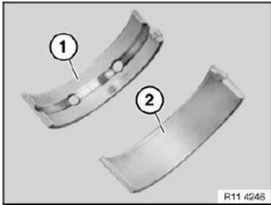
Fig. 130: Identifying Bearing Shell With/Without Lubricant Groove Courtesy of BMW OF NORTH AMERICA, INC.
