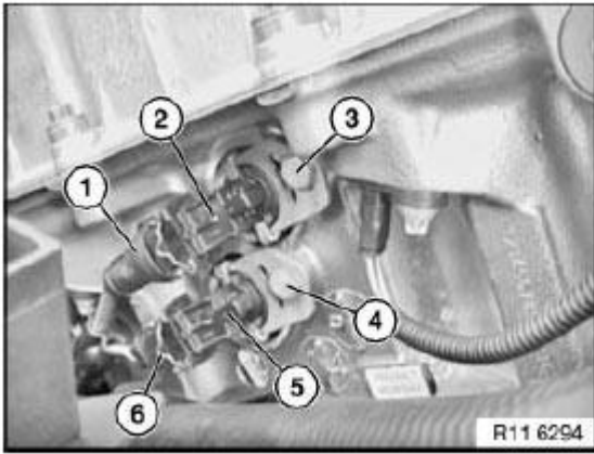
Fig. 301: Identifying Solenoid Valve, Plug Connection And Screws Courtesy of BMW OF NORTH AMERICA, INC.
