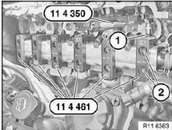
Fig. 268: Mounting Special Tool (11 4 461) On Cylinder Head Screw Courtesy of BMW OF NORTH AMERICA, INC.
