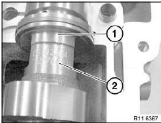
Fig. 251: Identifying Exhaust Camshafts With Part Number
