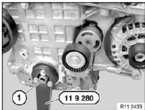
Fig. 277: Releasing Central Bolt Courtesy of BMW OF NORTH AMERICA, INC.
