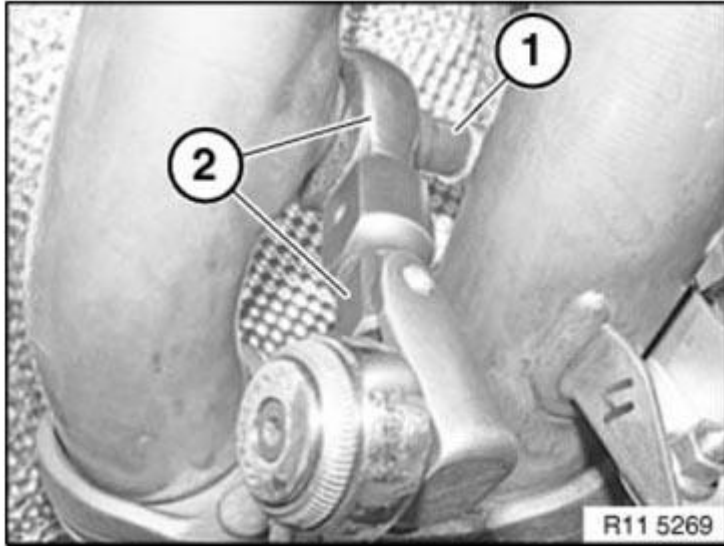
Fig. 414: Identifying Lambda Monitoring Sensor Courtesy of BMW OF NORTH AMERICA, INC.
