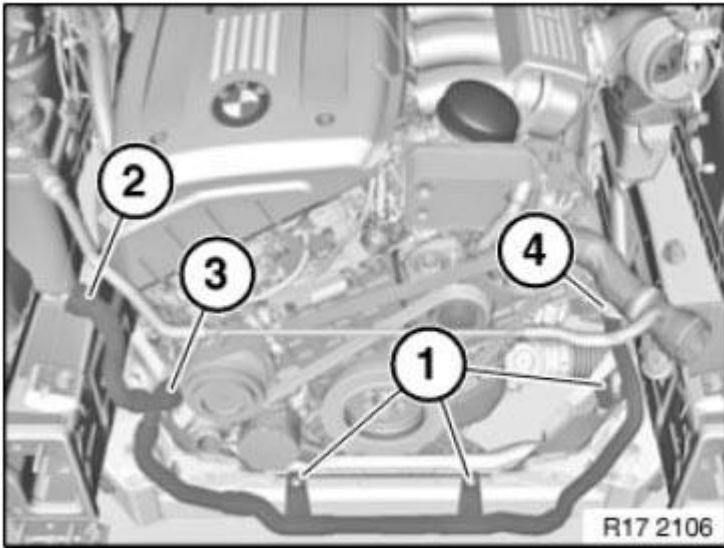
Fig. 400: Identifying Screws On Front Axle Support Courtesy of BMW OF NORTH AMERICA, INC.
