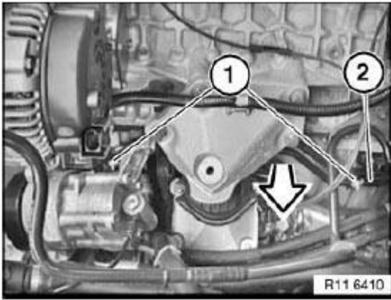
Fig. 26: Removing Lines With Oil-Water Heat Exchanger Courtesy of BMW OF NORTH AMERICA, INC.
