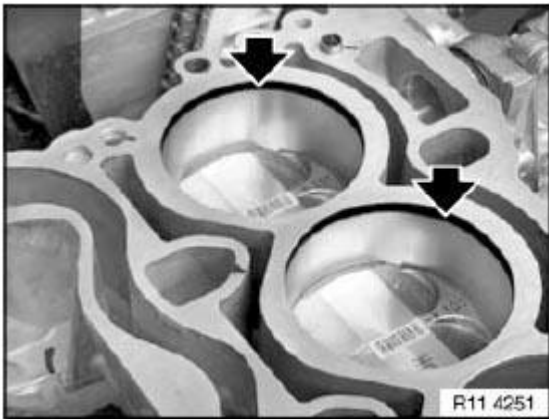
Fig. 207: Locating Oil Carbon Residue On Cylinder Wall
