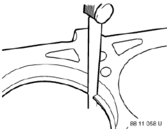
Fig. 227: Measuring End Clearance Using Feeler Gauge Courtesy of BMW OF NORTH AMERICA, INC.
