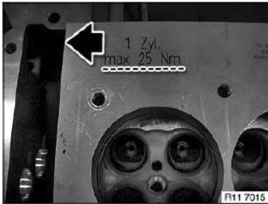
Fig. 41: Securing Special Tool (11 4 341) With Bolts Courtesy of BMW OF NORTH AMERICA, INC.
