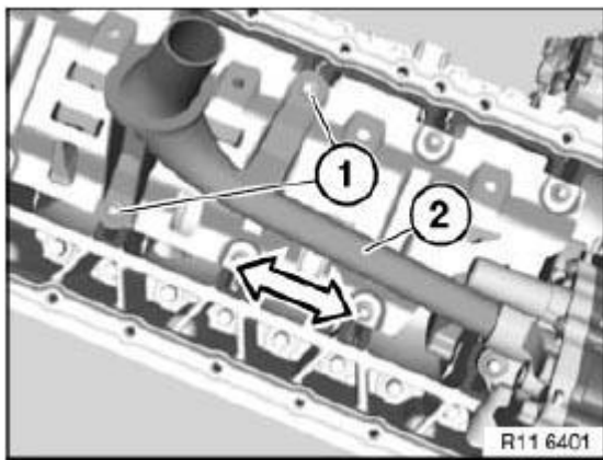
Fig. 153: Pulling Oil Pump Intake Pipe Courtesy of BMW OF NORTH AMERICA, INC.
