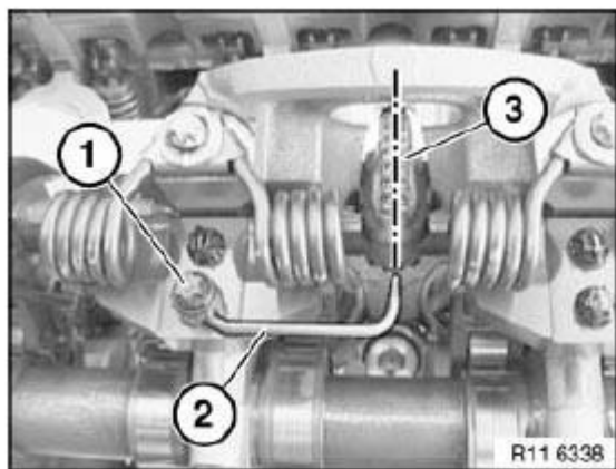
Fig. 339: Identifying Oil Spray Nozzle With Spray
