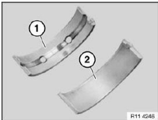
Fig. 133: Identifying Bearing Shell With/Without Lubricant Groove Courtesy of BMW OF NORTH AMERICA, INC.
