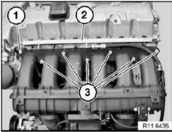
Fig. 406: Identifying Fuel Rail, Screw And Nuts Courtesy of BMW OF NORTH AMERICA, INC.
