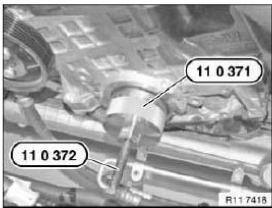
Fig. 110: Inserting Special Tools (11 0 371) Into Crankshaft Seal Courtesy of BMW OF NORTH AMERICA, INC.
