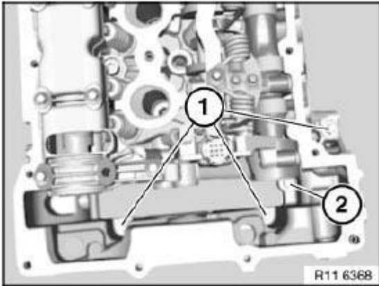
Fig. 50: Identifying Timing Chain Module Screws And Bolts Courtesy of BMW OF NORTH AMERICA, INC.
