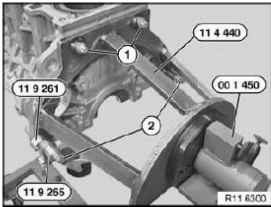
Fig. 22: Identifying Engine Block With Steel And Aluminum Bolts Courtesy of BMW OF NORTH AMERICA, INC.
