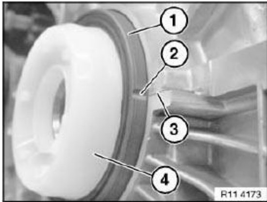
Fig. 78: Identifying Radial Seal, Groove Housing Partition And Bush Courtesy of BMW OF NORTH AMERICA, INC.
