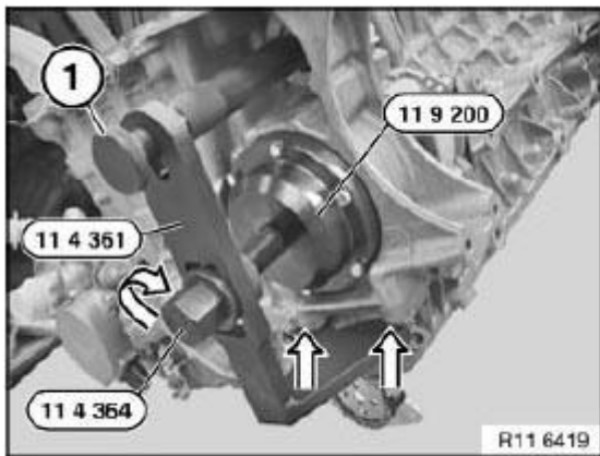
Fig. 124: Attaching Special Tool (11 4 361) To Bedplate Construction Screw Connection Courtesy of BMW OF NORTH AMERICA, INC.
