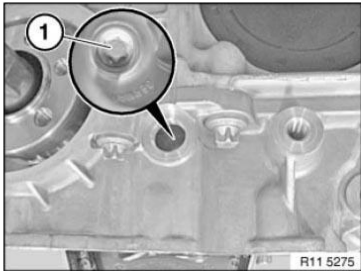
Fig. 158: Identifying Oil Pump Screw Courtesy of BMW OF NORTH AMERICA, INC.
