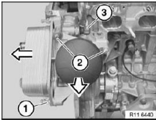
Fig. 398: Releasing Screw
