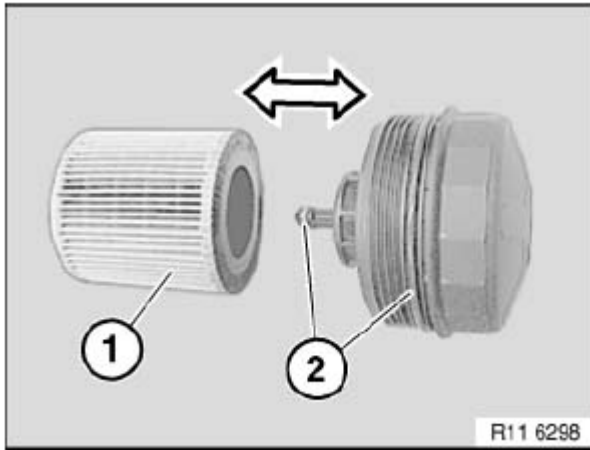
Fig. 20: Removing Oil Filter Element
