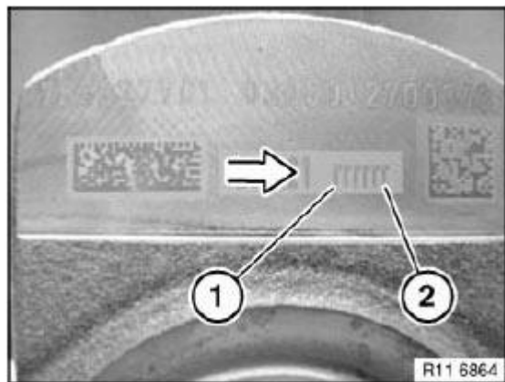
Fig. 201: Identifying Crankpin Marking Courtesy of BMW OF NORTH AMERICA, INC.
