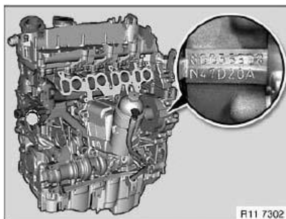
Fig. 4: Identifying Engine Identification Mark - N47/N47S/N47C/N57 N57S Courtesy of BMW OF NORTH AMERICA, INC.
