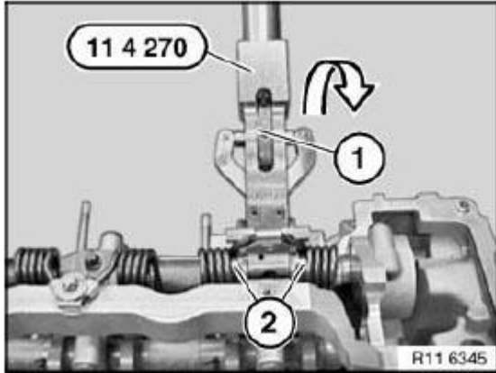
Fig. 320: Pressing Special Tool (11 4 270) Courtesy of BMW OF NORTH AMERICA, INC.
