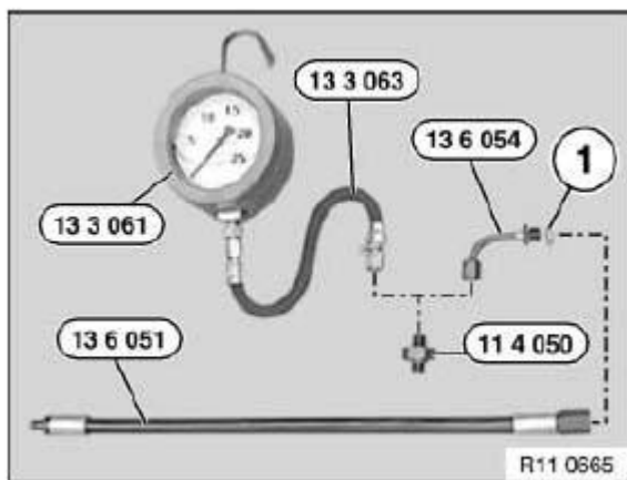
Fig. 368: Checking Engine Oil Pressure Using Pressure Gauge Courtesy of BMW OF NORTH AMERICA, INC.
