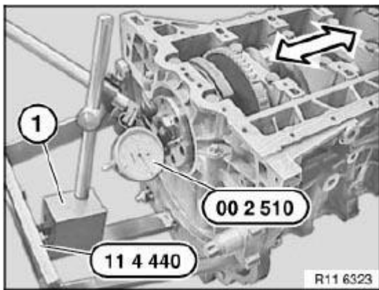
Fig. 146: Moving Crankshaft Courtesy of BMW OF NORTH AMERICA, INC.
