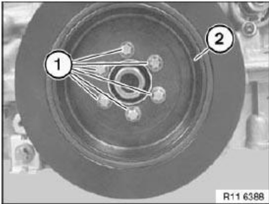
Fig. 200: Identifying Vibration Damper And Screws Courtesy of BMW OF NORTH AMERICA, INC.
