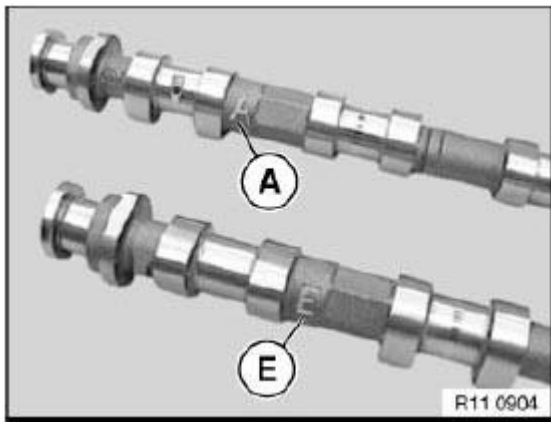
Fig. 273: Identifying Exhaust/Intake Camshafts Marks Courtesy of BMW OF NORTH AMERICA, INC.
