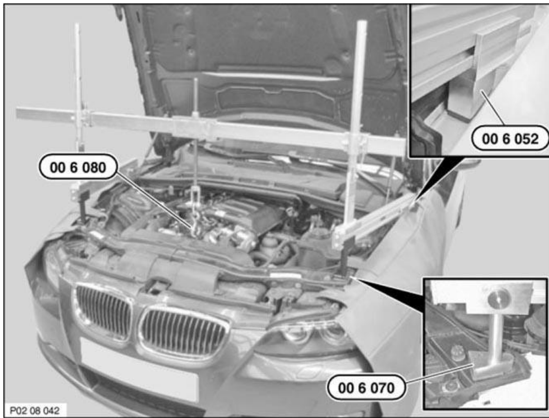
Fig. 38: Identifying Special Tools
