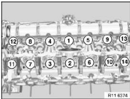
Fig. 58: Cylinder Head Bolts Tightening Sequence Courtesy of BMW OF NORTH AMERICA, INC.
