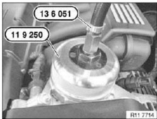
Fig. 376: Securing Special Tool (13 6 051) With Sealing Ring Courtesy of BMW OF NORTH AMERICA, INC.
