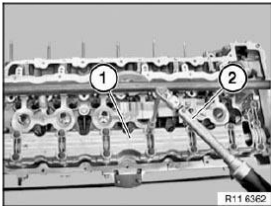
Fig. 256: Removing Bearing Strips Bolt Courtesy of BMW OF NORTH AMERICA, INC.
