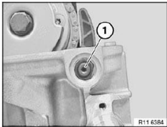
Fig. 280: Identifying Timing Chain Module Bearing Pin (Cylinder Head) Courtesy of BMW OF NORTH AMERICA, INC.
