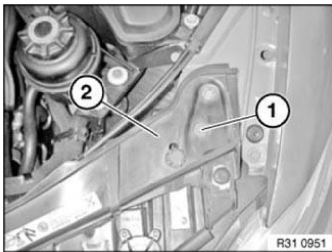
Fig. 37: Identifying Screw On Front Panel
