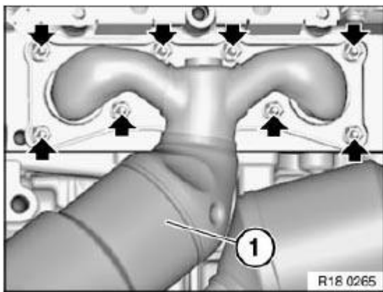
Fig. 409: Locating Exhaust Manifold Nuts Courtesy of BMW OF NORTH AMERICA, INC.
