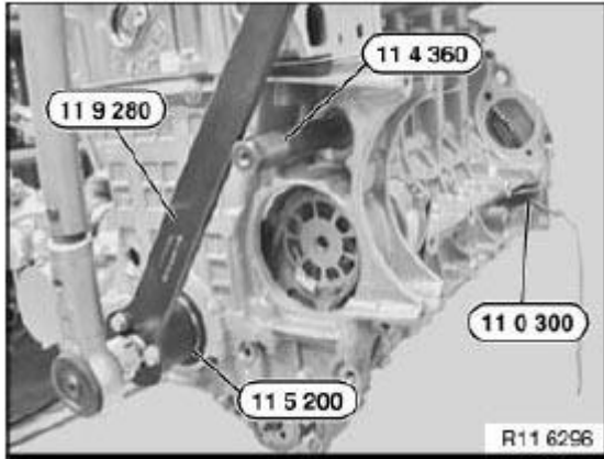
Fig. 289: Tightening Central Bolt Courtesy of BMW OF NORTH AMERICA, INC.
