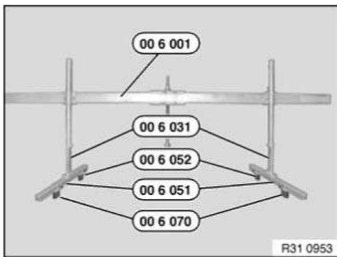
Fig. 33: Identifying Profile Strips, Supports And Connections Courtesy of BMW OF NORTH AMERICA, INC.
