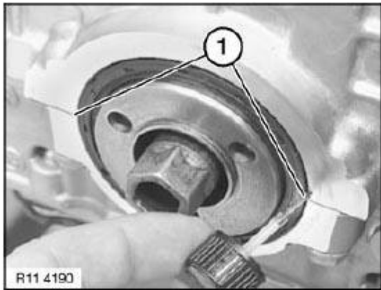
Fig. 120: Coating Sealing Compound Surface Courtesy of BMW OF NORTH AMERICA, INC.
