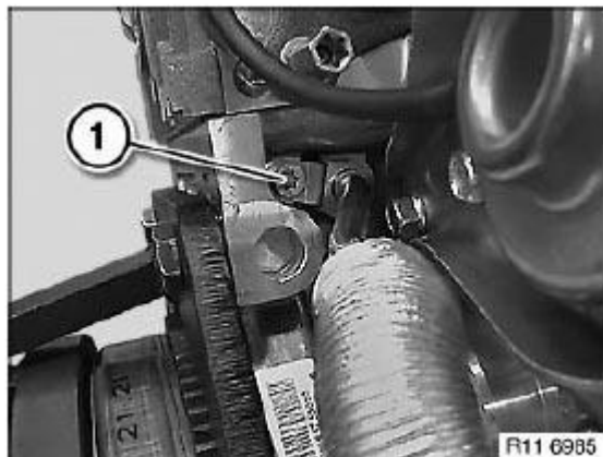
Fig. 281: Identifying Screws
