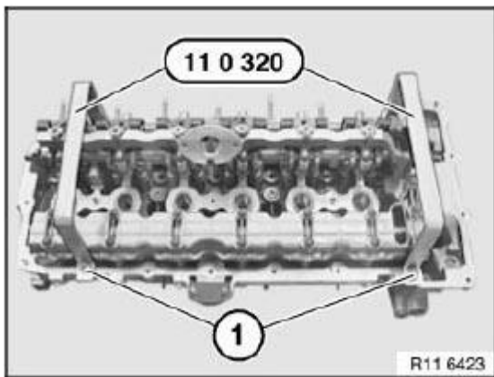
Fig. 44: Identifying Special Tool (11 0 320)
