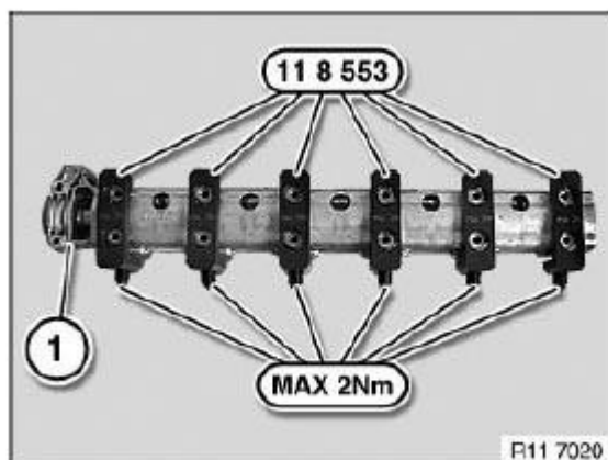
Fig. 191: Identifying Special Tools (11 8 553) With Upper & Lower Bearing Strips Courtesy of BMW OF NORTH AMERICA, INC.
