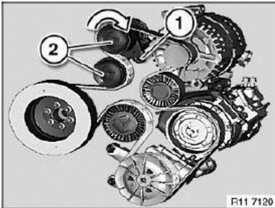
Fig. 138: Identifying Drive Belt Installation Position Courtesy of BMW OF NORTH AMERICA, INC.
