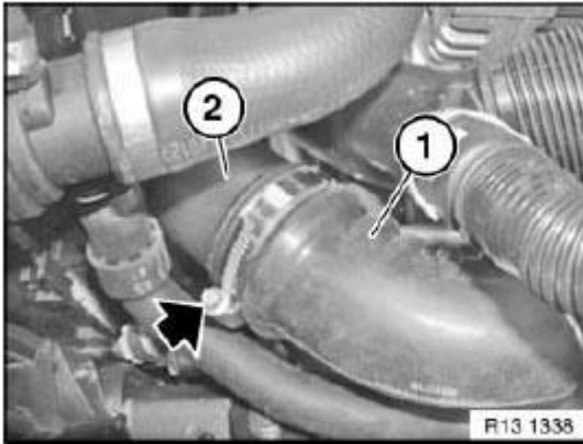
Fig. 369: Identifying Charge-Air Hose And Charge-Air Duct Courtesy of BMW OF NORTH AMERICA, INC.
