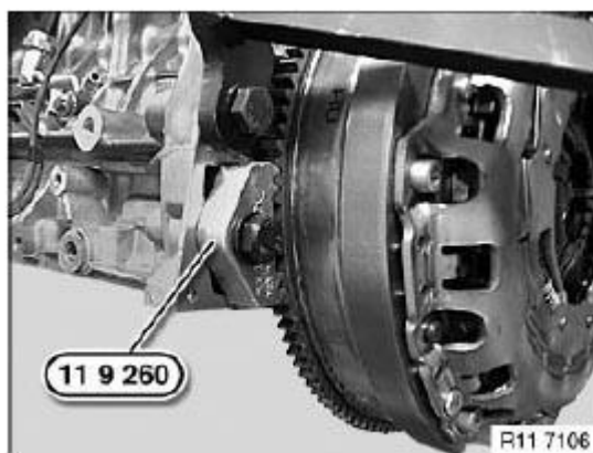
Fig. 265: Securing Flywheel (Crankshaft) With Special Tool (11 9 260) Courtesy of BMW OF NORTH AMERICA, INC.
