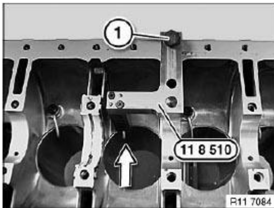
Fig. 165: Attaching Special Tool (11 8 510) To Bolt Connection On Main Bearing Courtesy of BMW OF NORTH AMERICA, INC.
