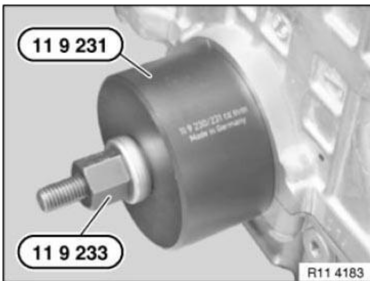
Fig. 158: Identifying Special Tools 119 231 And 11 9 233 Courtesy of BMW OF NORTH AMERICA, INC.
