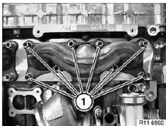
Fig. 396: Identifying Nuts
