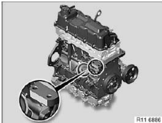
Fig. 31: Identifying Engine Identification Marks - W10 / W11 Courtesy of BMW OF NORTH AMERICA, INC.
