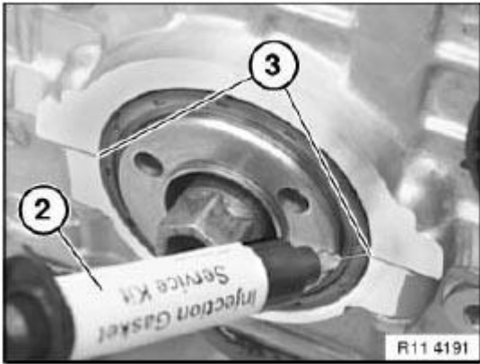
Fig. 77: Filling Both Grooves Flush With Sealant Using Injector/Syringe Courtesy of BMW OF NORTH AMERICA, INC.
