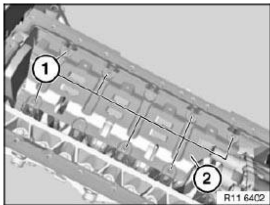
Fig. 106: Identifying Bolts And Screws Courtesy of BMW OF NORTH AMERICA, INC.
