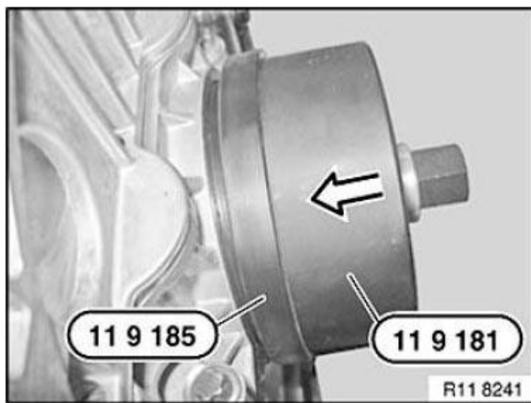
Fig. 104: Installing Rear Crankshaft Seal Using Tool 119 180/181 Courtesy of BMW OF NORTH AMERICA, INC.
