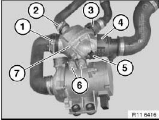
Fig. 349: Identifying Hose Clamp, Coolant Hose, Plug Connection And Screw Courtesy of BMW OF NORTH AMERICA, INC.
