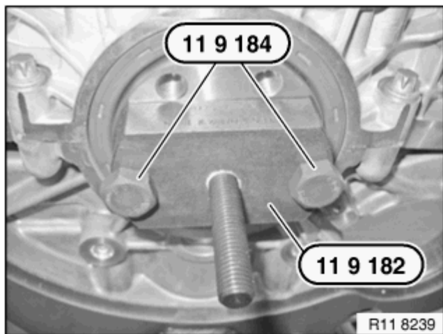
Fig. 102: Fastening Special Tool 11 9 182 With Special Tool 11 9 184 On Crankshaft Courtesy of BMW OF NORTH AMERICA, INC.
