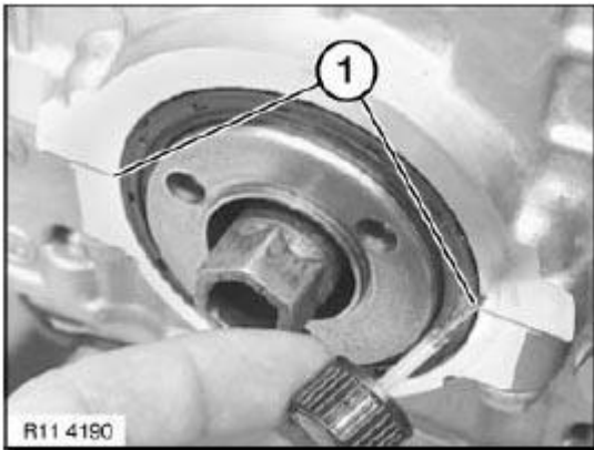
Fig. 78: Coating Surface Of Sealing Compound In Both Grooves With Loctite Primer Courtesy of BMW OF NORTH AMERICA, INC.
