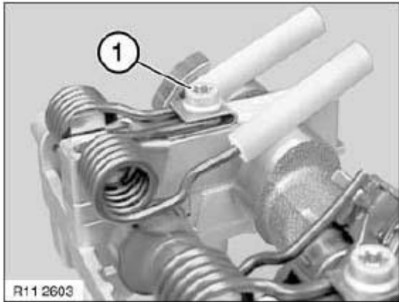
Fig. 253: Identifying Screw
