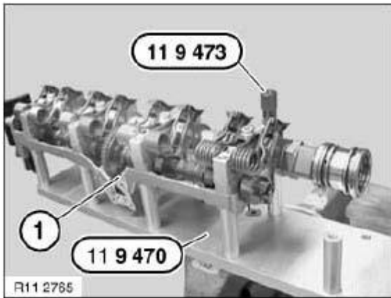
Fig. 283: Identifying Special Tools (11 9 473) And (11 9 470) Courtesy of BMW OF NORTH AMERICA, INC.
