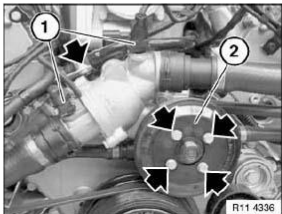
Fig. 587: Identifying Plug Connections And Belt Pulley Screws Courtesy of BMW OF NORTH AMERICA, INC.
