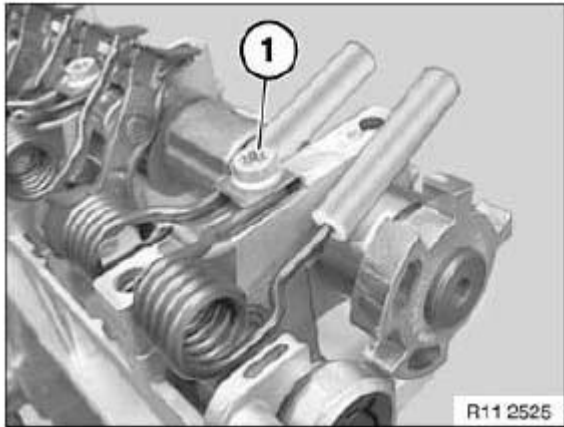
Fig. 205: Identifying Screw
