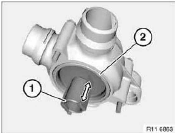
Fig. 457: Removing Thermostat Courtesy of BMW OF NORTH AMERICA, INC.
