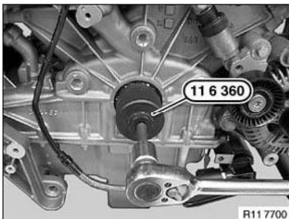
Fig. 84: Screwing Special Tool (11 6 360) Into Radial Seal Courtesy of BMW OF NORTH AMERICA, INC.
