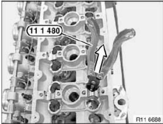
Fig. 270: Removing Valve Stem Seal With Special Tool 11 1 480 Courtesy of BMW OF NORTH AMERICA, INC.
