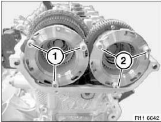
Fig. 340: Identifying Hexagon Socket Screws With Washers Courtesy of BMW OF NORTH AMERICA, INC.
