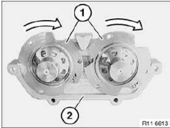
Fig. 302: Checking Thrust Bearing Plates Courtesy of BMW OF NORTH AMERICA, INC.
