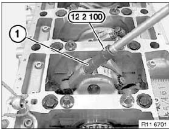
Fig. 168: Identifying Connecting Rod Bolts And Special Tools 12 2 100
