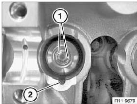
Fig. 288: Identifying Valve Keys Courtesy of BMW OF NORTH AMERICA, INC.
