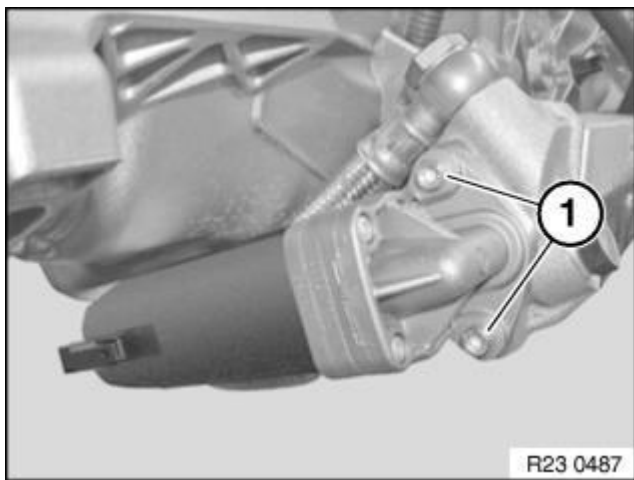
Fig. 439: Release Bolts (1)
