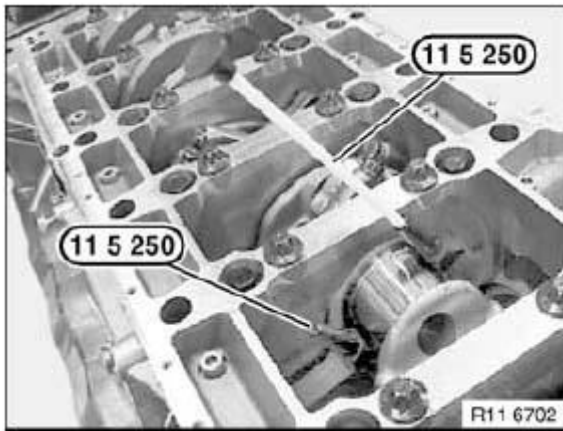
Fig. 167: Identifying Special Tool 11 5 250
