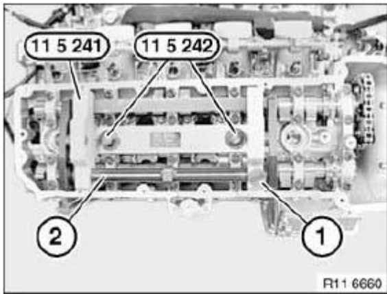
Fig. 190: Identifying Special Tool 11 5 241 And Eccentric Shaft Courtesy of BMW OF NORTH AMERICA, INC.
