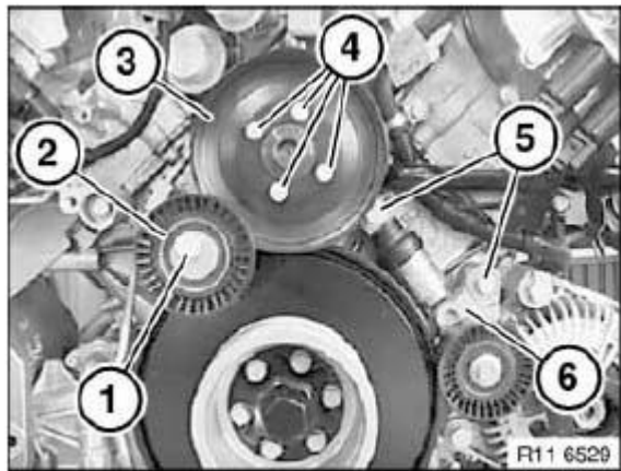
Fig. 134: Identifying Idler Pulley, Belt Pulley And Belt Tensioner Courtesy of BMW OF NORTH AMERICA, INC.
