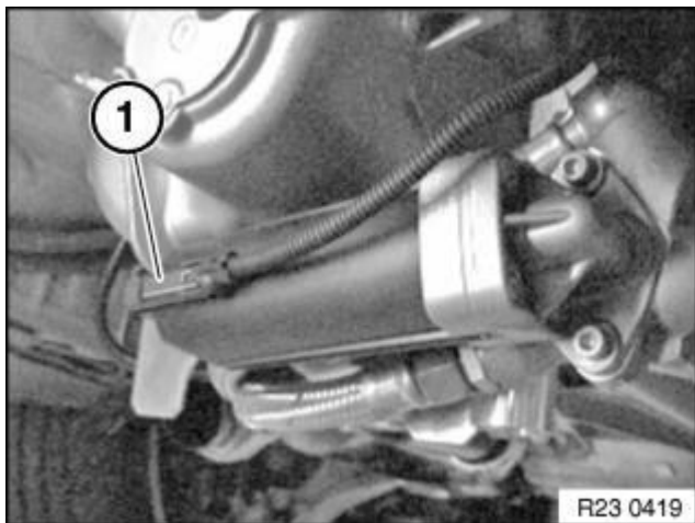
Fig. 438: Disconnect Connector (1)
