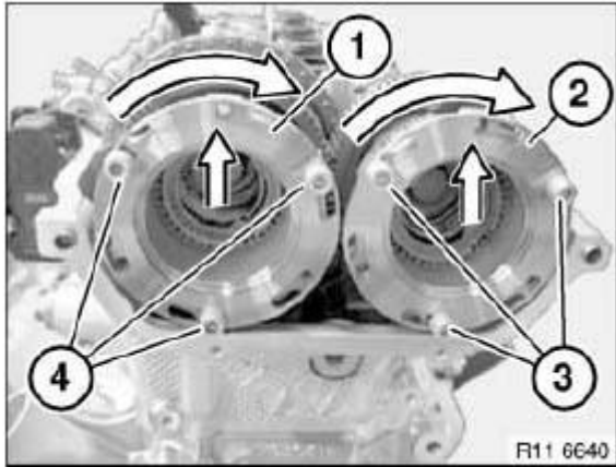
Fig. 242: Pulling VANOS Gear With Outer Sleeve Forwards (2 Of 2) Courtesy of BMW OF NORTH AMERICA, INC.
