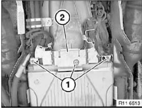
Fig. 71: Identifying Oxygen Sensor Holder Courtesy of BMW OF NORTH AMERICA, INC.
