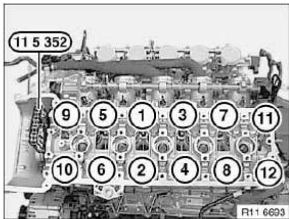
Fig. 54: Identifying Cylinder Head Bolts Removal Sequence Courtesy of BMW OF NORTH AMERICA, INC.
