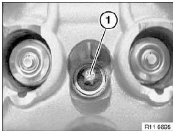
Fig. 53: Identifying Cylinder Head Bolt Courtesy of BMW OF NORTH AMERICA, INC.
