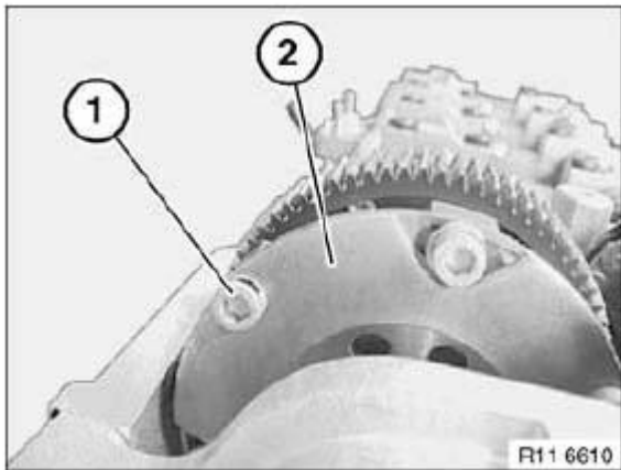
Fig. 393: Identifying Hexagon Socket Screws Courtesy of BMW OF NORTH AMERICA, INC.
