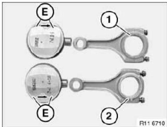
Fig. 155: Identifying Connecting Rod Elevation - Cylinders 6-10 And 1-5 (1 Of 2) Courtesy of BMW OF NORTH AMERICA, INC.
