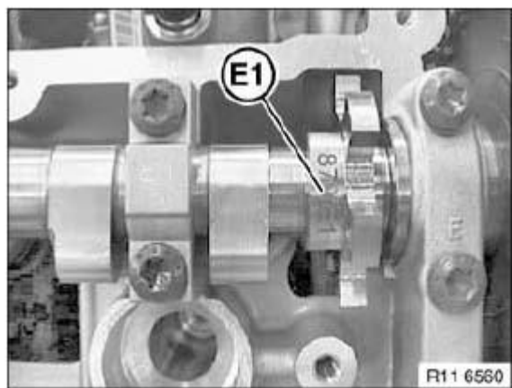
Fig. 233: Identifying Designation (E1) On Dihedron Points Upwards Courtesy of BMW OF NORTH AMERICA, INC.
