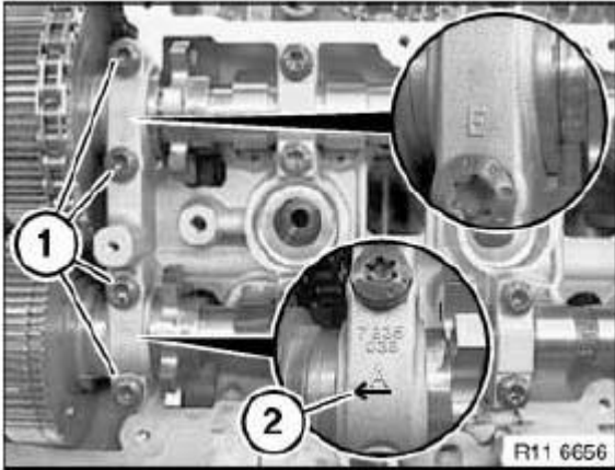
Fig. 200: Identifying Screws
