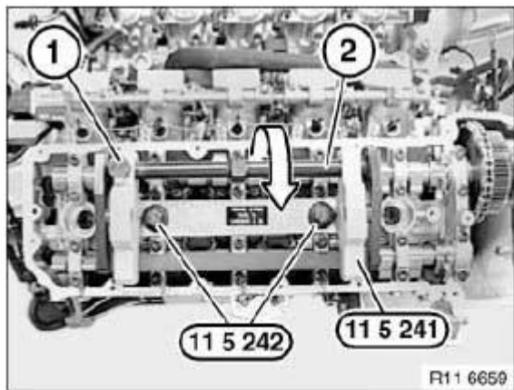
Fig. 211: Relieving Tension On Eccentric Shaft At Hexagon Head (1 Of 2) Courtesy of BMW OF NORTH AMERICA, INC.
