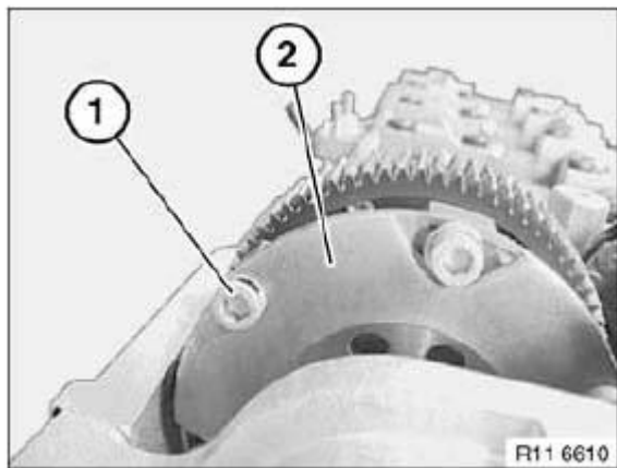
Fig. 367: Identifying Hexagon Socket Screws Courtesy of BMW OF NORTH AMERICA, INC.
