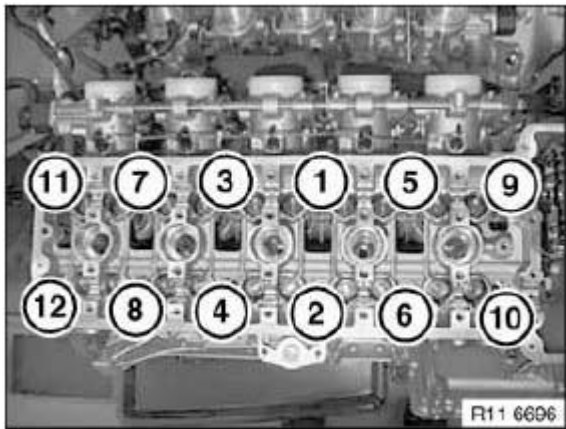
Fig. 62: Identifying Cylinder Head Bolts Removal Sequence Courtesy of BMW OF NORTH AMERICA, INC.
