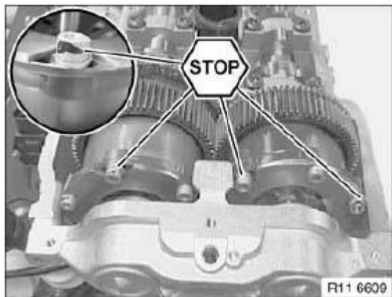
Fig. 296: Identifying Hexagon Socket Screws Courtesy of BMW OF NORTH AMERICA, INC.
