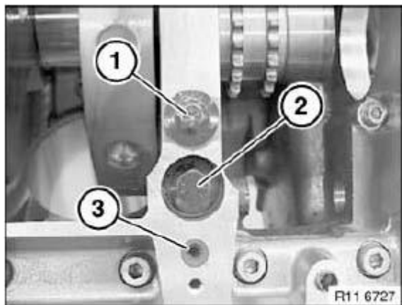
Fig. 96: Identifying Bearing Block Bolts And Fine-Mesh Strainer Courtesy of BMW OF NORTH AMERICA, INC.
