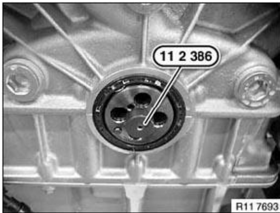
Fig. 83: Identifying Special Tool (11 2 386) On Crankshaft Courtesy of BMW OF NORTH AMERICA, INC.
