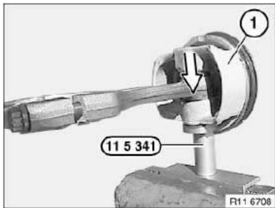
Fig. 149: Securing Piston With Conrod To Special Tool 11 5 341 Courtesy of BMW OF NORTH AMERICA, INC.
