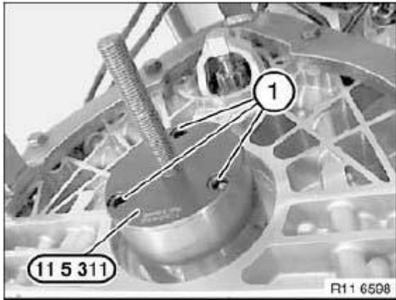
Fig. 92: Identifying Special Tool 11 5 311 Courtesy of BMW OF NORTH AMERICA, INC.
