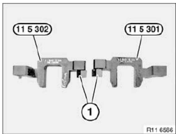
Fig. 237: Identifying Spacers, Special Tools E 11 5 301 And A 11 5 302 Courtesy of BMW OF NORTH AMERICA, INC.
