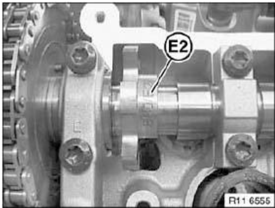
Fig. 234: Identifying Designation (E2) On Dihedron Points Upwards Courtesy of BMW OF NORTH AMERICA, INC.
