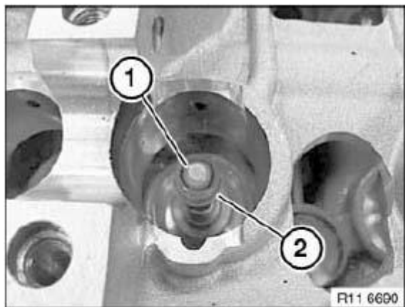
Fig. 272: Identifying Valve Stem Seal And Mounting Sleeve Courtesy of BMW OF NORTH AMERICA, INC.
