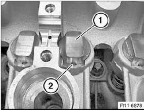
Fig. 253: Identifying HVCA Elements And Lock Courtesy of BMW OF NORTH AMERICA, INC.
