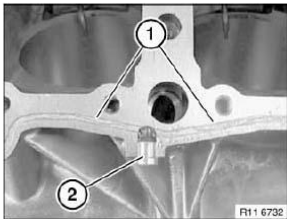
Fig. 100: Identifying Nozzles
