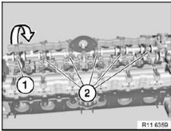
Fig. 267: Bearing Caps
