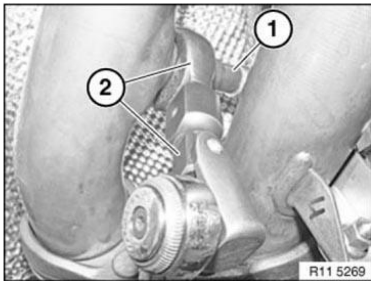
Fig. 336: Removing Lambda Monitoring Sensor Plug Connection Using Special Tool (11 9 150) Courtesy of BMW OF NORTH AMERICA, INC.
