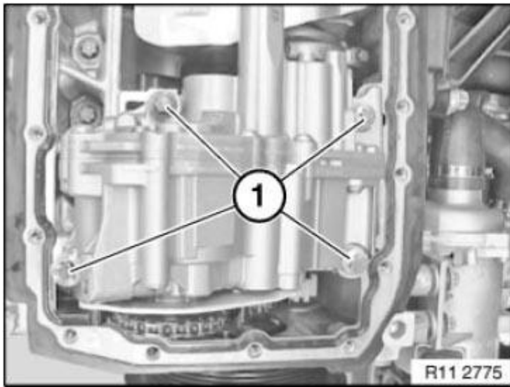
Fig. 112: Identifying Screws
