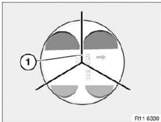
Fig. 193: Contact Points Of Piston Rings Courtesy of BMW OF NORTH AMERICA, INC.
