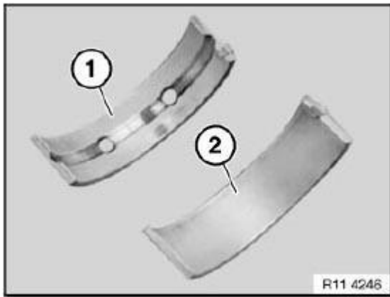
Fig. 152: Bearing Shells
