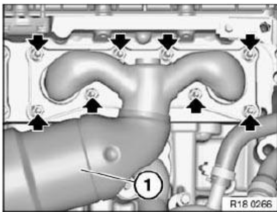
Fig. 324: Locating Exhaust Manifold Nuts Courtesy of BMW OF NORTH AMERICA, INC.
