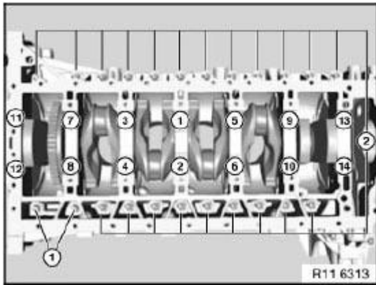
Fig. 100: Crankshaft Bolts Tightening Sequence Courtesy of BMW OF NORTH AMERICA, INC.
