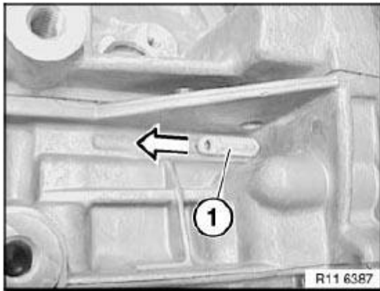
Fig. 229: Fastener
