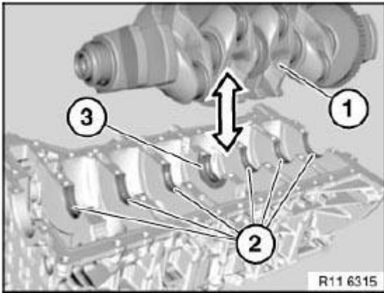
Fig. 155: Bearing Shells
