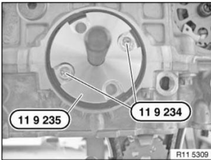
Fig. 141: Mounting Special Tool 11 9 235 With Special Tool 11 9 234 On Crankshaft Courtesy of BMW OF NORTH AMERICA, INC.
