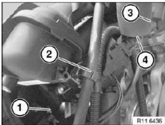
Fig. 319: Crankcase Breathers, Plug Connection And Holder Courtesy of BMW OF NORTH AMERICA, INC.
