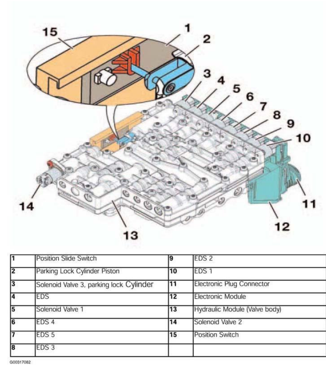
Fig. 23: Identifying Valve Body Components (6HP26Z) Courtesy of BMW OF NORTH AMERICA, INC.
