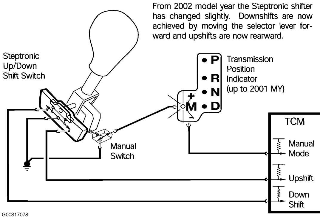
Fig. 19: Identifying Steptronic Components
